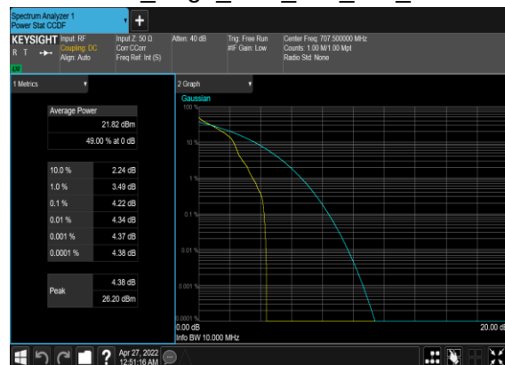
N12(10M)_DFT-s-OFDM_PI_2- BPSK_Edge_1RB_Left_Mid_CH
