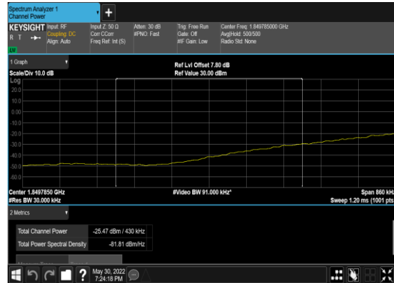
N2(40M)_DFT-s- OFDM_BPSK_Edge_1RB_Left_Low_CH_chp_PASS
