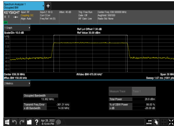
N26(15M)_DFT-s- OFDM_QPSK_Outer_Full_Mid_CH
