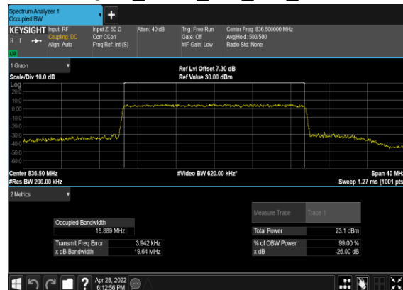
N26(20M)_CP-OFDM_256 QAM_Outer_Full_Mid_CH
