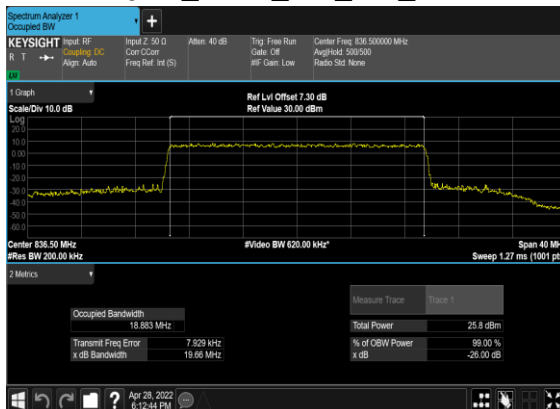
N26(20M)_CP-OFDM_64 QAM_Outer_Full_Mid_CH
