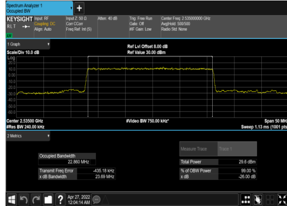
N7(25M)_DFT-s- OFDM_QPSK_Outer_Full_Mid_CH
