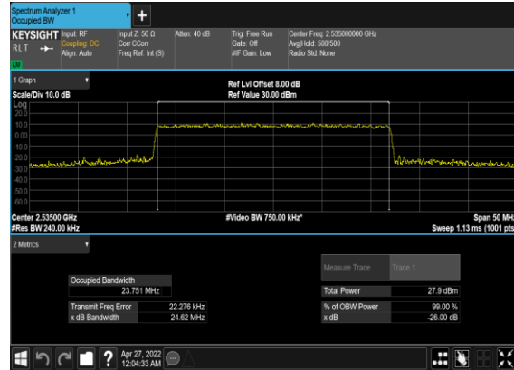
N7(25M)_CP-OFDM_16 QAM_Outer_Full_Mid_CH
