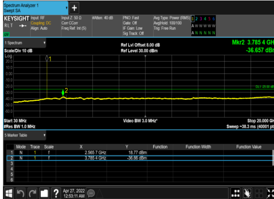
N7(5M)_DFT-s- OFDM_BPSK_Edge_1RB_Left_High_CH
