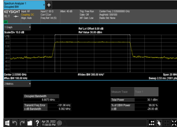
N7(10M)_DFT-s- OFDM_QPSK_Outer_Full_Mid_CH
