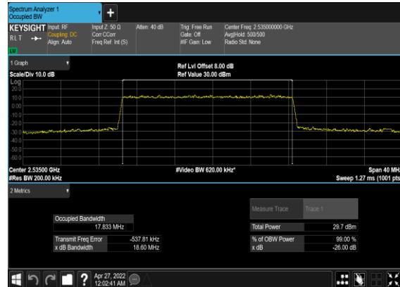
N7(20M)_DFT-s- OFDM_QPSK_Outer_Full_Mid_CH
