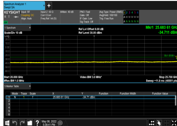
N7(50M)_DFT-s- OFDM_BPSK_Edge_1RB_Left_Mid_CH
