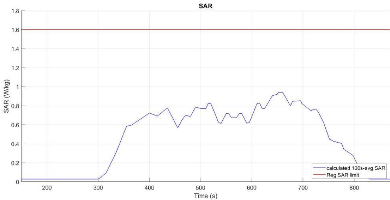
Figure 6- 21 Time-averaged SAR
