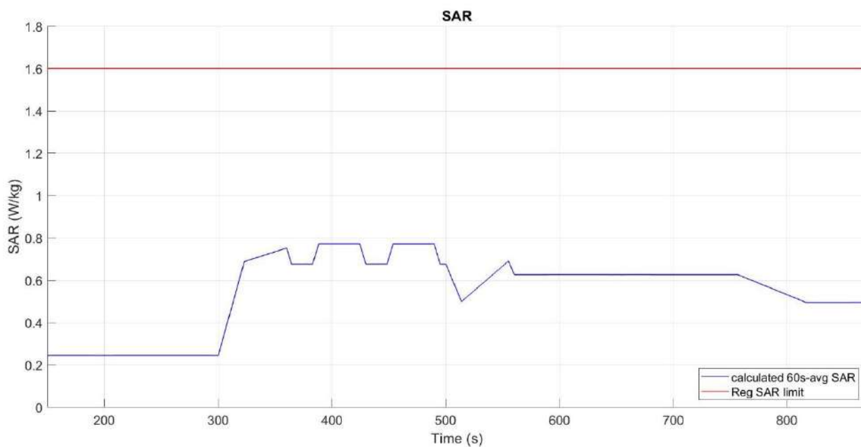
Figure 6- 23 Time-averaged SAR
