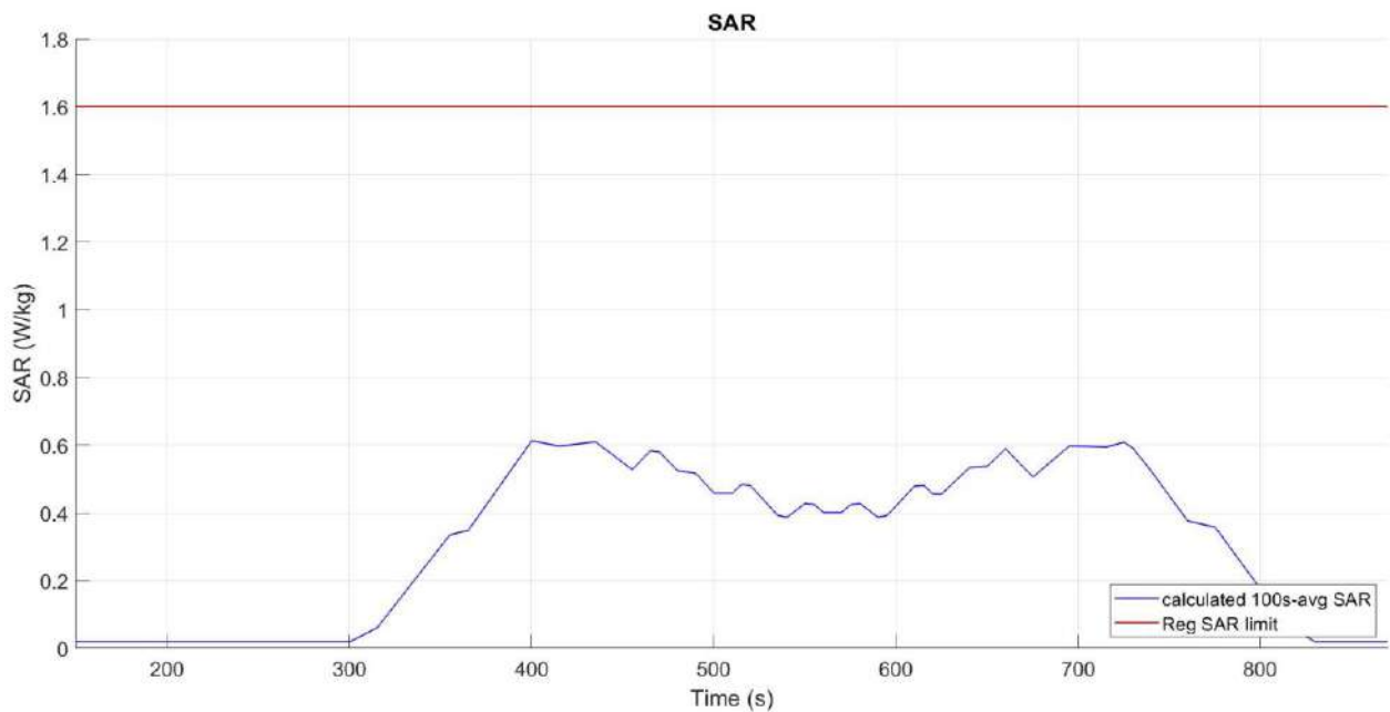
Figure 6- 28 Time-averaged SAR
