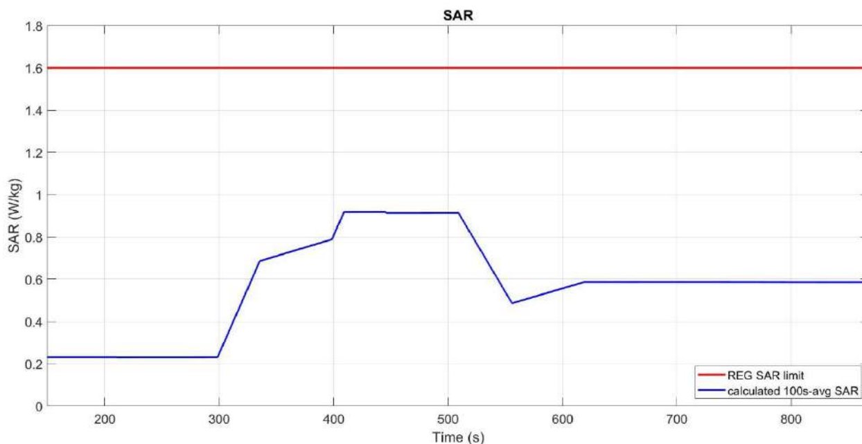
Figure 7-11 Time-averaged SAR
