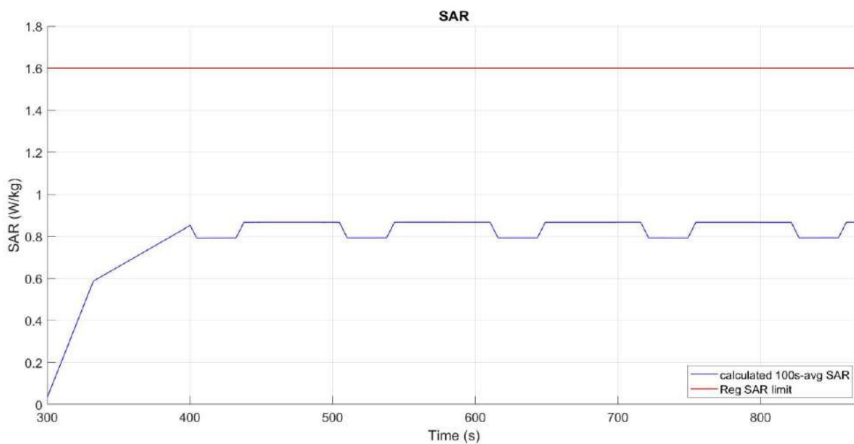
Figure 6- 6 Time-averaged SAR
