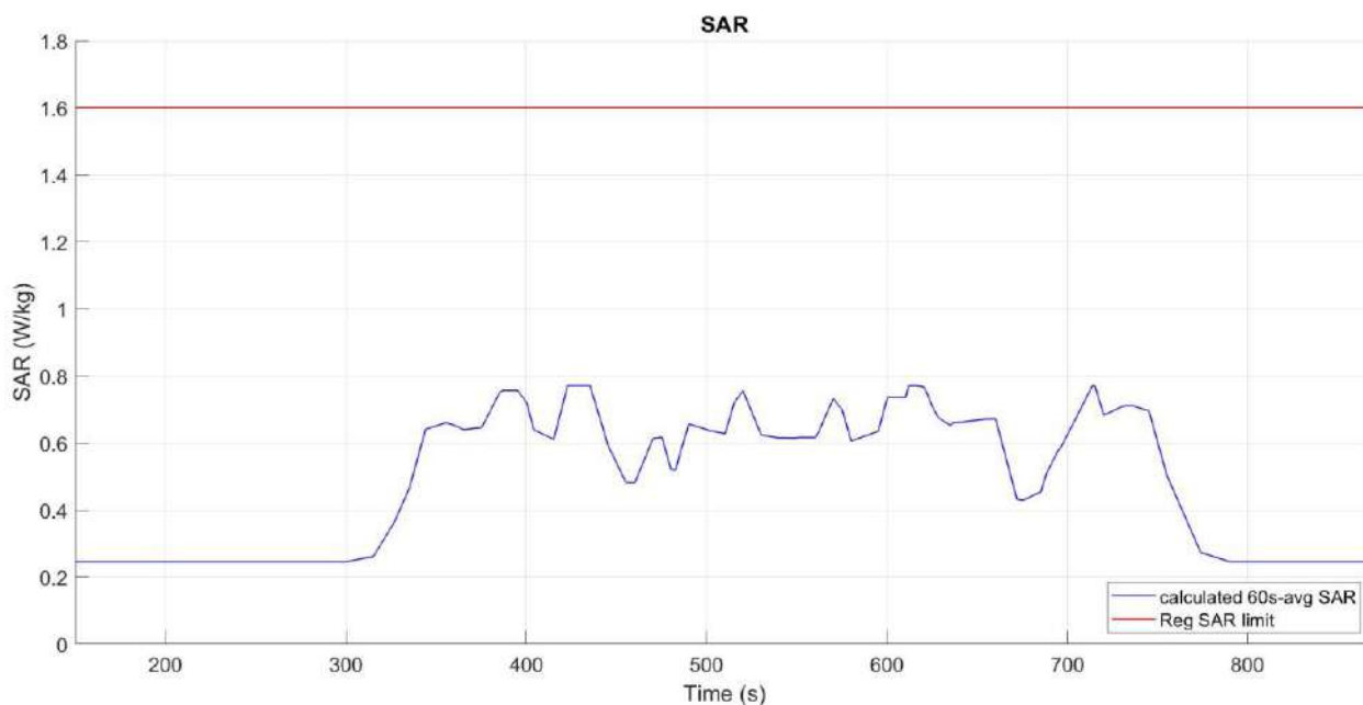
Figure 6- 24 Time-averaged SAR
