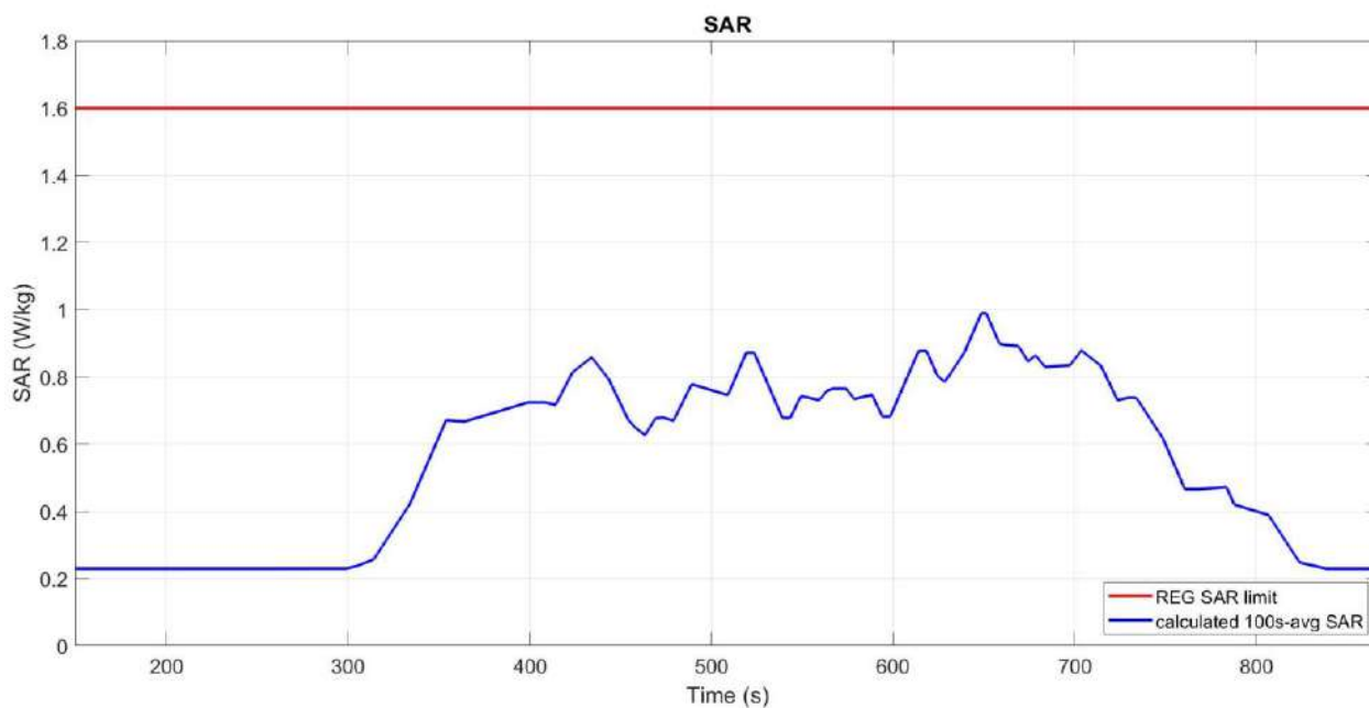
Figure 7-12 Time-averaged SAR
