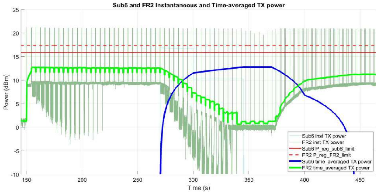
Figure 8-14 LTE, mmW inst. Pwr and Time-averaged Tx Pwr
