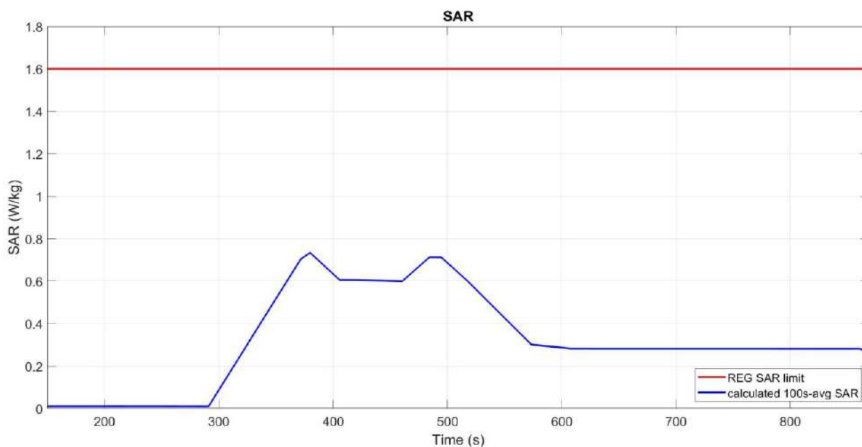
Figure 7-5 Time-averaged SAR
