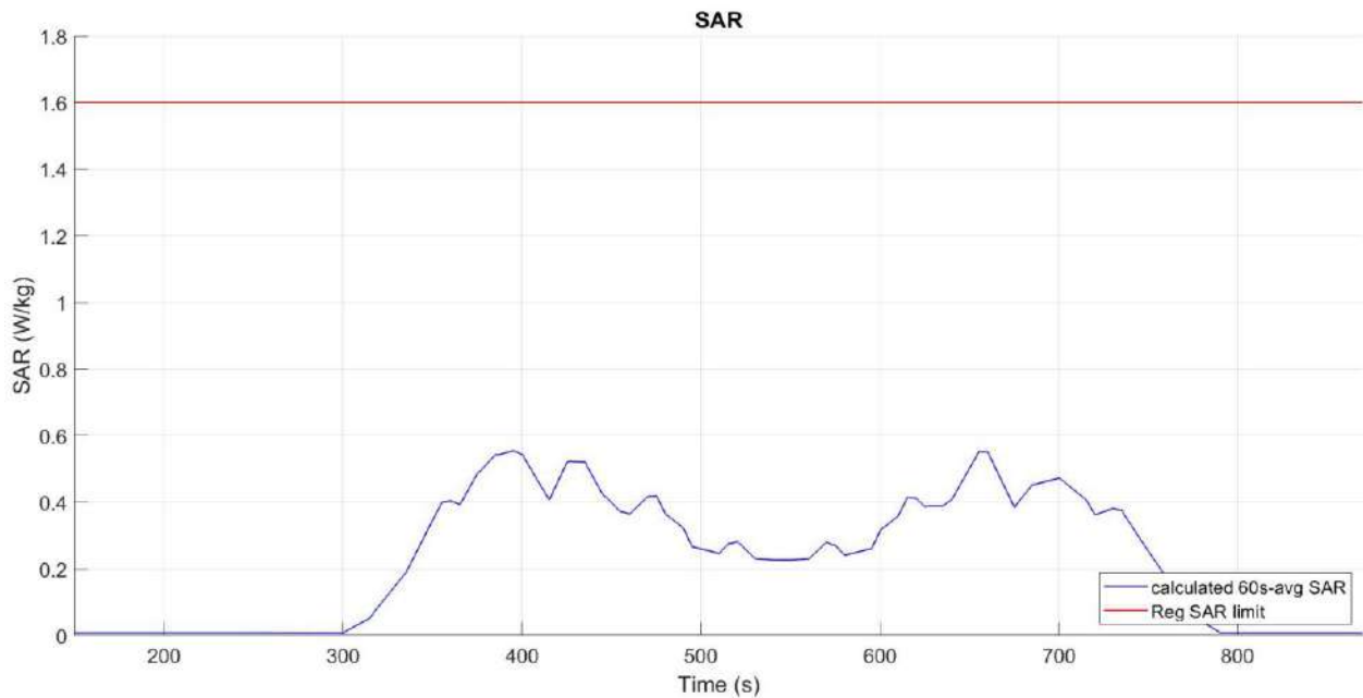
Figure 6- 36 Time-averaged SAR
