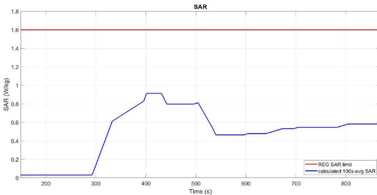
Figure 7-13 Time-averaged SAR
