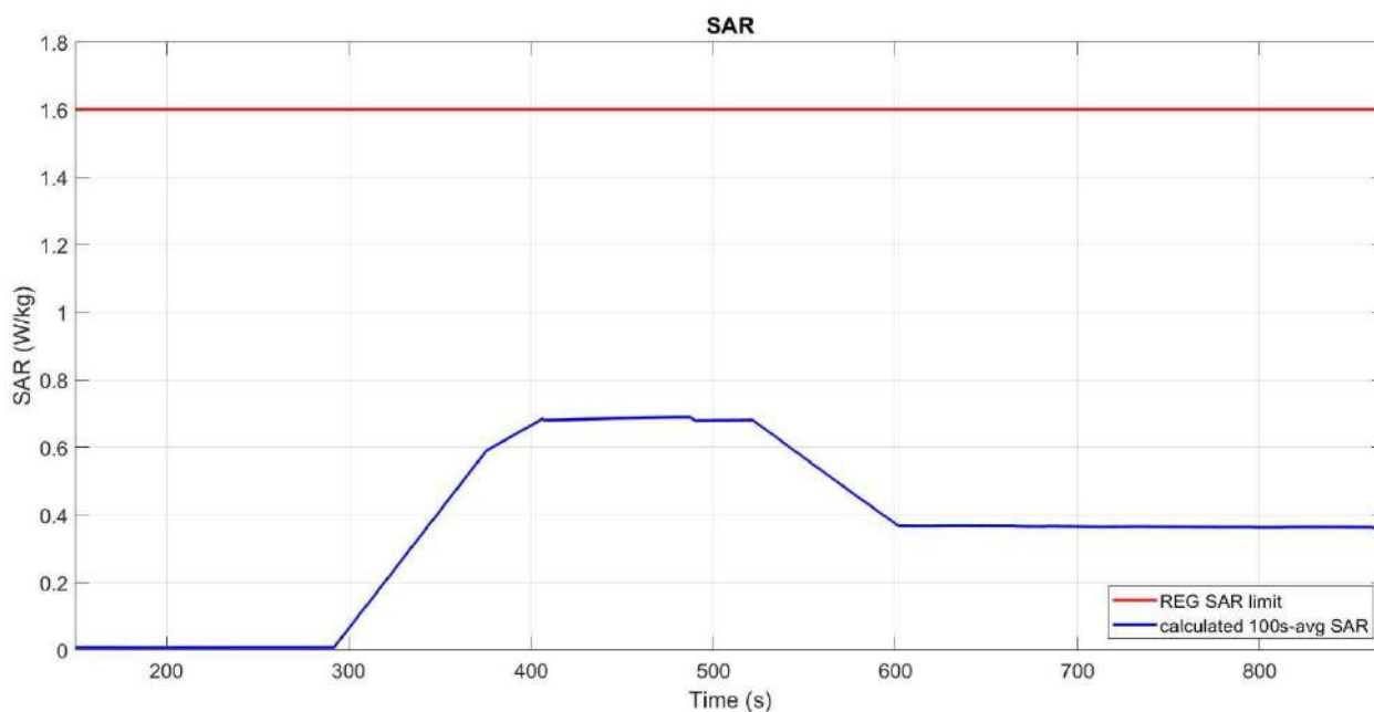
Figure 7-9 Time-averaged SAR
