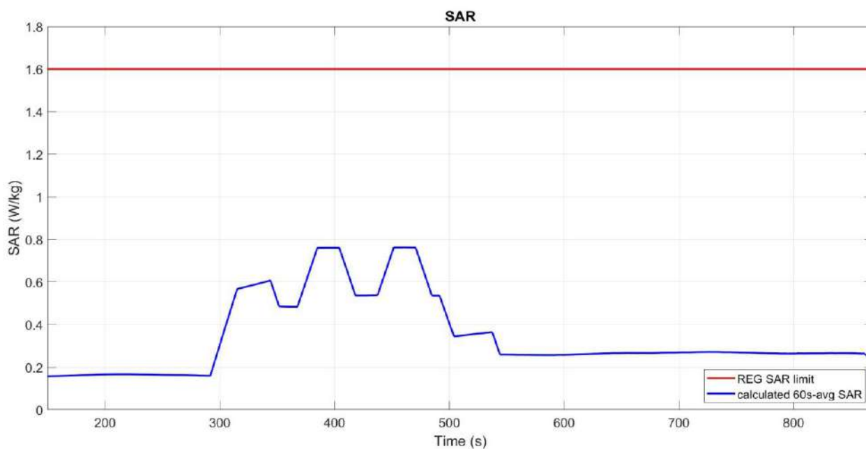
Figure 7-3 Time-averaged SAR
