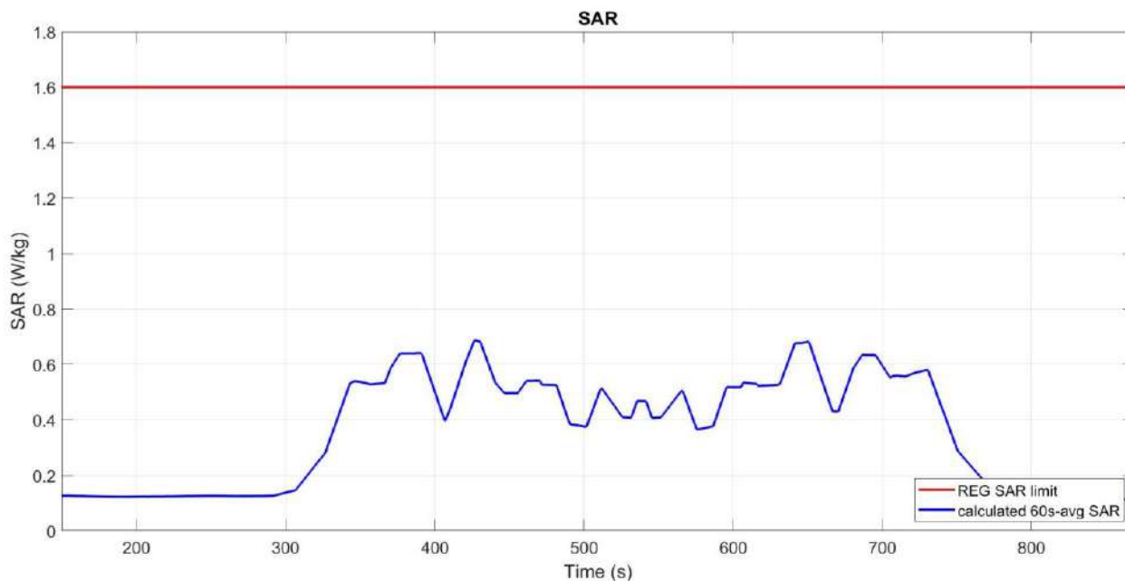
Figure 7-4 Time-averaged SAR
