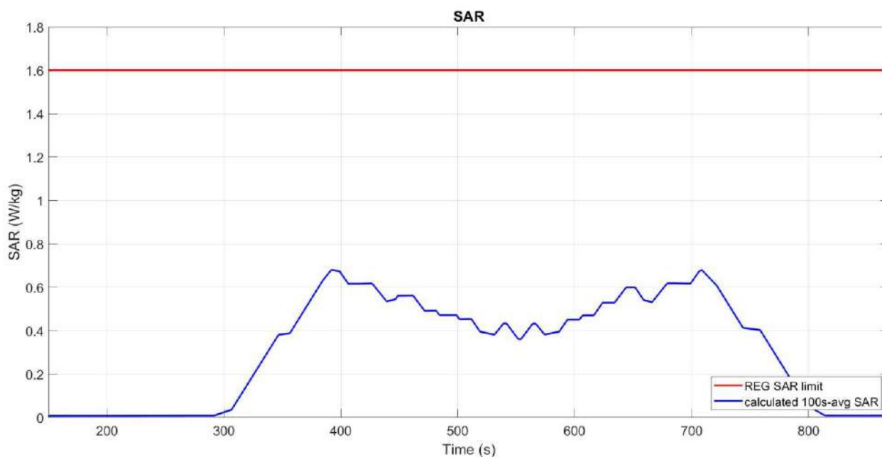
Figure 7-10 Time-averaged SAR
