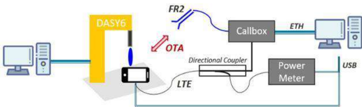
Figure 9-1 TA-PD near-field measurement setup diagram
