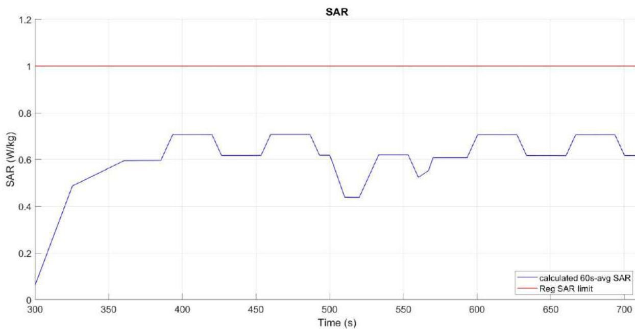
Figure 6- 37 Time-averaged SAR
