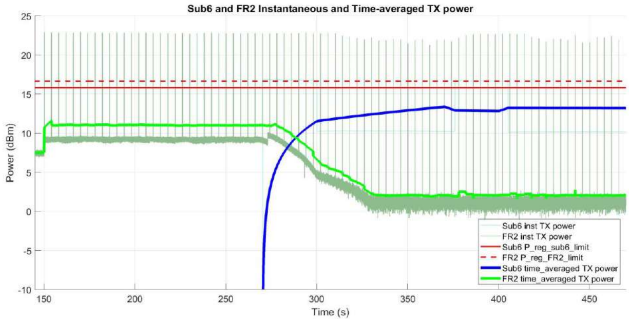
Figure 8-4 LTE, mmW inst. Pwr and Time-averaged Tx Pwr
