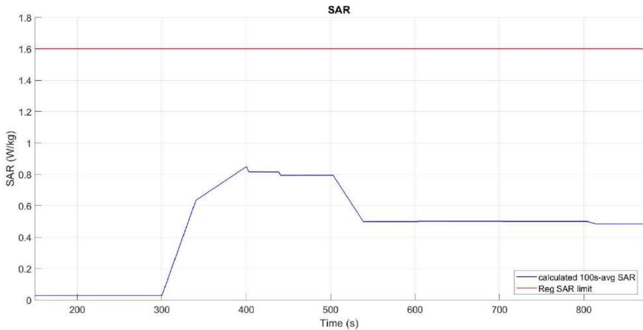
Figure 6- 19 Time-averaged SAR
