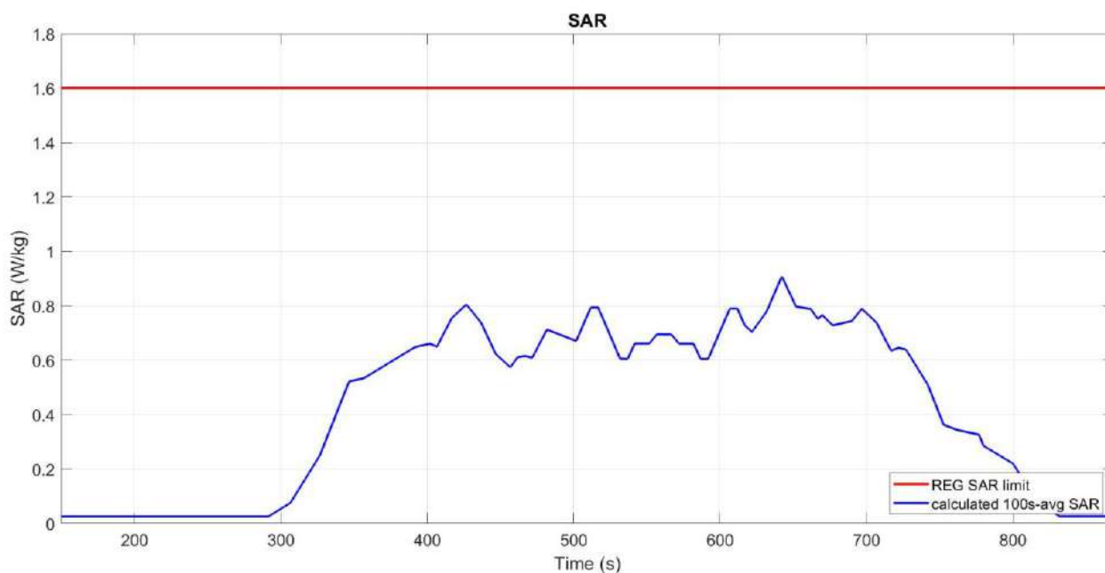
Figure 7-18 Time-averaged SAR
