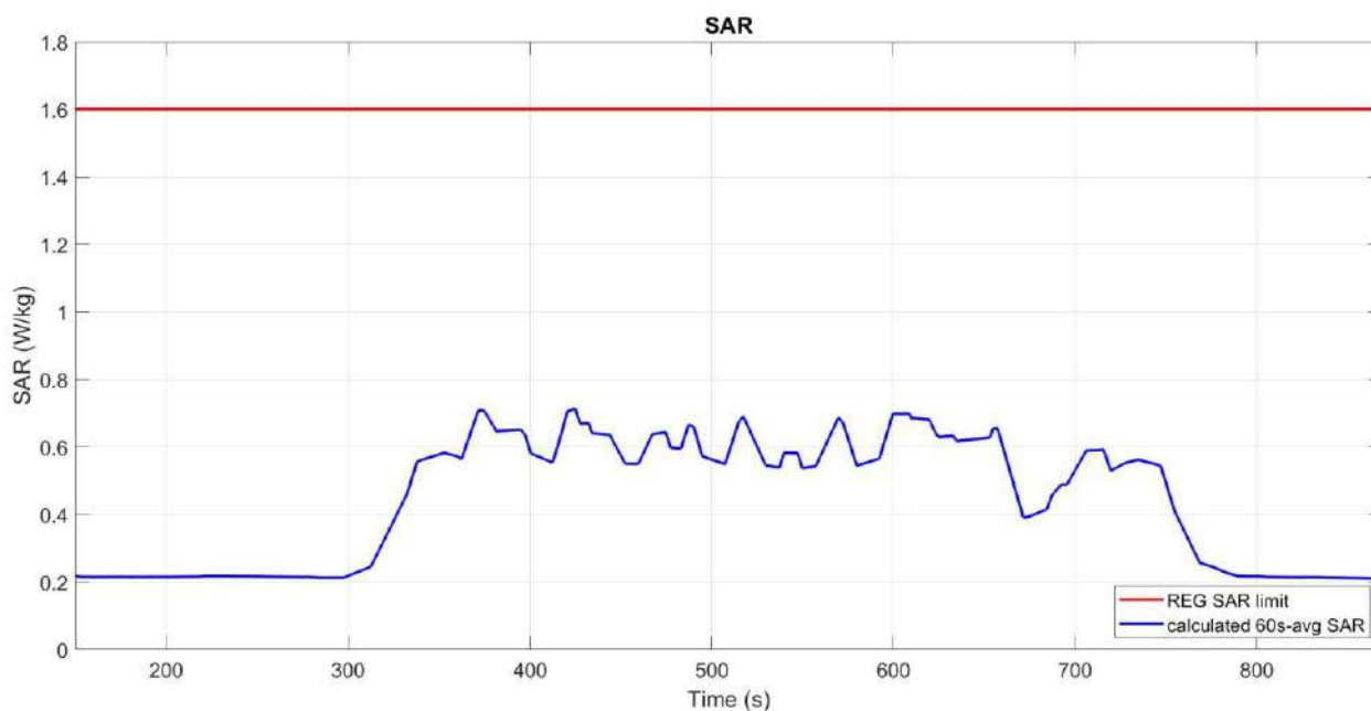
Figure 7-8 Time-averaged SAR
