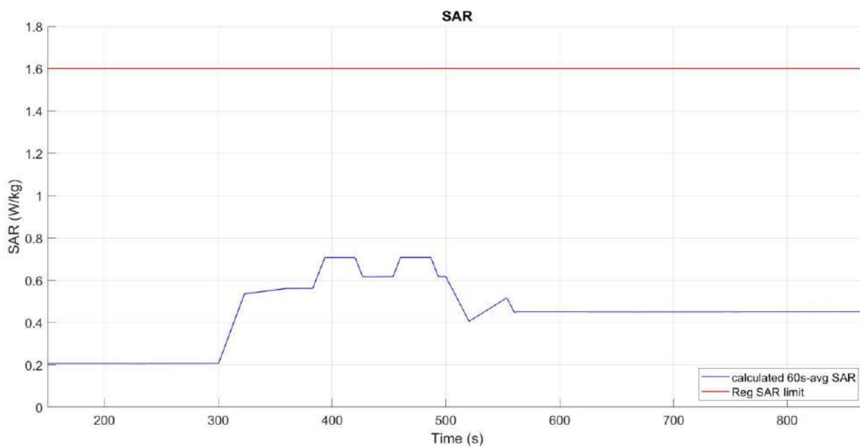
Figure 6- 30 Time-averaged SAR
