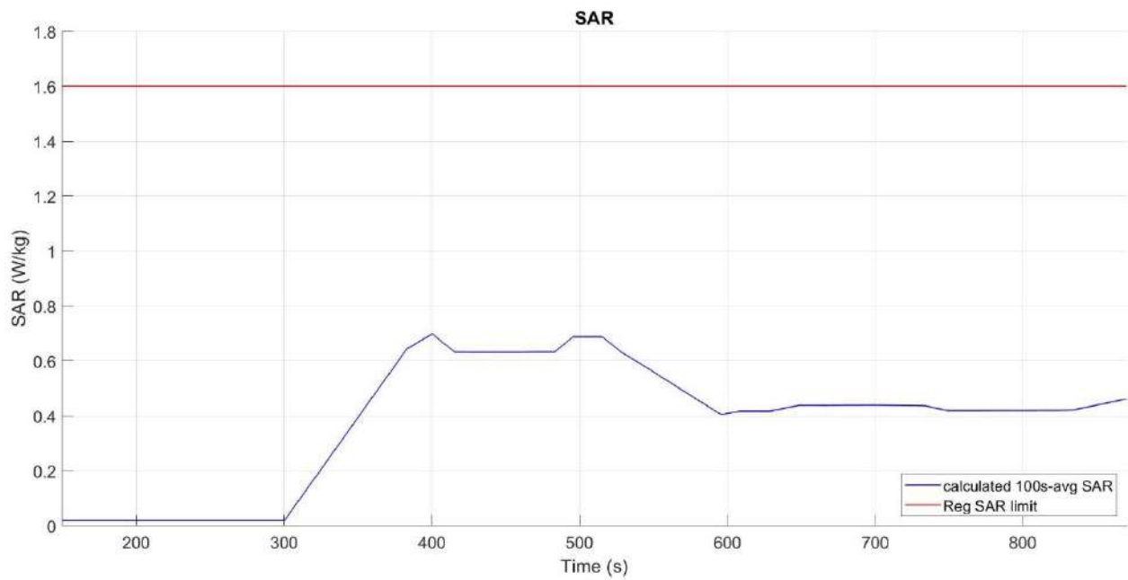
Figure 6- 26 Time-averaged SAR
