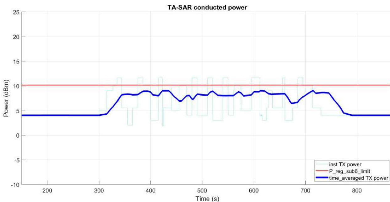
Figure 6- 20 Time-averaged conducted TX power over time
