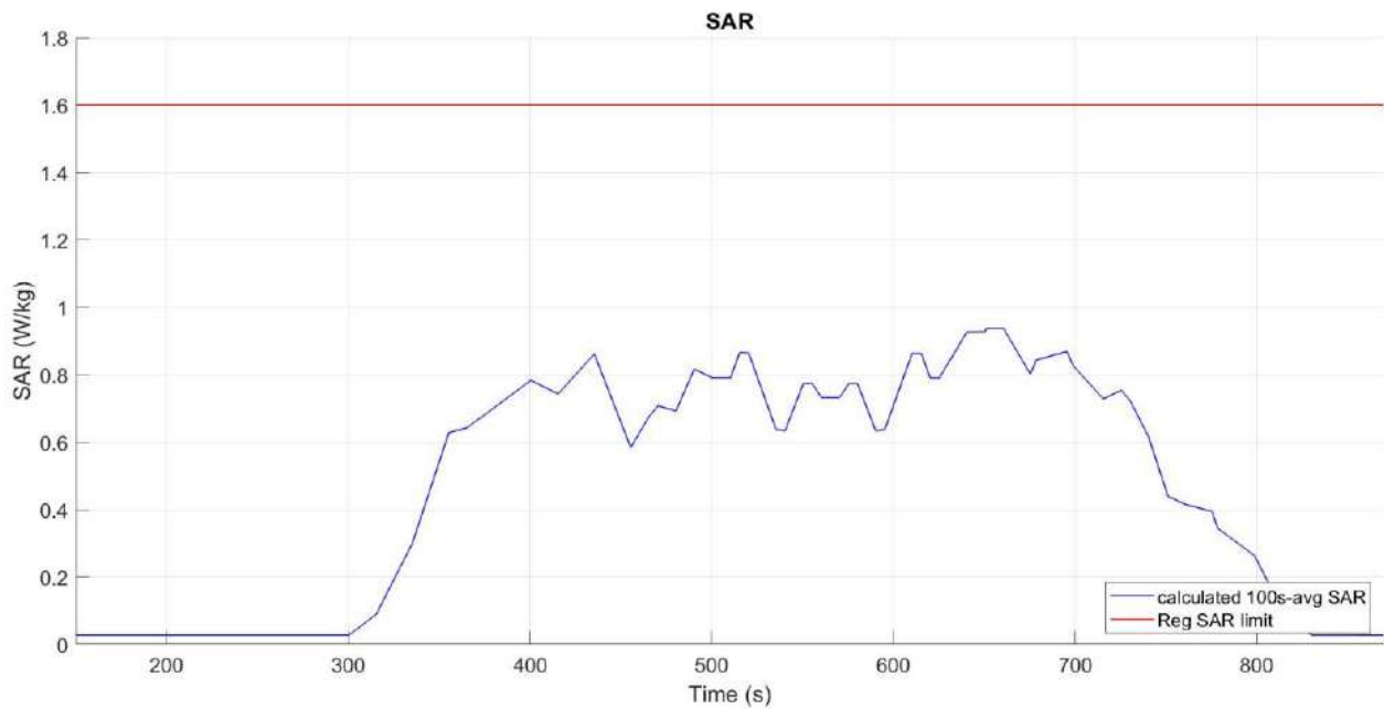
Figure 6- 14 Time-averaged SAR
