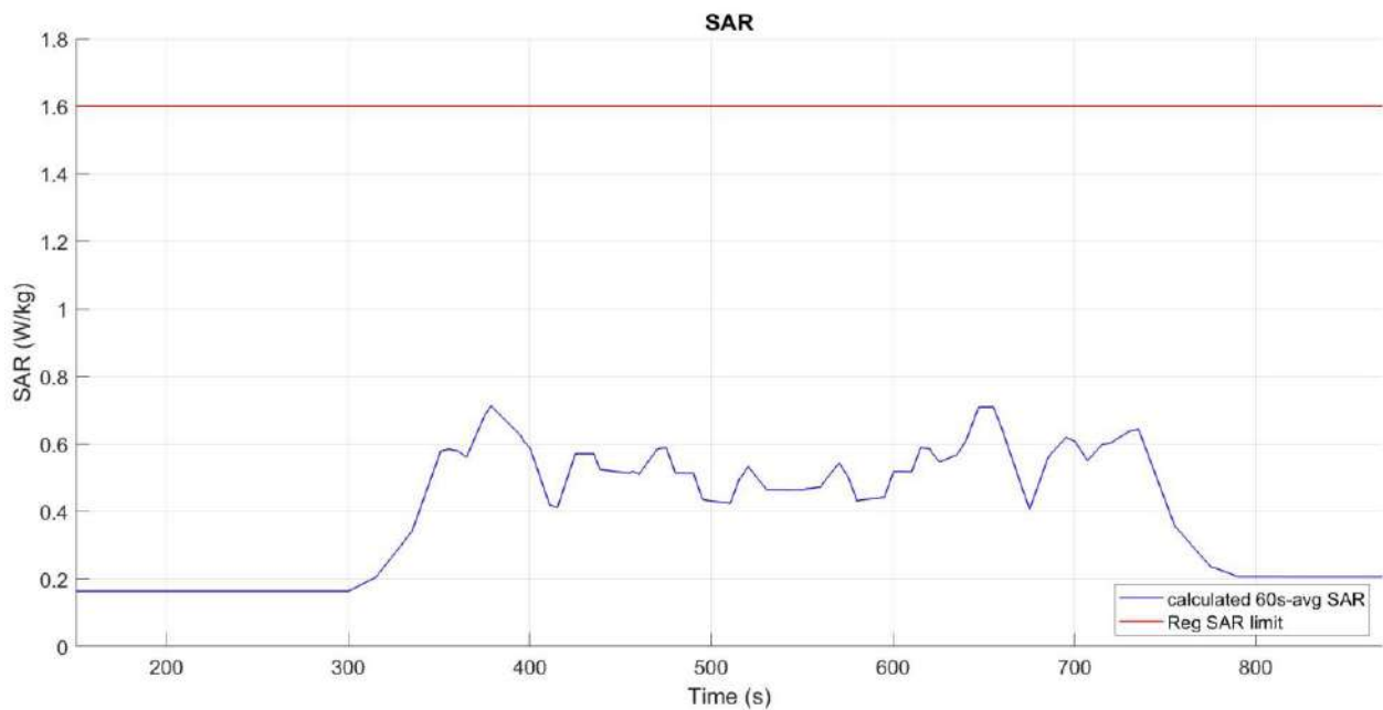
Figure 6- 32 Time-averaged SAR
