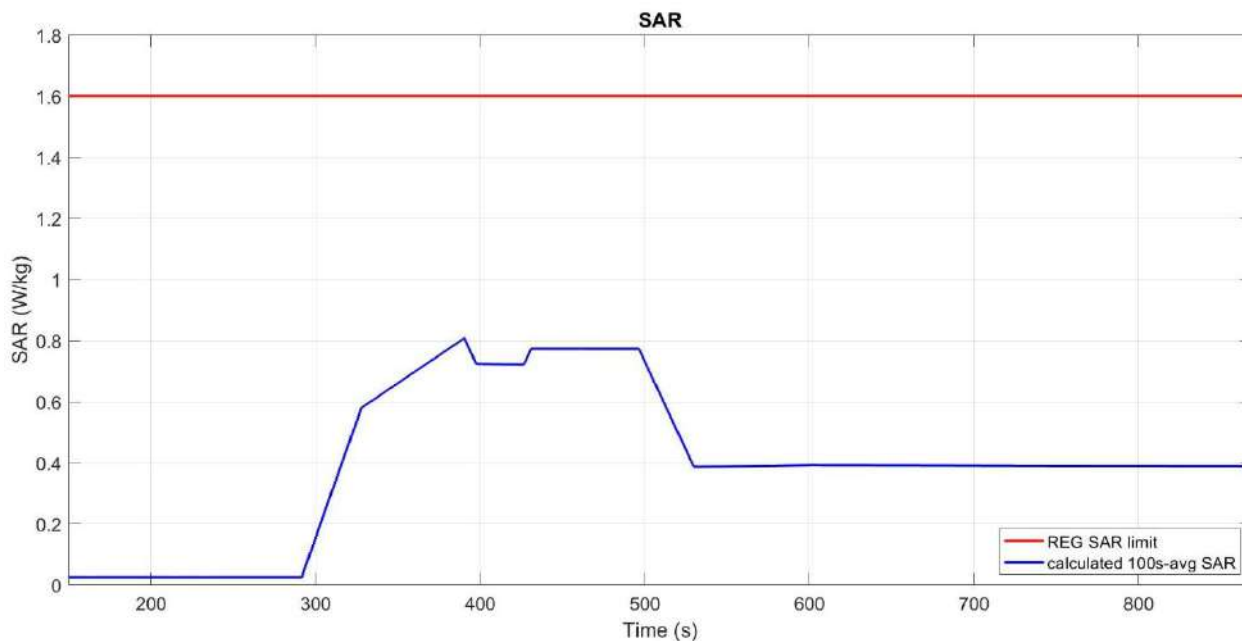
Figure 7-17 Time-averaged SAR
