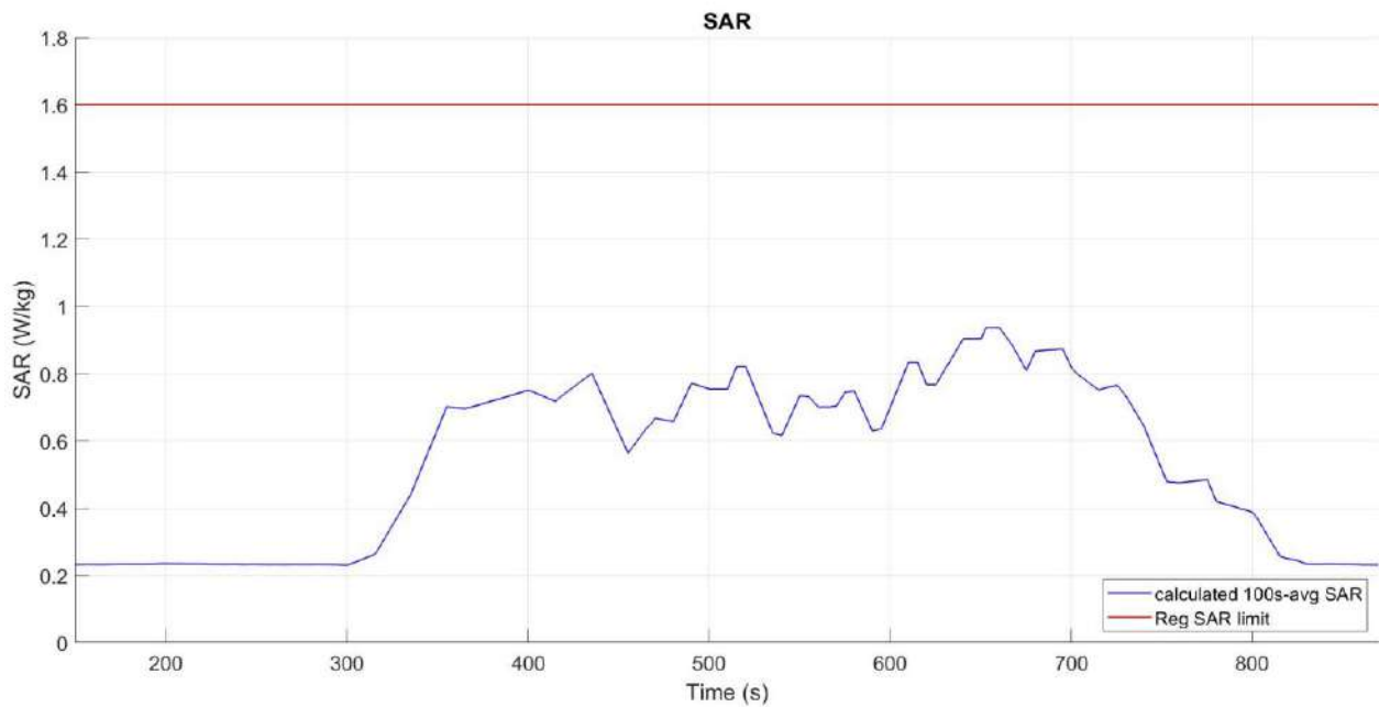
Figure 6- 17 Time-averaged SAR
