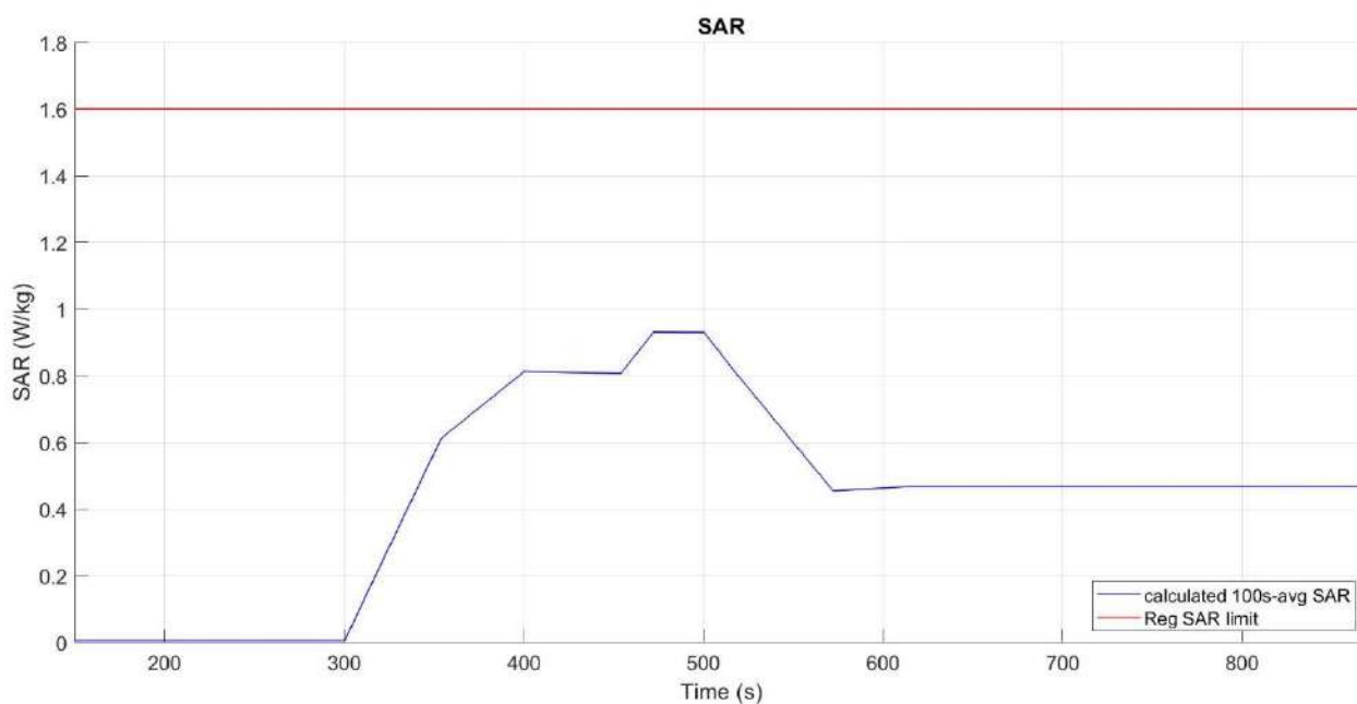
Figure 6- 8 Time-averaged SAR
