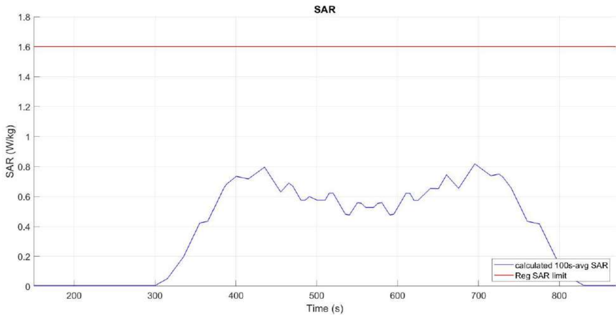
Figure 6- 10 Time-averaged SAR
