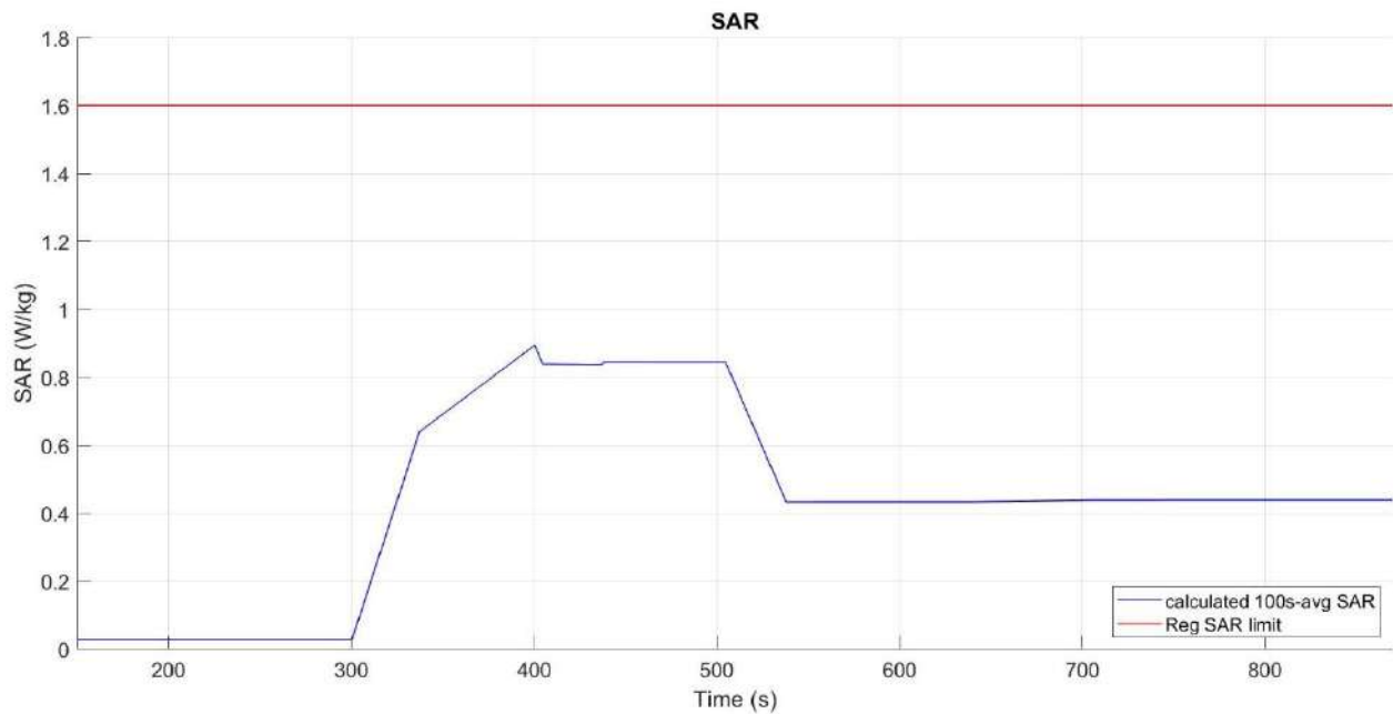
Figure 6- 12 Time-averaged SAR
