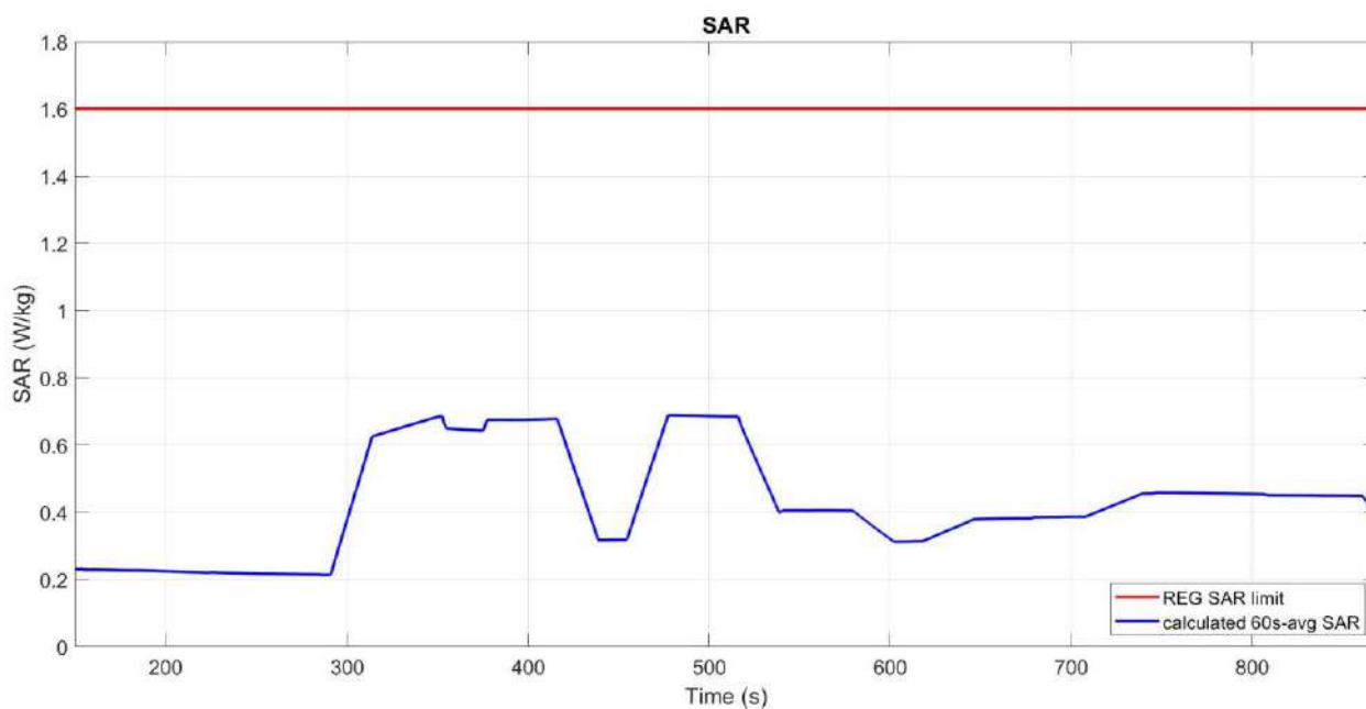
Figure 7-7 Time-averaged SAR
