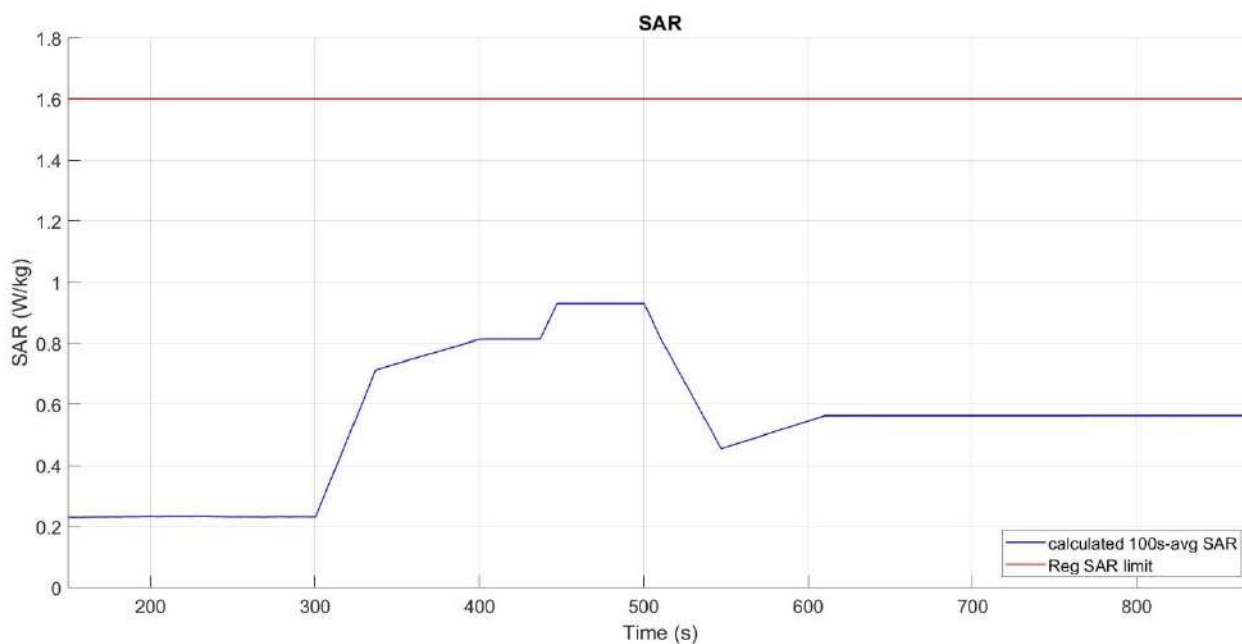
figure 6- 16 Time-averaged SAR
