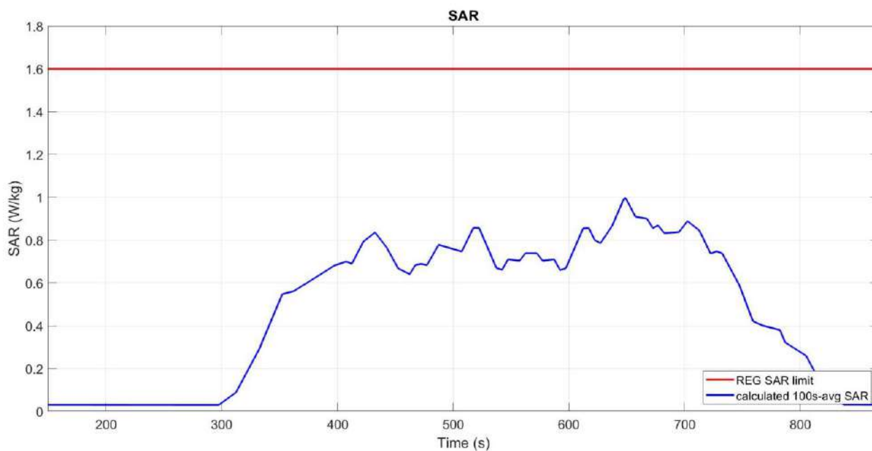
Figure 7-14 Time-averaged SAR
