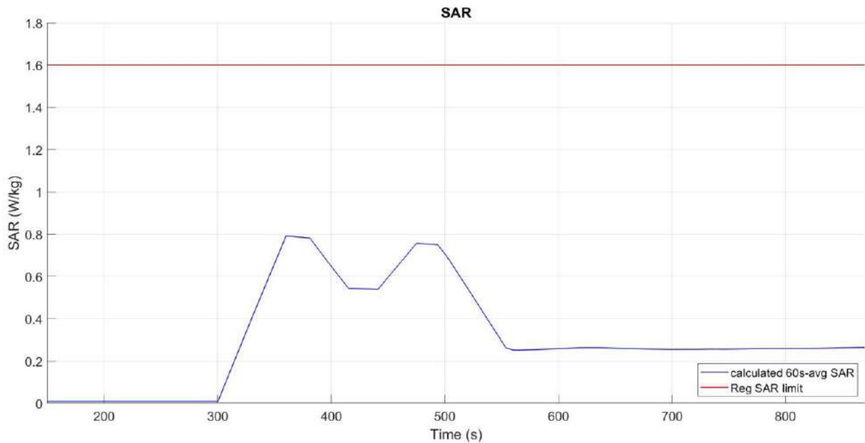
Figure 6- 34 Time-averaged SAR
