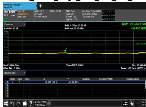
N77(10M)_DFT-s- OFDM_BPSK_Edge_1RB_Left_Mid_CH
