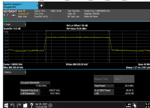
N2(20M)_DFT-s- OFDM_QPSK_Outer_Full_Mid_CH
