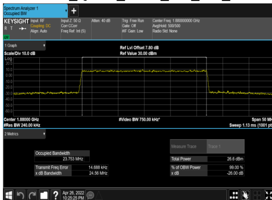
N2(25M)_CP- OFDM_QPSK_Outer_Full_Mid_CH
