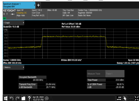
N2(30M)_CP-OFDM_256 QAM_Outer_Full_Mid_CH
