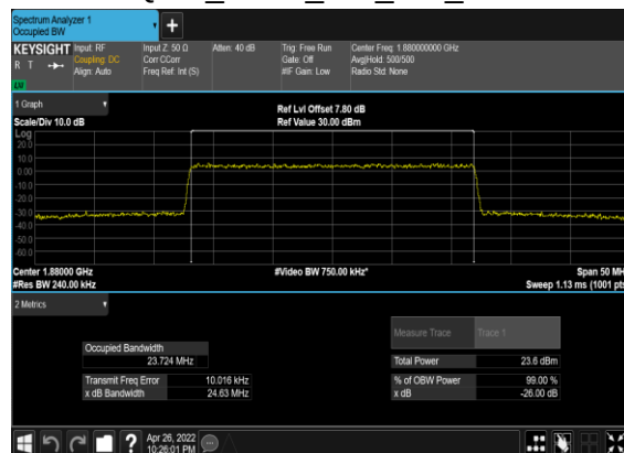
N2(25M)_CP-OFDM_256 QAM_Outer_Full_Mid_CH
