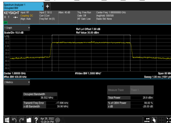
N2(40M)_DFT-s- OFDM_QPSK_Outer_Full_Mid_CH
