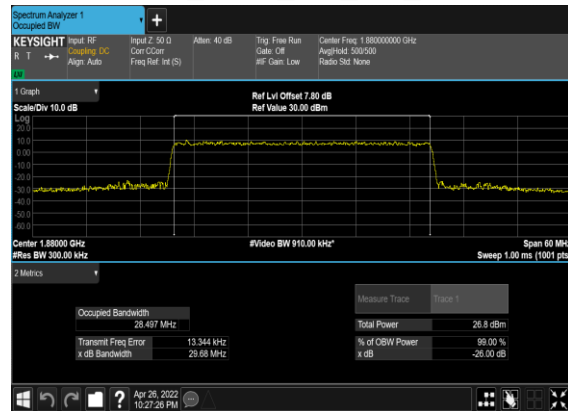
N2(30M)_CP-OFDM_16 QAM_Outer_Full_Mid_CH
