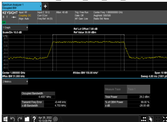
N2(5M)_DFT-s-OFDM_PI_2- BPSK_Outer_Full_Mid_CH
