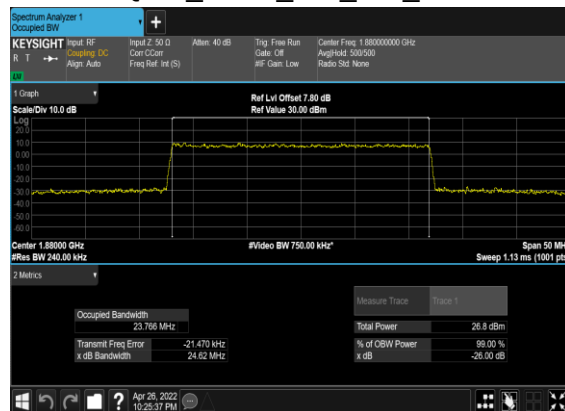
N2(25M)_CP-OFDM_16 QAM_Outer_Full_Mid_CH
