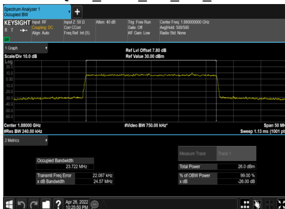
N2(25M)_CP-OFDM_64 QAM_Outer_Full_Mid_CH
