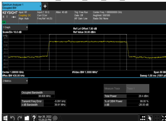
N2(40M)_DFT-s-OFDM_PI_2- BPSK_Outer_Full_Mid_CH
