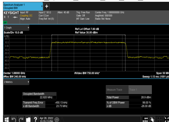
N2(25M)_DFT-s- OFDM_QPSK_Outer_Full_Mid_CH
