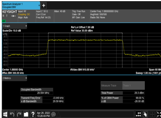
N2(30M)_DFT-s-OFDM_PI_2- BPSK_Outer_Full_Mid_CH
