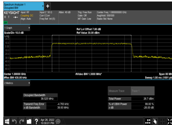
N2(40M)_CP-OFDM_16 QAM_Outer_Full_Mid_CH
