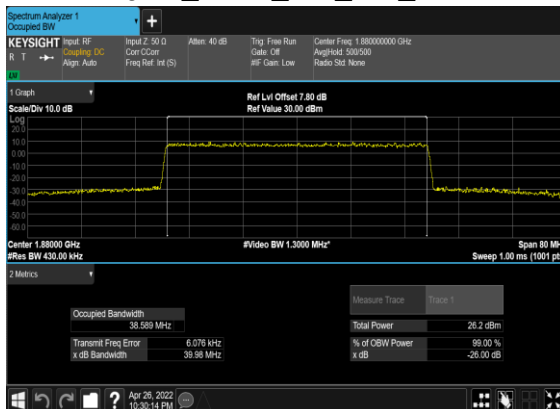
N2(40M)_CP-OFDM_64 QAM_Outer_Full_Mid_CH
