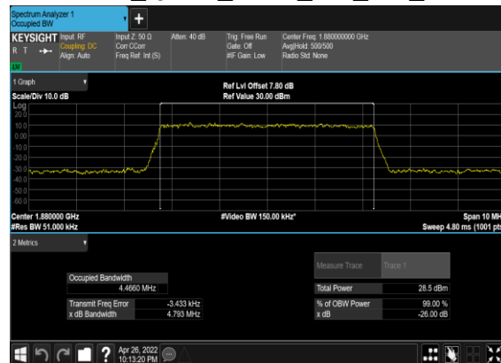
N2(5M)_DFT-s- OFDM_QPSK_Outer_Full_Mid_CH
