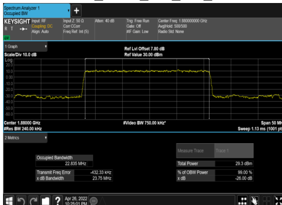
N2(25M)_DFT-s-OFDM_PI_2- BPSK_Outer_Full_Mid_CH
