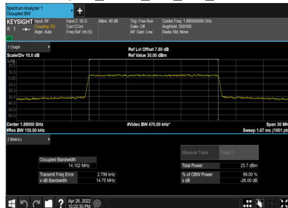
N2(15M)_CP-OFDM_256 QAM_Outer_Full_Mid_CH
