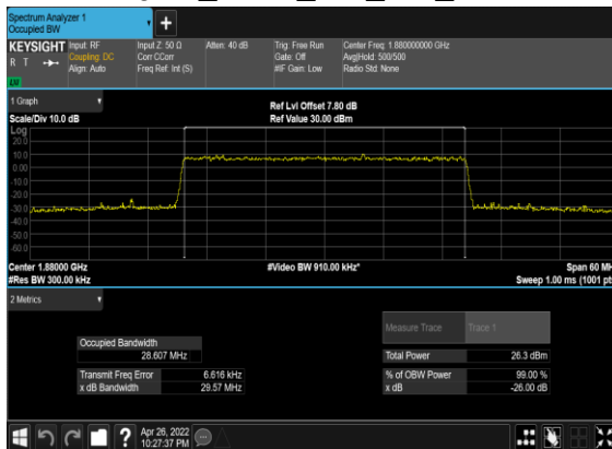
N2(30M)_CP-OFDM_64 QAM_Outer_Full_Mid_CH
