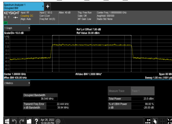
N2(40M)_CP-OFDM_256 QAM_Outer_Full_Mid_CH
