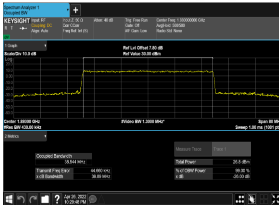
N2(40M)_CP- OFDM_QPSK_Outer_Full_Mid_CH
