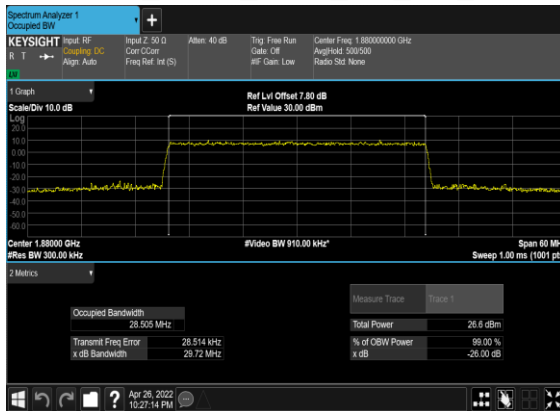
N2(30M)_CP- OFDM_QPSK_Outer_Full_Mid_CH
