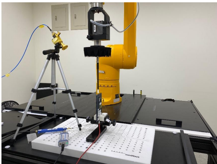
Top, Test separation 2mm
