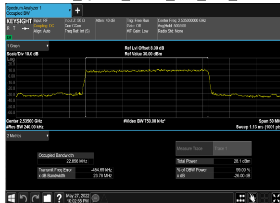
B2_N7(25M)_DFT-s- OFDM_QPSK_Outer_Full_Mid_CH
