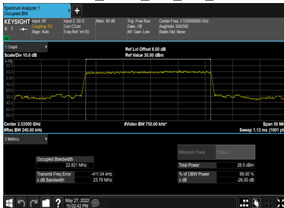
B2_N7(25M)_DFT-s-OFDM_PI_2- BPSK_Outer_Full_Mid_CH
