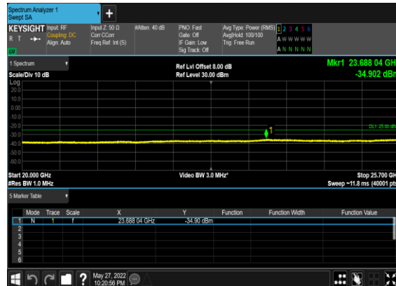
B2_N7(20M)_DFT-s-OFDM_QPSK_Edge_1RB_Left_Mid_CH
