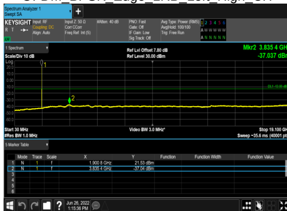
B7_N2(10M)_DFT-s-OFDM BPSK Edge 1RB Left High CH
