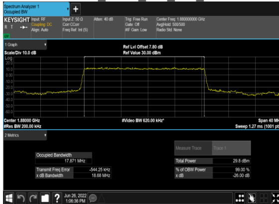
B7_N2(20M)_DFT-s-OFDM_PI_2- BPSK Outer Full Mid CH
