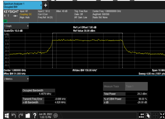
B7_N2(5M)_DFT-s- OFDM QPSK Outer Full Mid CH
