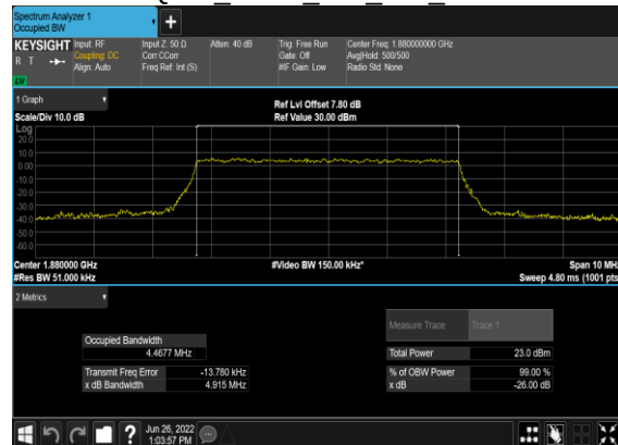
B7_N2(5M)_CP-OFDM_256 QAM Outer Full Mid CH
