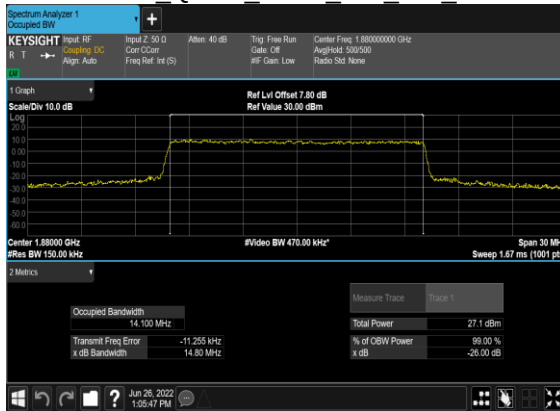
B7_N2(15M)_CP- OFDM QPSK Outer Full Mid CH
