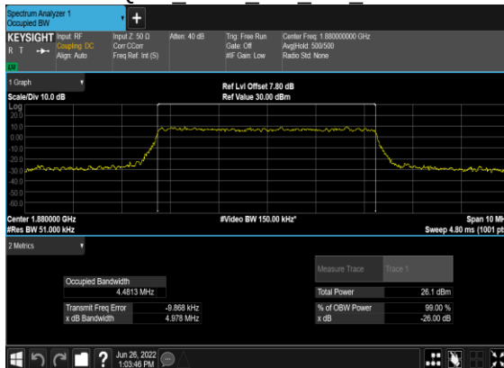
B7_N2(5M)_CP-OFDM_64 QAM Outer Full Mid CH
