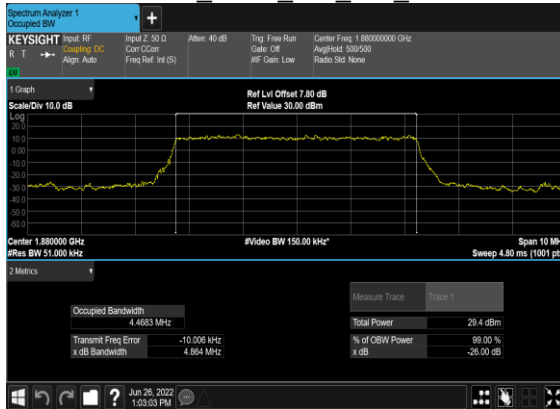
B7_N2(5M)_DFT-s-OFDM_PI_2- BPSK Outer Full Mid CH
