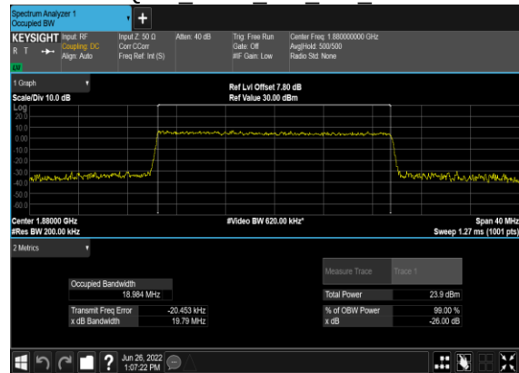
B7_N2(20M)_CP-OFDM_256 QAM Outer Full Mid CH
