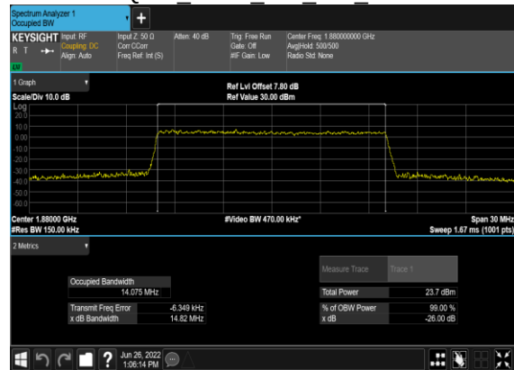
B7_N2(15M)_CP-OFDM_256 QAM Outer Full Mid CH
