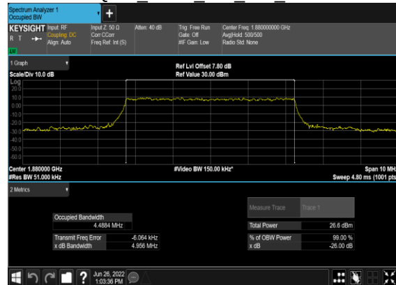
B7_N2(5M)_CP-OFDM_16 QAM Outer Full Mid CH
