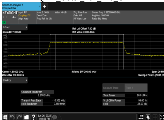
B7_N2(10M)_CP-OFDM_64 QAM Outer Full Mid CH
