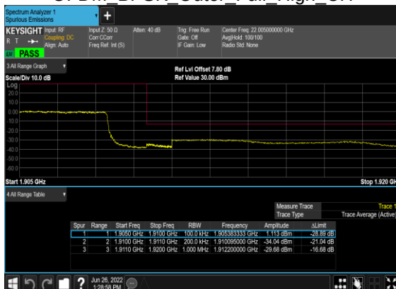
B7_N2(20M)_DFT-s- OFDM BPSK Outer Full High CH
