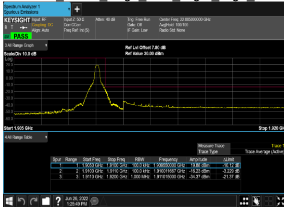
B7_N2(10M)_DFT-s-OFDM BPSK Edge 1RB Right High CH
