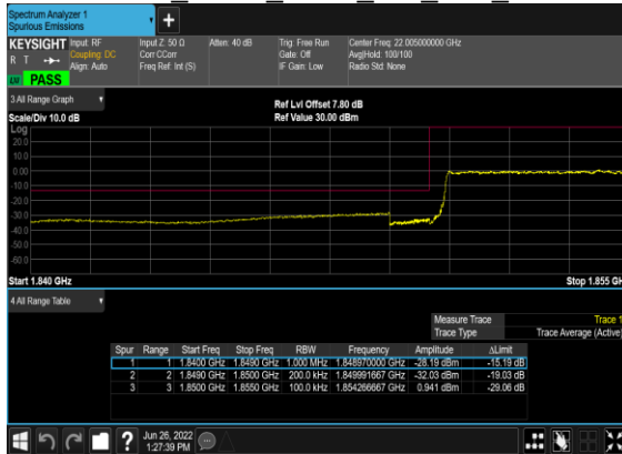
B7_N2(20M)_DFT-s- OFDM BPSK Outer Full Low CH
