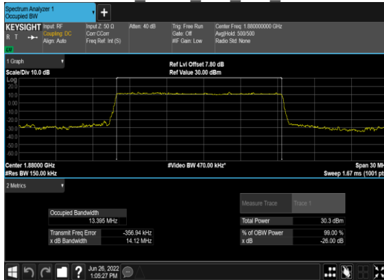
B7_N2(15M)_DFT-s-OFDM_PI_2- BPSK Outer Full Mid CH
