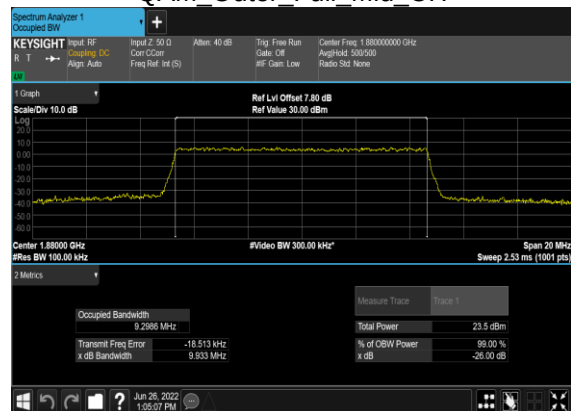
B7_N2(10M)_CP-OFDM_256 QAM Outer Full Mid CH
