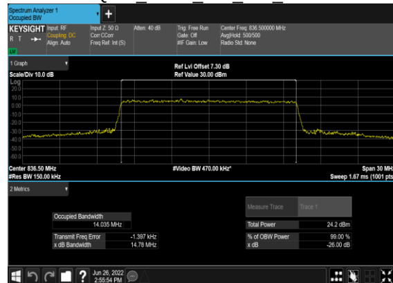
B7_N5(15M)_CP-OFDM_256 QAM Outer Full Mid CH
