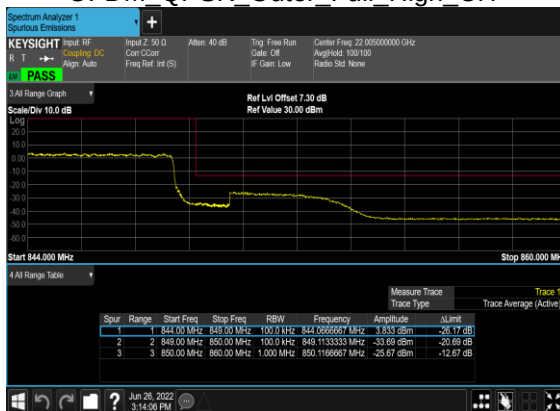
B7_N5(10M)_DFT-s-OFDM QPSK Outer Full High CH
