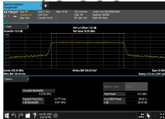
B7_N5(10M)_CP-OFDM_256 QAM Outer Full Mid CH
