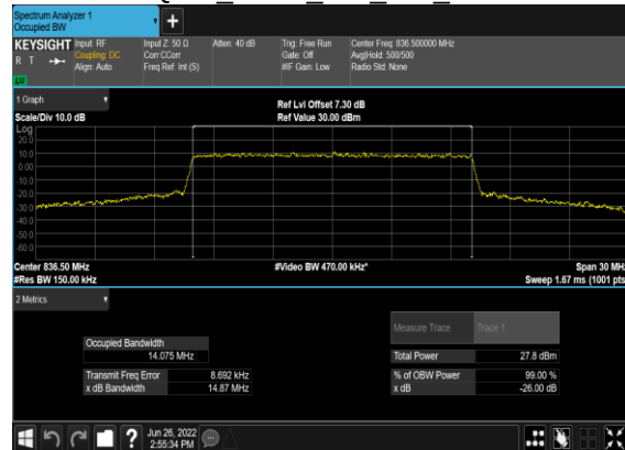
B7_N5(15M)_CP-OFDM_16 QAM Outer Full Mid CH
