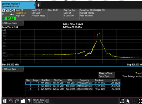
B7_N5(10M)_DFT-s- OFDM QPSK Edge 1RB Left Low CH
