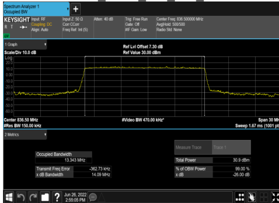
B7_N5(15M)_DFT-s-OFDM_PI_2- BPSK Outer Full Mid CH
