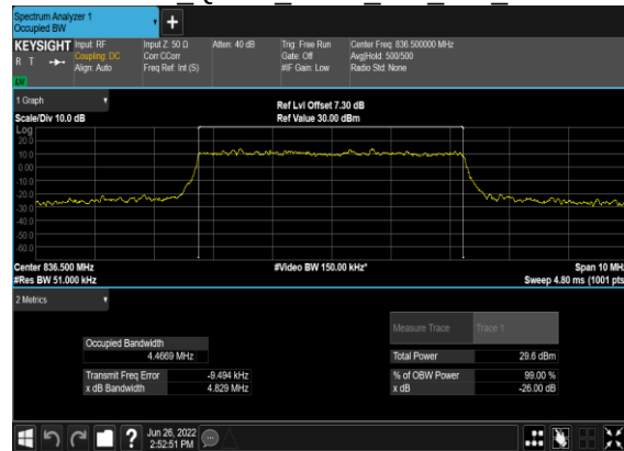
B7_N5(5M)_DFT-s- OFDM QPSK Outer Full Mid CH
