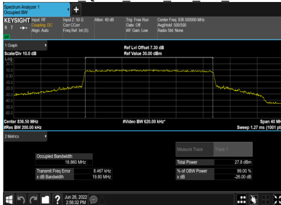
B7_N5(20M)_CP- OFDM QPSK Outer Full Mid CH
