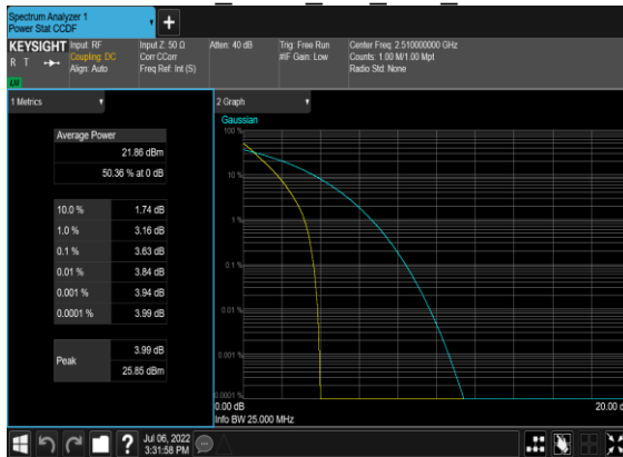
N7(20M)_DFT-s-OFDM_PI_2-BPSK Outer Full Low CH
