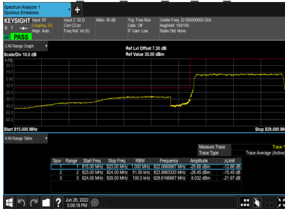
B7_N5(5M)_DFT-s- OFDM BPSK Outer Full Low CH
