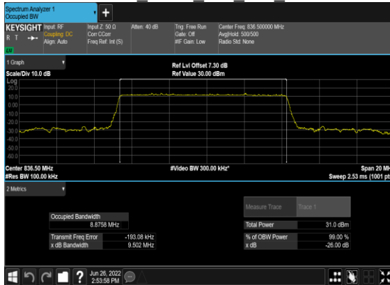
B7_N5(10M)_DFT-s-OFDM_PI_2- BPSK Outer Full Mid CH
