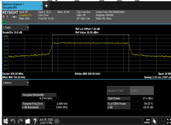
B7_N5(10M)_CP- OFDM QPSK Outer Full Mid CH
