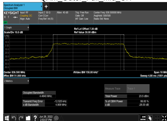
B7_N5(5M)_CP-OFDM_256 QAM Outer Full Mid CH
