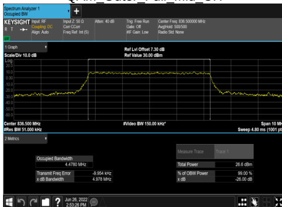
B7_N5(5M)_CP-OFDM_64 QAM Outer Full Mid CH
