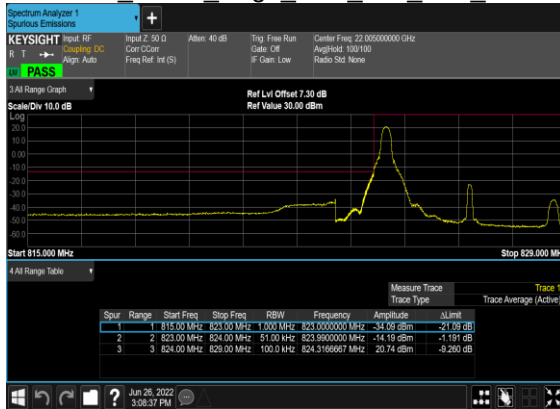
B7_N5(5M)_DFT-s- OFDM BPSK Edge 1RB Left Low CH
