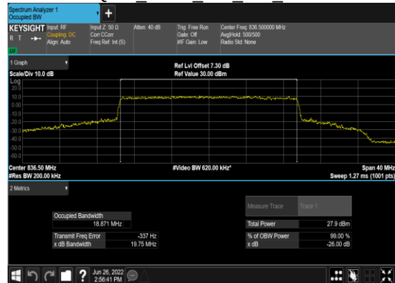
B7_N5(20M)_CP-OFDM_16 QAM Outer Full Mid CH
