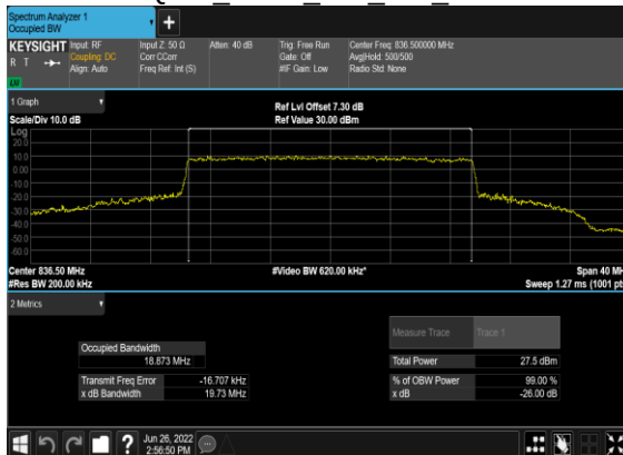
B7_N5(20M)_CP-OFDM_64 QAM Outer Full Mid CH
