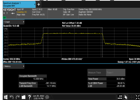
B7_N5(15M)_DFT-s- OFDM QPSK Outer Full Mid CH
