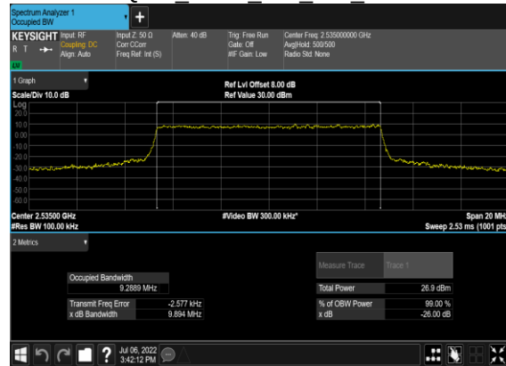
N7(10M)_CP-OFDM_16 QAM Outer Full Mid CH
