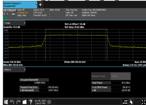
B7_N5(10M)_DFT-s- OFDM QPSK Outer Full Mid CH
