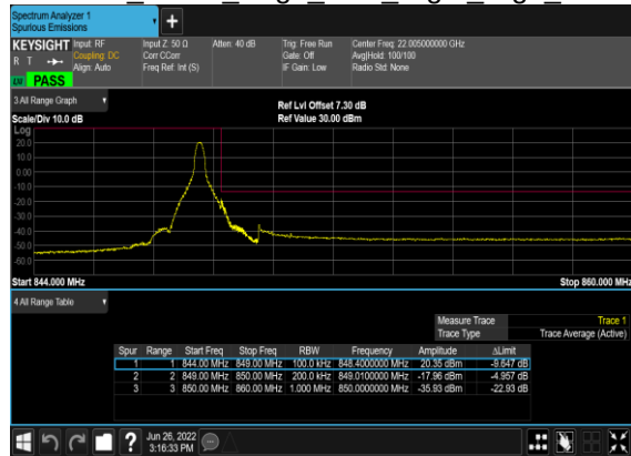
B7_N5(20M)_DFT-s- OFDM BPSK Edge 1RB Right High CH
