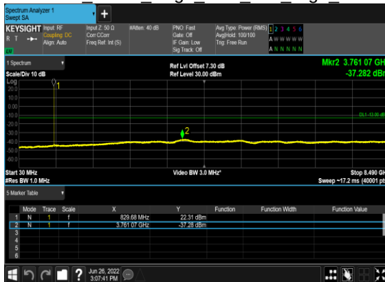
B7_N5(20M)_DFT-s-OFDM BPSK Edge 1RB Left High CH
