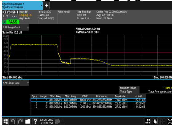
B7_N5(5M)_DFT-s- OFDM BPSK Outer Full High CH
