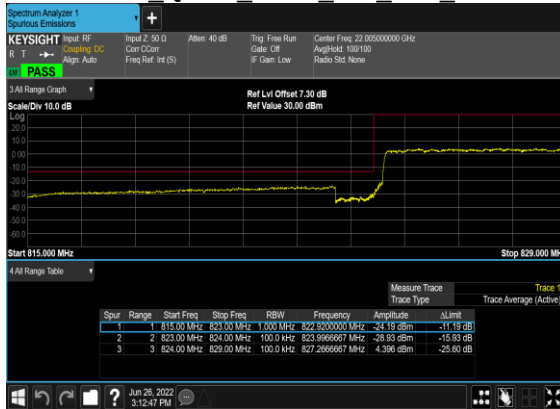
B7_N5(10M)_DFT-s-OFDM QPSK Outer Full Low CH
