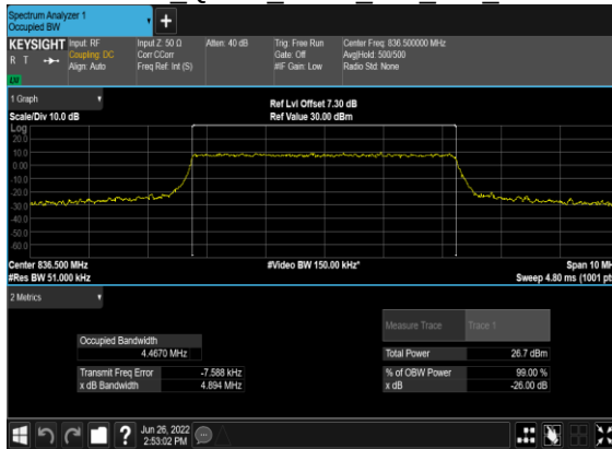
B7_N5(5M)_CP- OFDM QPSK Outer Full Mid CH
