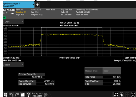
B7_N5(20M)_CP-OFDM_256 QAM Outer Full Mid CH
