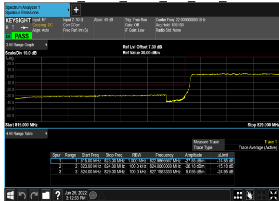
B7_N5(10M)_DFT-s- OFDM BPSK Outer Full Low CH
