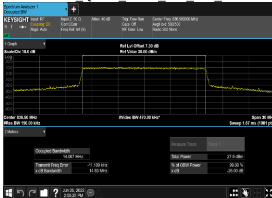
B7_N5(15M)_CP- OFDM QPSK Outer Full Mid CH
