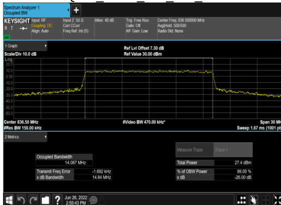
B7_N5(15M)_CP-OFDM_64 QAM Outer Full Mid CH
