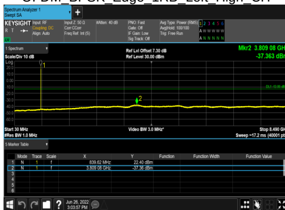
B7_N5(10M)_DFT-s- OFDM BPSK Edge 1RB Left High CH
