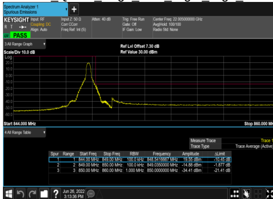
B7_N5(10M)_DFT-s-OFDM QPSK Edge 1RB Right High CH
