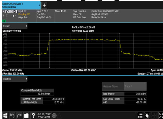
B7_N5(20M)_DFT-s-OFDM_PI_2- BPSK Outer Full Mid CH
