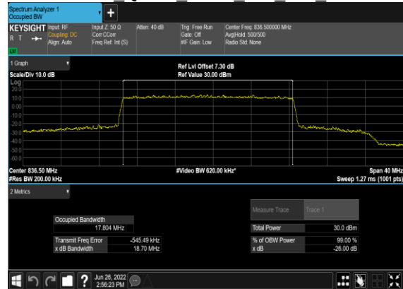
B7_N5(20M)_DFT-s- OFDM QPSK Outer Full Mid CH
