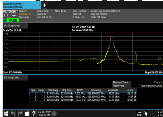
B7_N5(5M)_DFT-s- OFDM QPSK Edge 1RB Left Low CH
