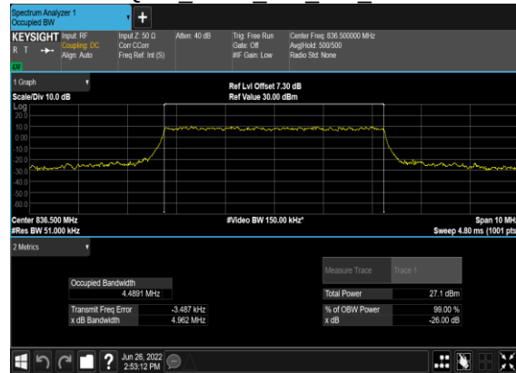
B7_N5(5M)_CP-OFDM_16 QAM Outer Full Mid CH
