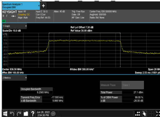
B7_N5(10M)_CP-OFDM_64 QAM Outer Full Mid CH
