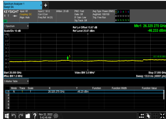
N48(40M)_DFT-s- OFDM_QPSK_Edge_1RB_Right_Low_CH
