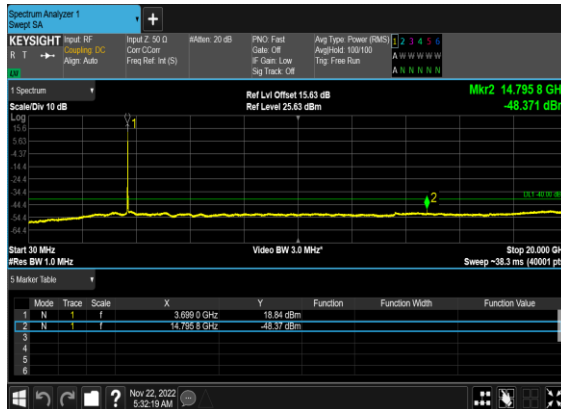
N48(20M)_DFT-s- OFDM_BPSK_Edge_1RB_Right_High_CH
