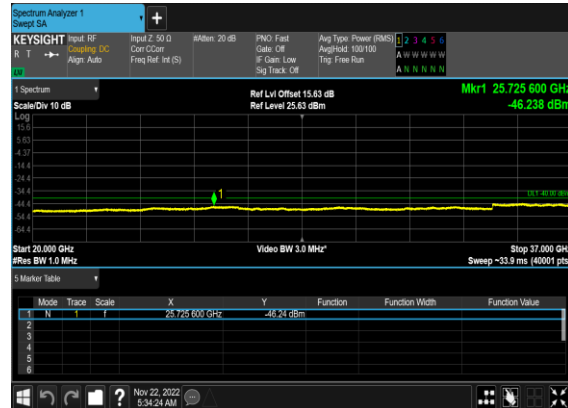
N48(20M)_DFT-s- OFDM_QPSK_Edge_1RB_Right_High_CH
