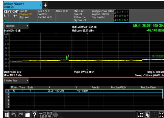
N48(20M)_DFT-s- OFDM_QPSK_Edge_1RB_Right_Mid_CH
