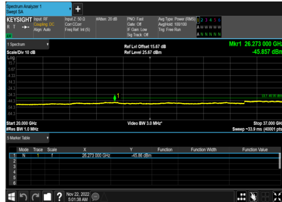
N48(10M)_DFT-s- OFDM_QPSK_Edge_1RB_Right_Mid_CH
