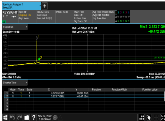
N48(20M)_DFT-s- OFDM_BPSK_Outer_Full_Mid_CH
