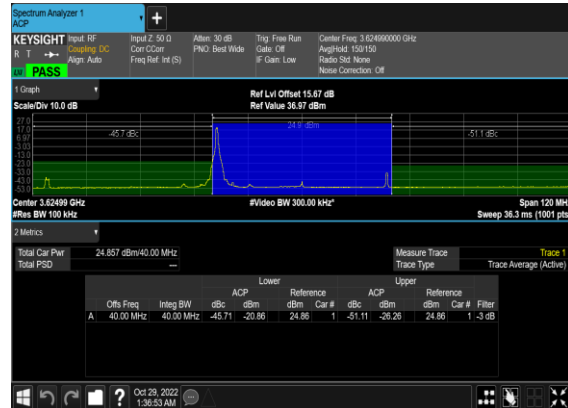
N48(40M)_DFT-s-OFDM_PI_2-BPSK_Edge_1RB_Left_Mid_CH
