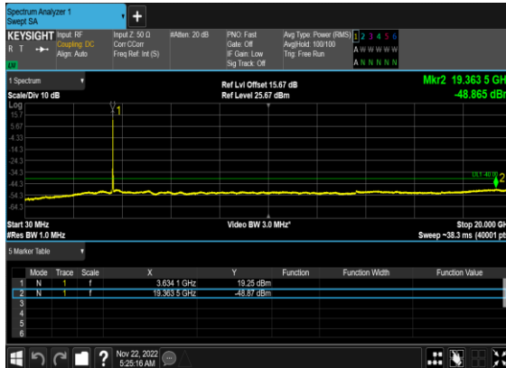
N48(20M)_DFT-s- OFDM_QPSK_Edge_1RB_Right_Mid_CH
