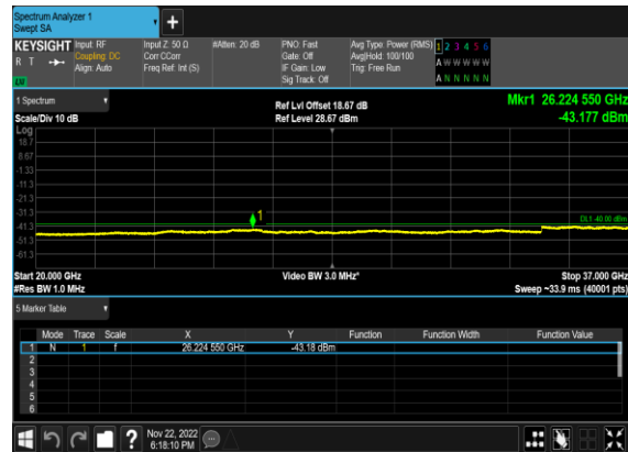
N48(40M)_CP- OFDM_QPSK_Edge_1RB_Right_High_CH
