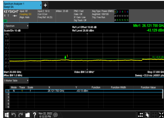
N48(40M)_CP- OFDM_QPSK_Edge_1RB_Left_Mid_CH
