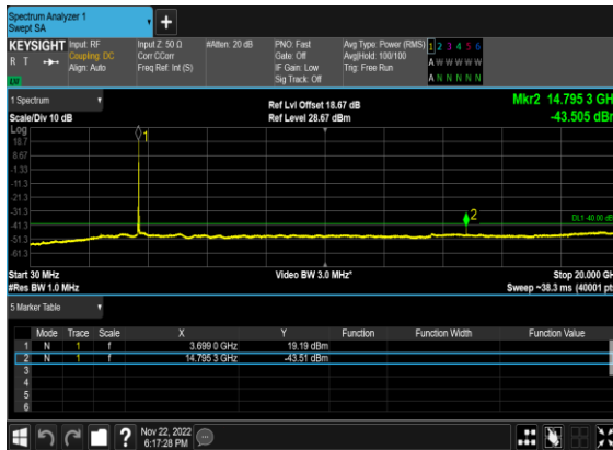
N48(40M)_CP- OFDM_QPSK_Edge_1RB_Right_High_CH
