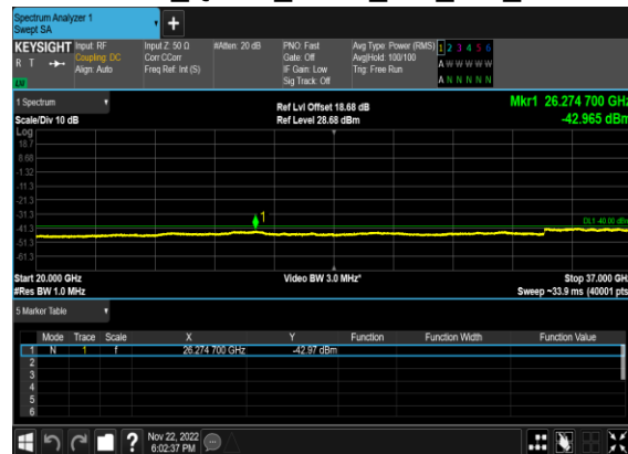
N48(20M)_CP- OFDM_QPSK_Outer_Full_Mid_CH
