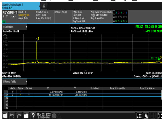
N48(40M)_CP- OFDM_QPSK_Outer_Full_High_CH
