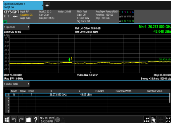
N48(20M)_CP- OFDM_QPSK_Edge_1RB_Left_High_CH
