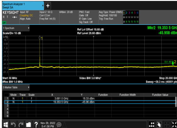
N48(20M)_CP- OFDM_QPSK_Edge_1RB_Left_High_CH
