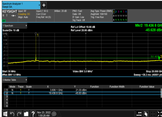
N48(40M)_CP- OFDM_QPSK_Edge_1RB_Left_Mid_CH
