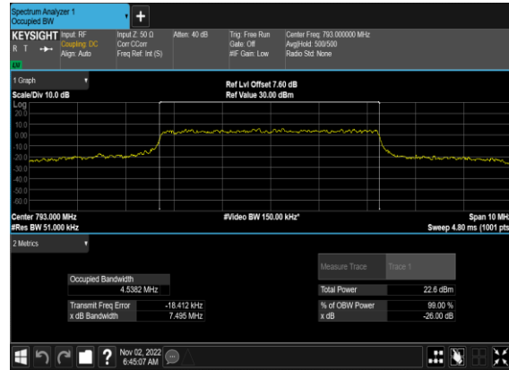
N14(5M)_CP-OFDM_16 QAM_Outer_Full_Mid_CH
