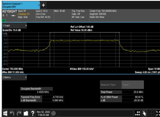
N14(5M)_DFT-s-OFDM_PI_2- BPSK_Outer_Full_Mid_CH
