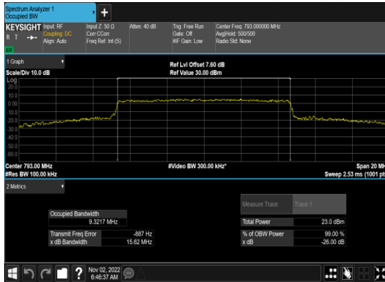
N14(10M)_CP-OFDM_QPSK_Outer_Full_Mid_CH
