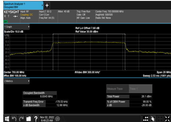
N14(10M)_DFT-s-OFDM_QPSK_Outer_Full_Mid_CH
