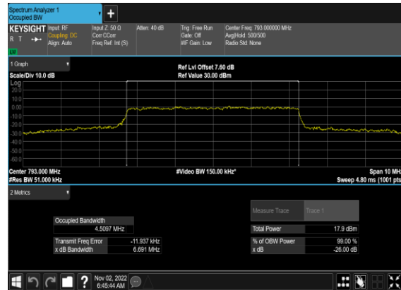
N14(5M)_CP-OFDM_256 QAM_Outer_Full_Mid_CH
