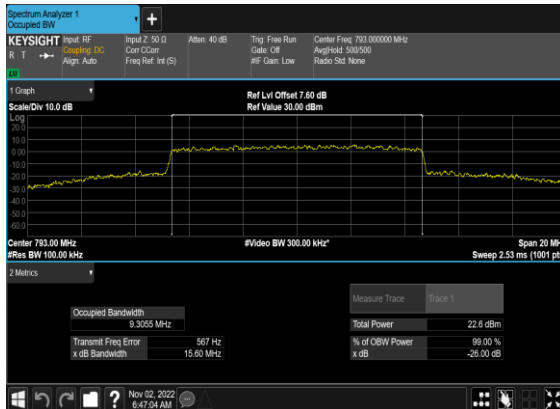
N14(10M)_CP-OFDM_64QAM_Outer_Full_Mid_CH
