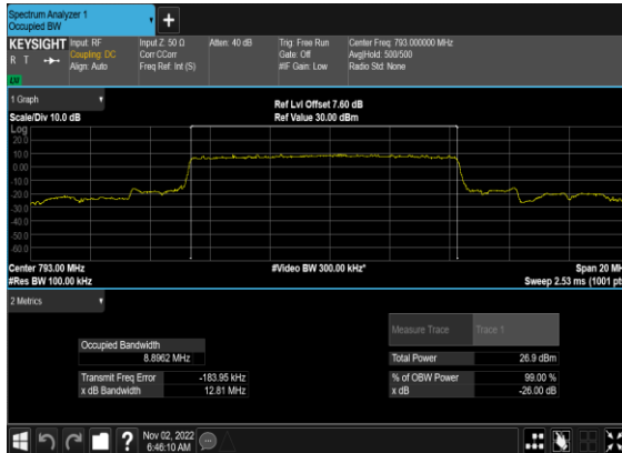
N14(10M)_DFT-s-OFDM_PI_2- BPSK_Outer_Full_Mid_CH
