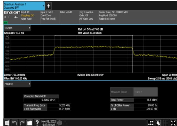
N14(10M)_CP-OFDM_256QAM_Outer_Full_Mid_CH
