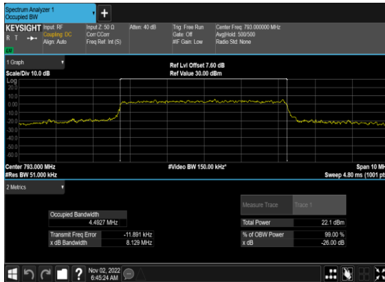
N14(5M)_CP-OFDM_64 QAM_Outer_Full_Mid_CH
