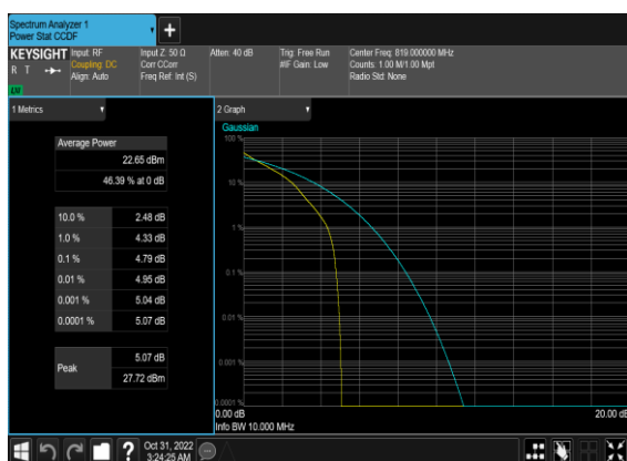
N26(10M)_DFT-s-OFDM_QPSK_Outer_Full_Mid_ CH
