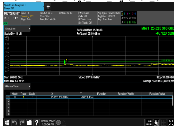
N48(10M)_DFT-s- OFDM BPSK Edge 1RB Right Low CH
