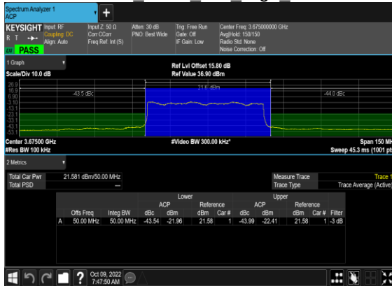
N48(50M)_DFT-s-OFDM_PI_2- BPSK Outer Full High CH
