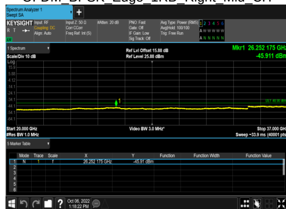
N48(10M)_DFT-s-OFDM BPSK Edge 1RB Right Mid CH
