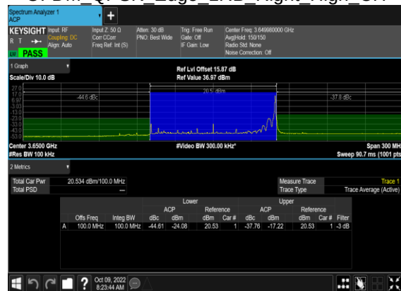
N48(100M)_DFT-s- OFDM QPSK Edge 1RB Right High CH
