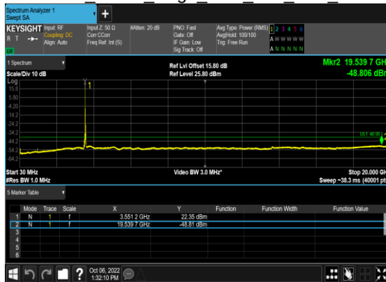
N48(50M)_DFT-s- OFDM BPSK Edge 1RB Left Low CH
