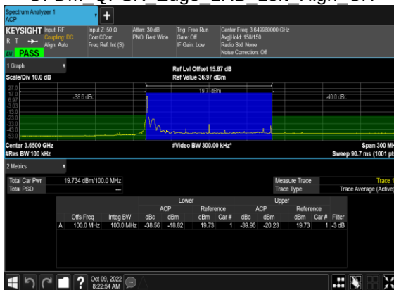
N48(100M)_DFT-s- OFDM QPSK Edge 1RB Left High CH
