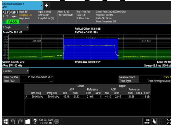
N48(50M)_DFT-s-OFDM_PI_2- BPSK Outer Full_Mid_CH
