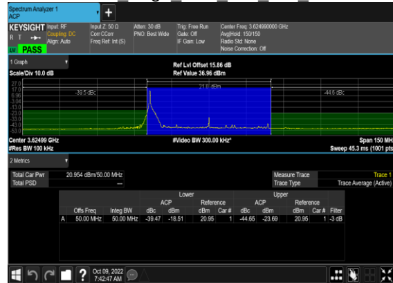
N48(50M)_DFT-s-OFDM_PI_2- BPSK Edge_1RB Left_Mid_CH
