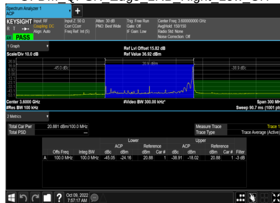
N48(100M)_DFT-s-OFDM QPSK Edge 1RB Right Low CH
