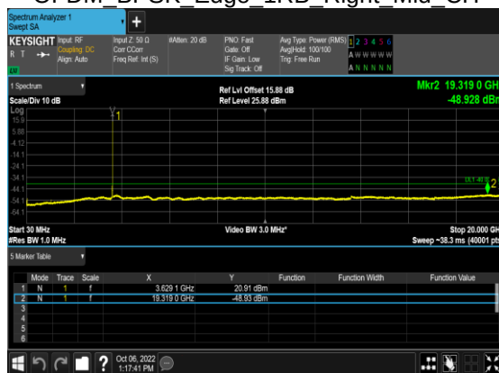
N48(10M)_DFT-s-OFDM BPSK Edge 1RB Right Mid CH
