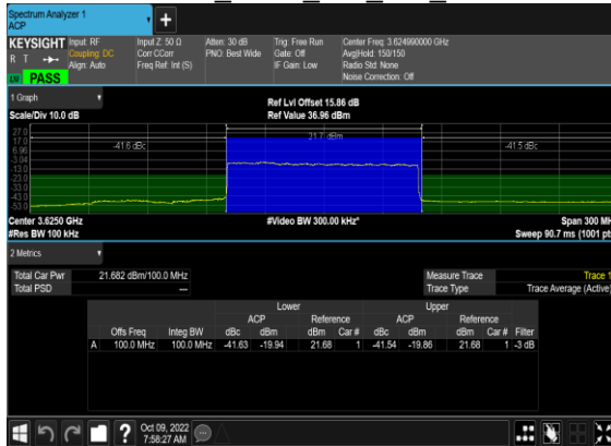
N48(100M)_DFT-s-OFDM_PI_2- BPSK Outer Full Mid CH
