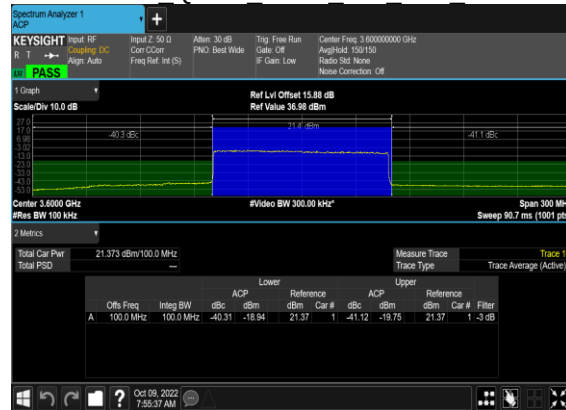
N48(100M)_DFT-s-OFDM QPSK Outer Full Low CH
