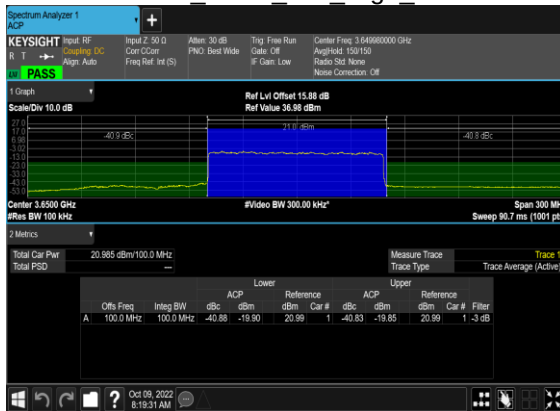
N48(100M)_DFT-s-OFDM_PI_2- BPSK Outer Full High CH
