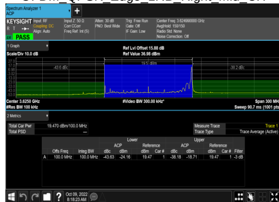
N48(100M)_DFT-s- OFDM QPSK Edge 1RB Right Mid CH
