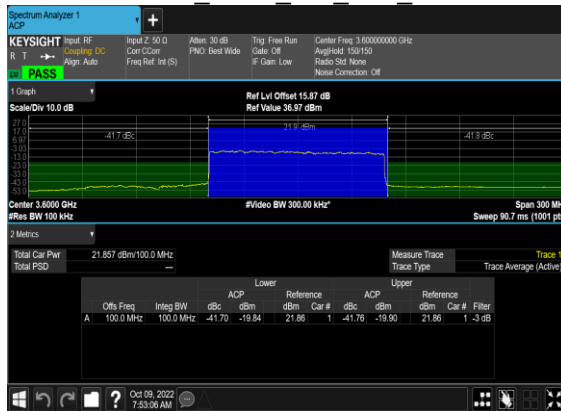
N48(100M)_DFT-s-OFDM_PI_2-BPSK Outer Full Low CH
