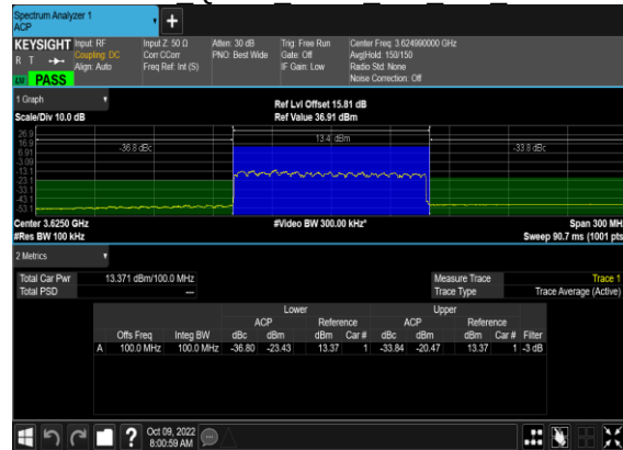
N48(100M)_DFT-s- OFDM QPSK Outer Full Mid CH
