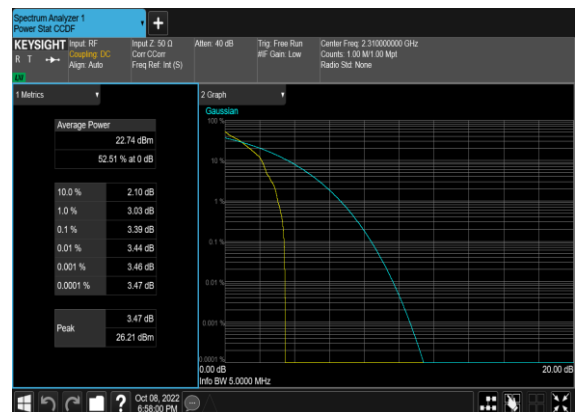
N30(5M)_DFT-s-OFDM_PI_2-BPSK_Edge_1RB_Left_ Mid_CH
