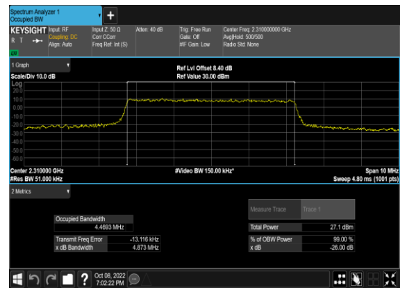
N30(5M)_CP-OFDM_16 QAM_Outer_Full_Mid_CH
