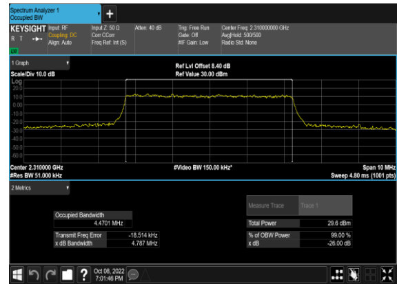
N30(5M)_DFT-s-OFDM_QPSK_Outer_Full_Mid_C
