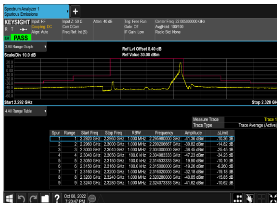
N30(10M)_DFT-s-OFDM_BPSK_Edge_1RB_Right_
