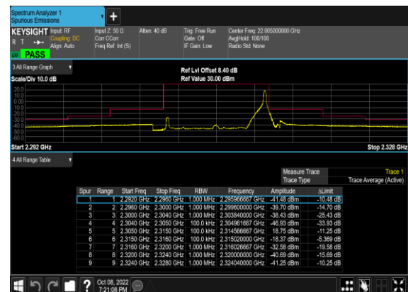
N30(10M)_DFT-s-OFDM_QPSK_Edge_1RB_Right_
