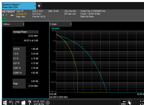
N30(5M)_DFT-s-OFDM_PI_2-BPSK_Outer_Full_ Mid_CH
