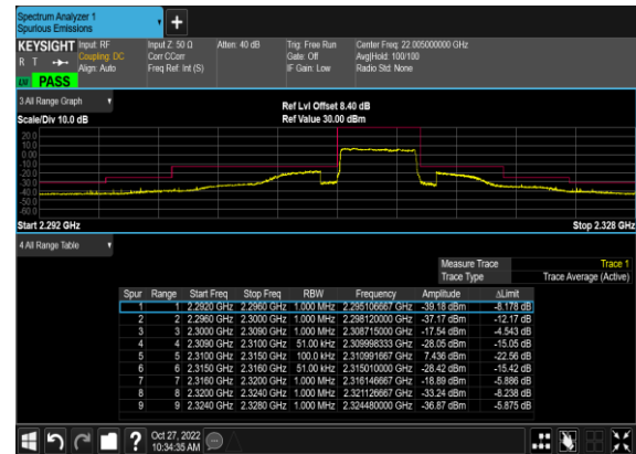
N30(10M)_DFT-s-OFDM_QPSK_Edge_1RB_Left_L
