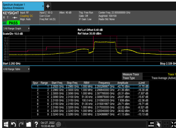
N30(10M)_DFT-s-OFDM_BPSK_Edge_1RB_Left_L
