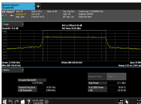
N30(10M)_CP-OFDM_64 QAM_Outer_Full_Low_CH
