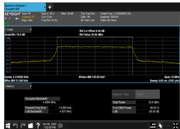
N30(5M)_CP-OFDM_256 QAM_Outer_Full_Mid_CH
