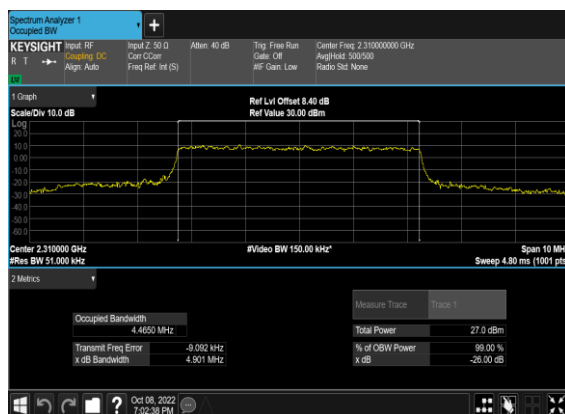
N30(5M)_CP-OFDM_64 QAM_Outer_Full_Mid_CH
