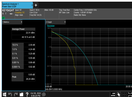
N30(5M)_DFT-s-OFDM_QPSK_Outer_Full_Low_ CH
