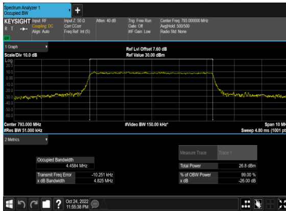
N14(5M)_CP- OFDM_QPSK_Outer_Full_Mid_CH
