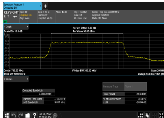
N14(10M)_CP-OFDM_256 QAM_Outer_Full_Mid_CH
