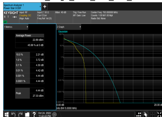
N14(5M)_DFT-s-OFDM_PI_2-BPSK_Edge_1RB_Left_Mid_CH
