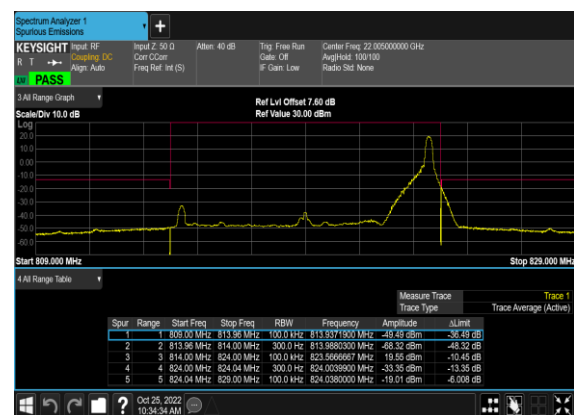
N26(10M)_DFT-s-OFDM_QPSK_Edge_1RB_Right_Mid_CH
