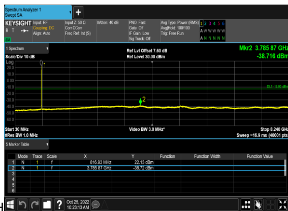
N26(5M)_DFT-s-OFDM_BPSK_Edge_1RB_Left_Mid
