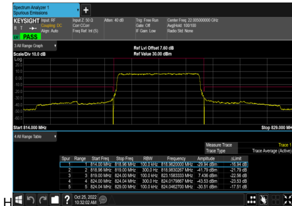
N26(5M)_DFT-s-OFDM_BPSK_Outer_Full_High_C
