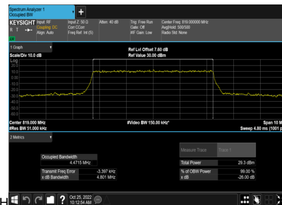
N26(5M)_DFT-s-OFDM_QPSK_Outer_Full_Mid_C
