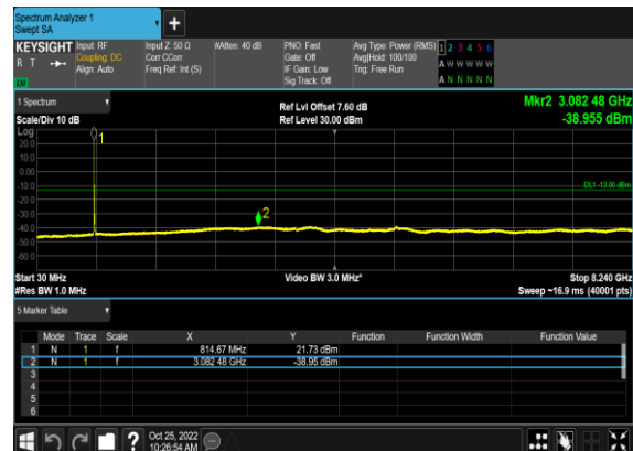
N26(10M)_DFT-s-OFDM_QPSK_Edge_1RB_Left_Mi d_CH
