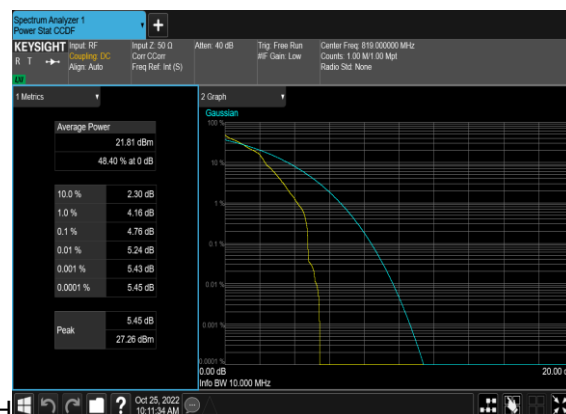
N26(10M)_DFT-s-OFDM_QPSK_Edge_1RB_Left_Mid_ _CH
