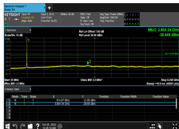
N26(20M)_DFT-s-OFDM_QPSK_Edge_1RB_Left_Mi d_CH
