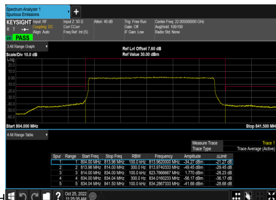
N26(20M)_DFT-s-OFDM_BPSK_Outer_Full_Low_C
