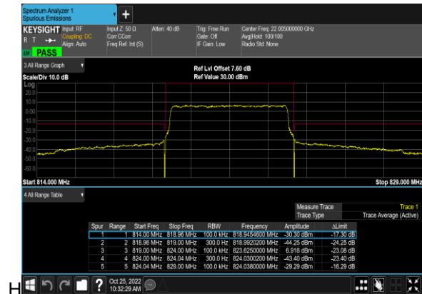
N26(5M)_DFT-s-OFDM_QPSK_Outer_Full_High_C
