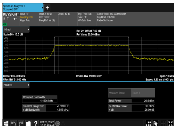
N26(5M)_CP-OFDM_64 QAM_Outer_Full_Mid_CH
