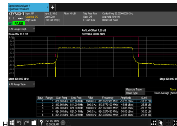
N26(10M)_DFT-s-OFDM_QPSK_Outer_Full_Mid_C
