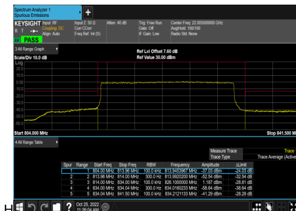
N26(20M)_DFT-s-OFDM_QPSK_Outer_Full_Low_C
