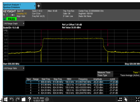
N26(10M)_DFT-s-OFDM_BPSK_Outer_Full_Mid_C
