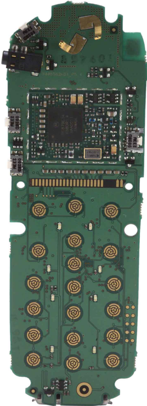
Front View (Shields Removed)
