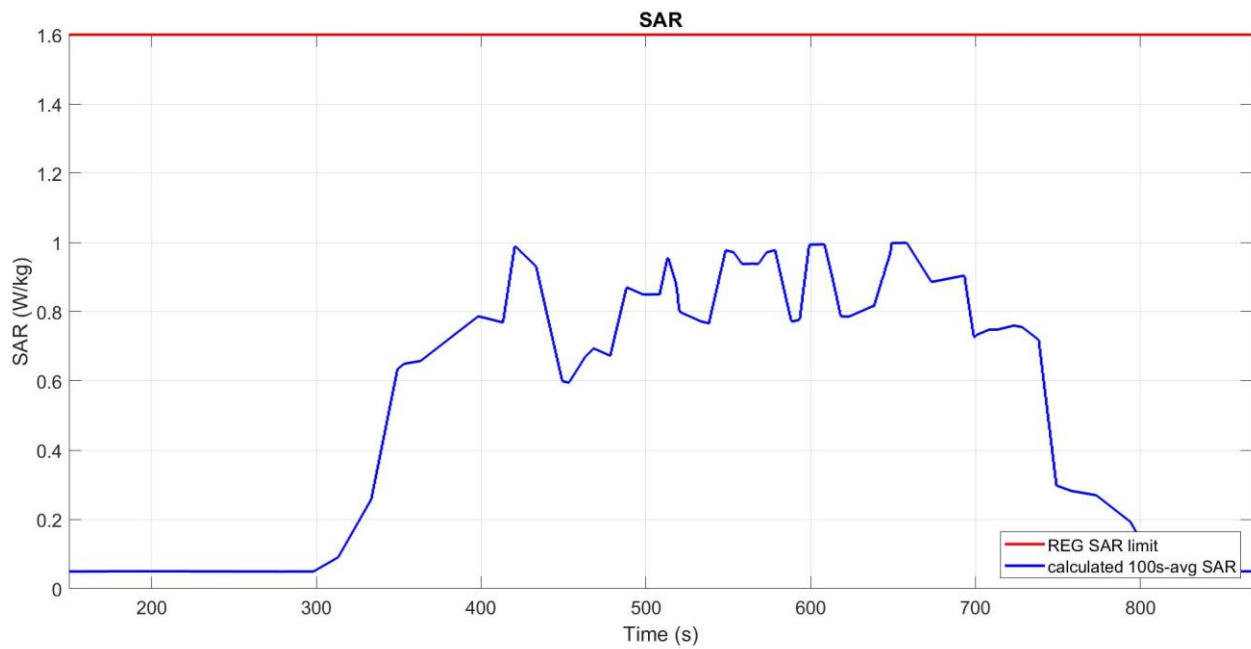
Figure 6-18 Time-averaged SAR
