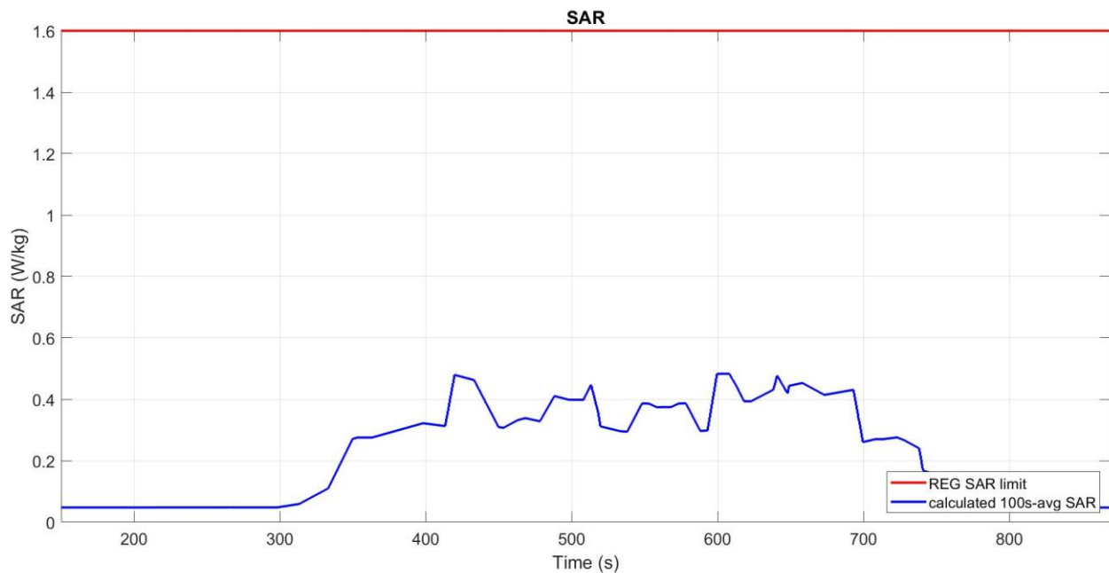
Figure 6-6 Time-averaged SAR for case
