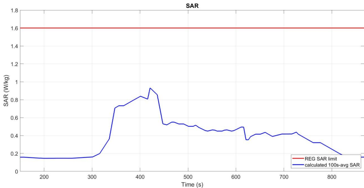
Figure 6-12 Time-averaged SAR
