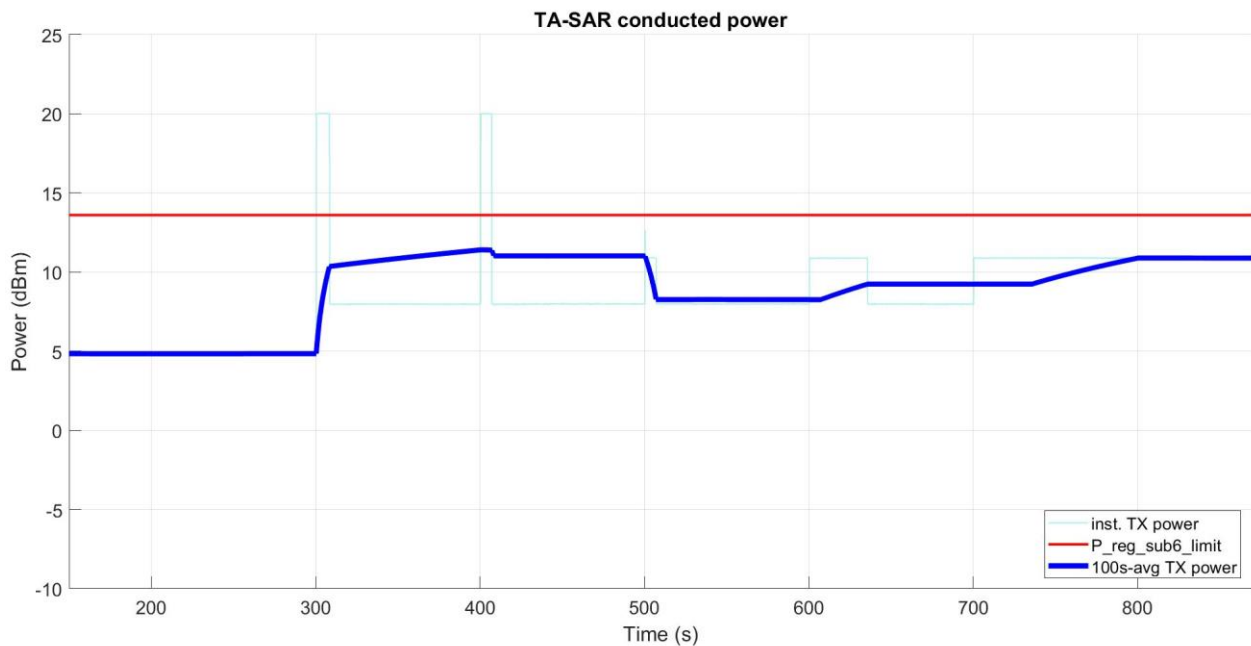
Figure 5- 29 Time-averaged conducted TX power over time
