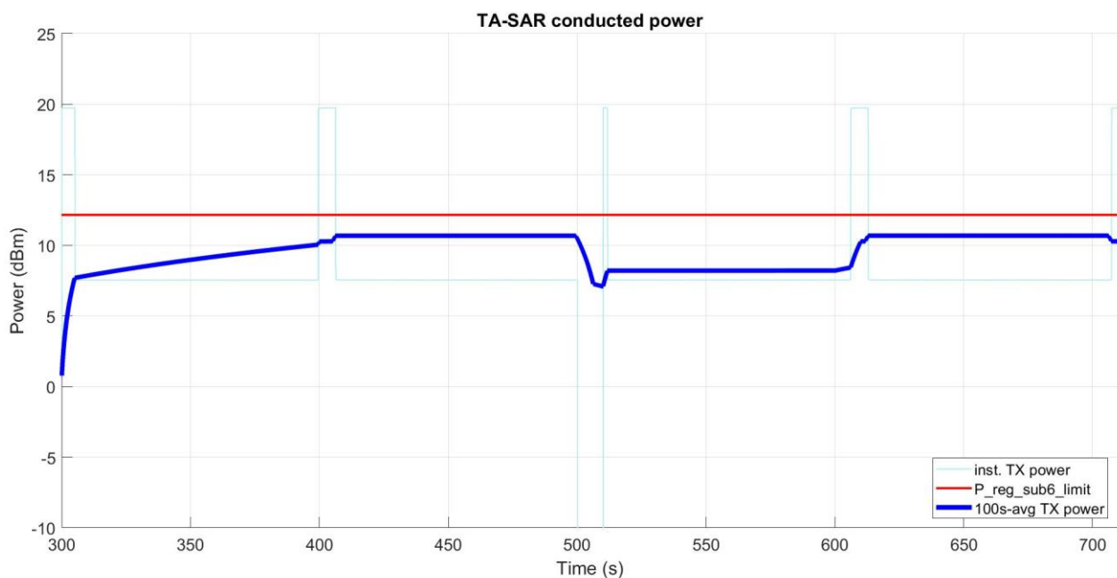
Figure 5- 42 Time-averaged conducted TX power over time
