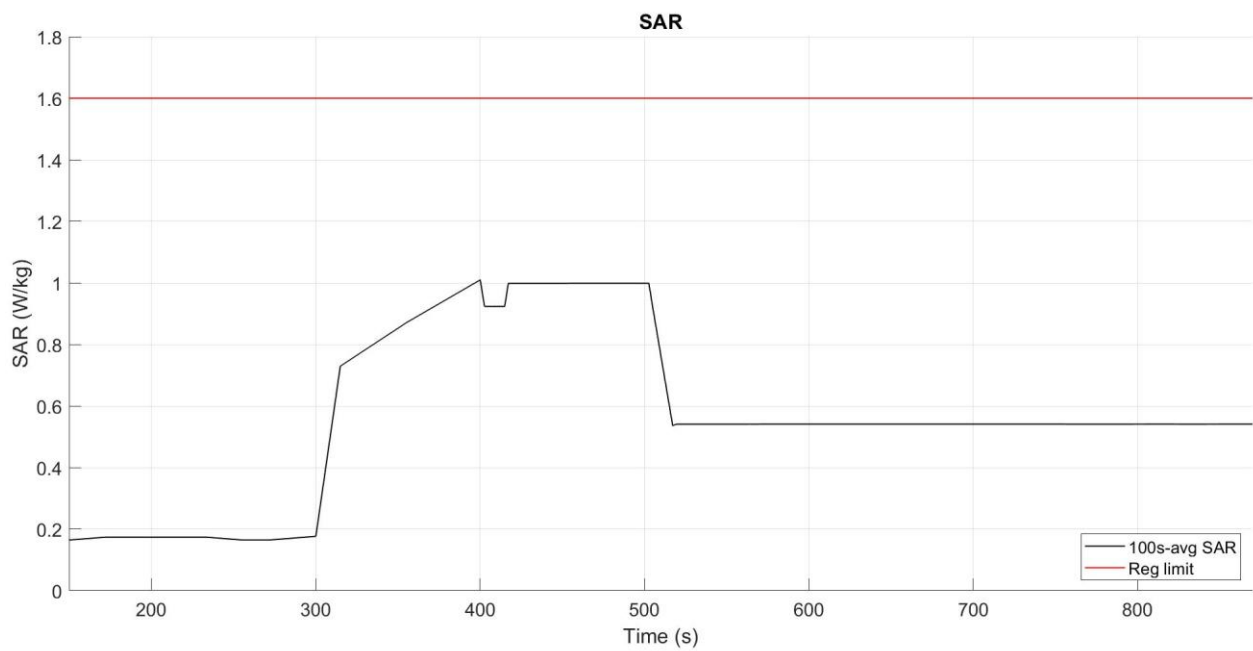
Figure 6- 16 Time-averaged SAR
