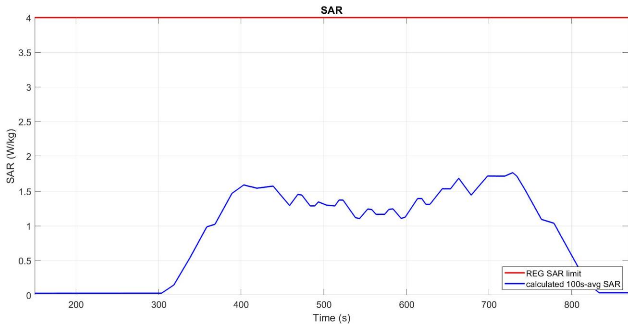
Figure 6-10 Time-averaged SAR
