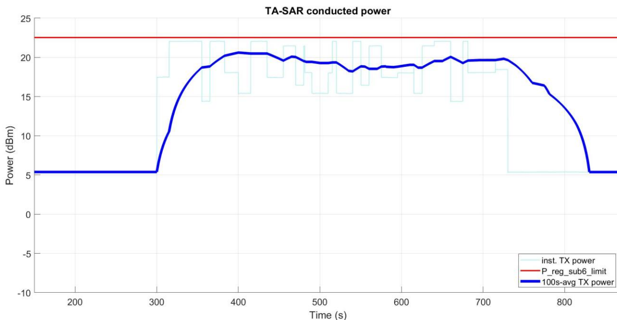
Figure 5- 35 Time-averaged conducted TX power over time
