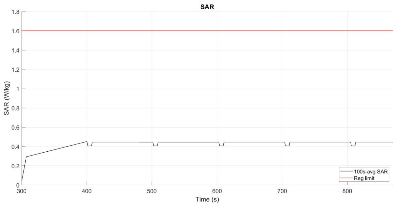
Figure 5- 6 Time-averaged SAR
