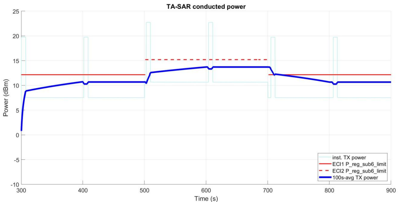
Figure 5- 40 Time-averaged conducted TX power over time
