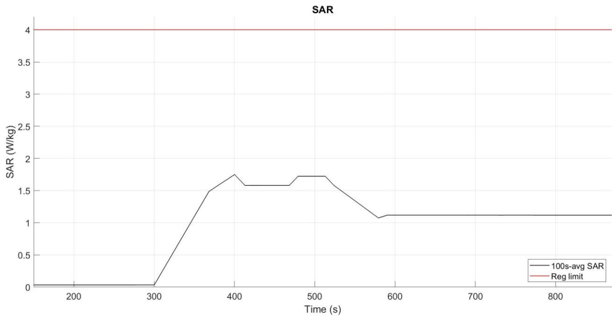
Figure 5- 26 Time-averaged SAR
