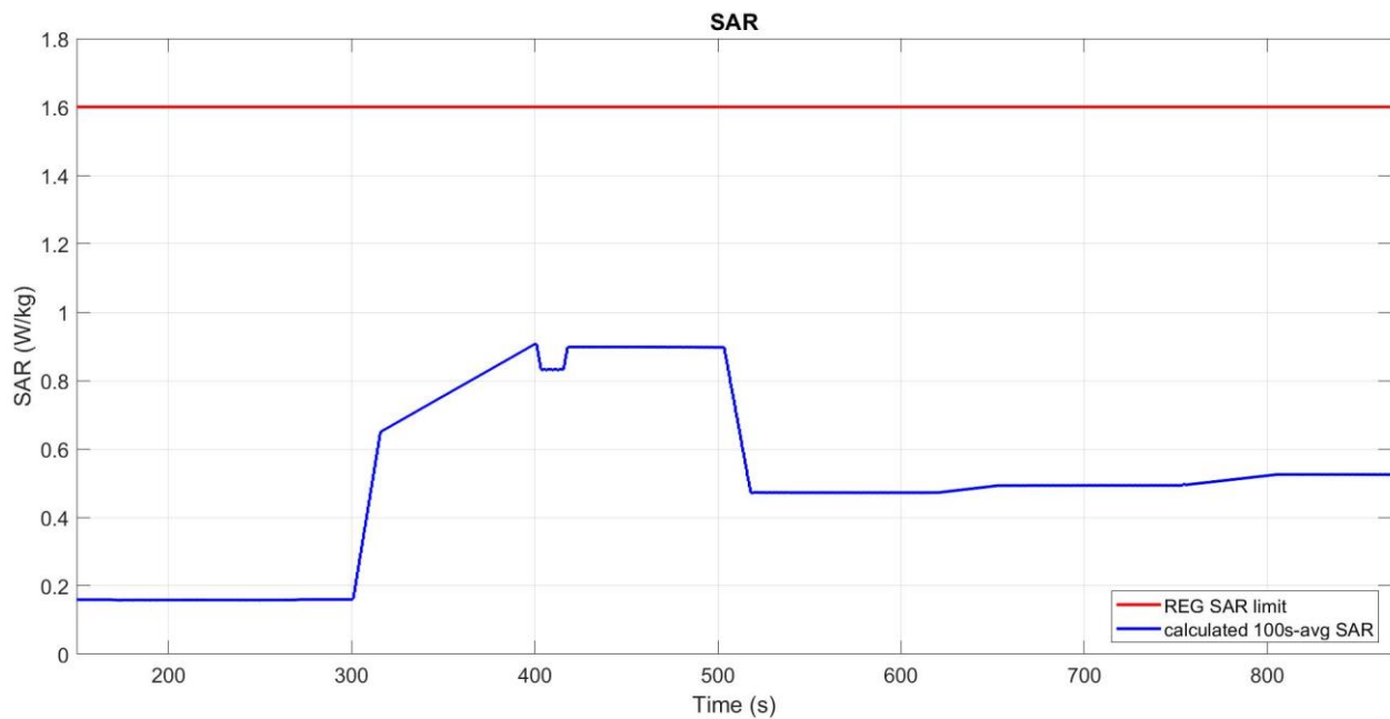
Figure 6-11 Time-averaged SAR
