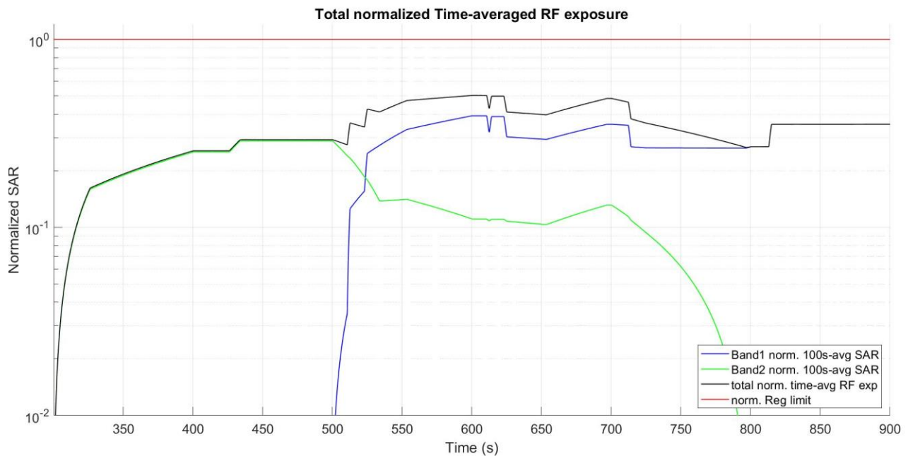
Figure 5- 49 Normalized time-averaged SAR
