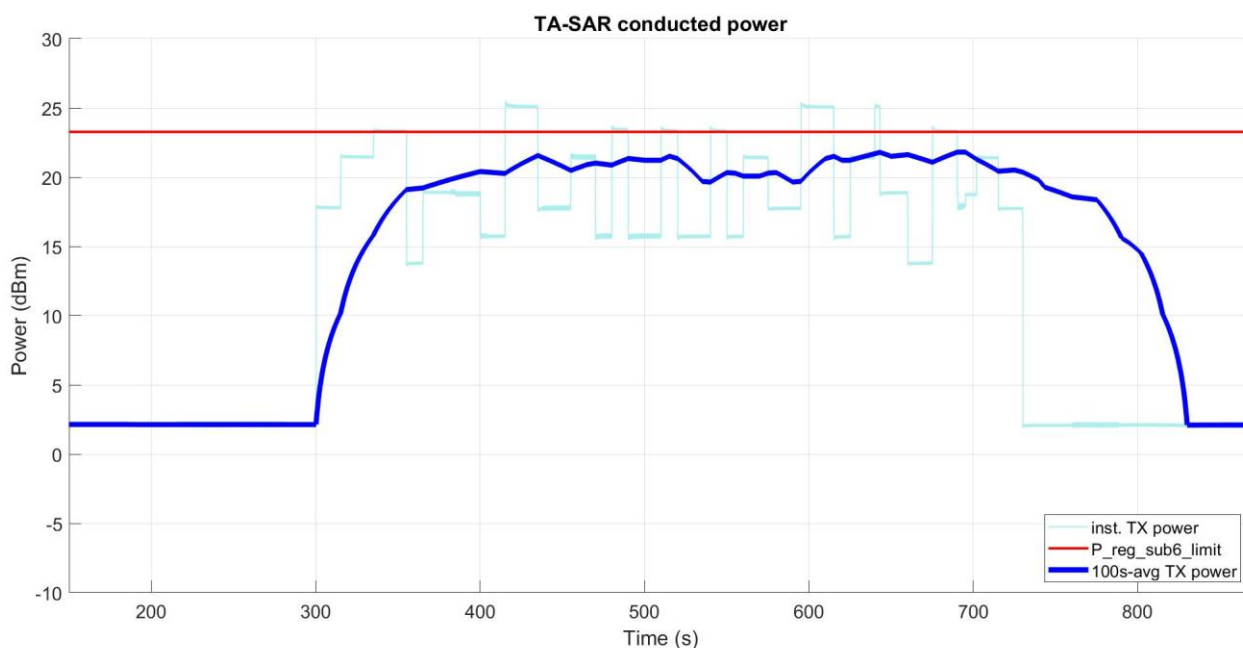
Figure 5- 9 Time-averaged conducted TX power over time
