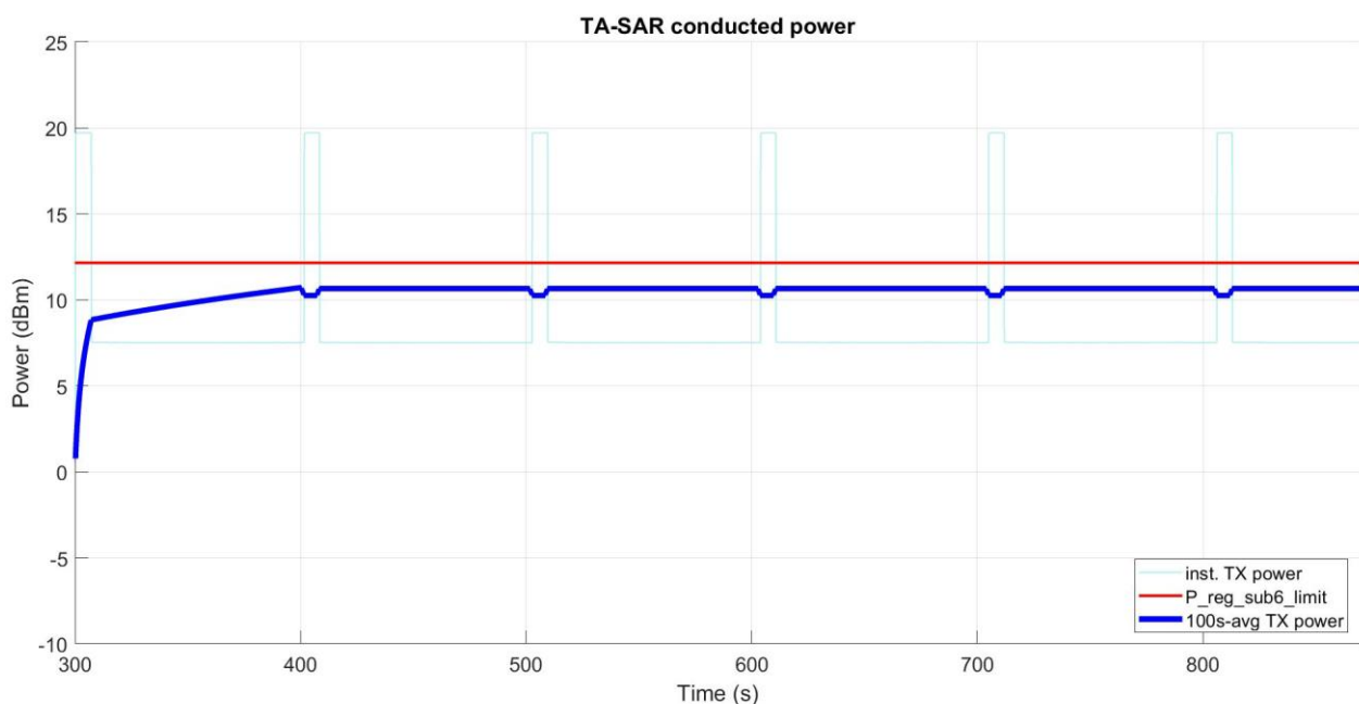
Figure 5- 5 Time-averaged conducted TX power over time
