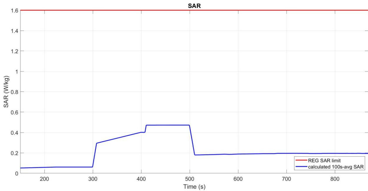
Figure 6-5 Time-averaged SAR
