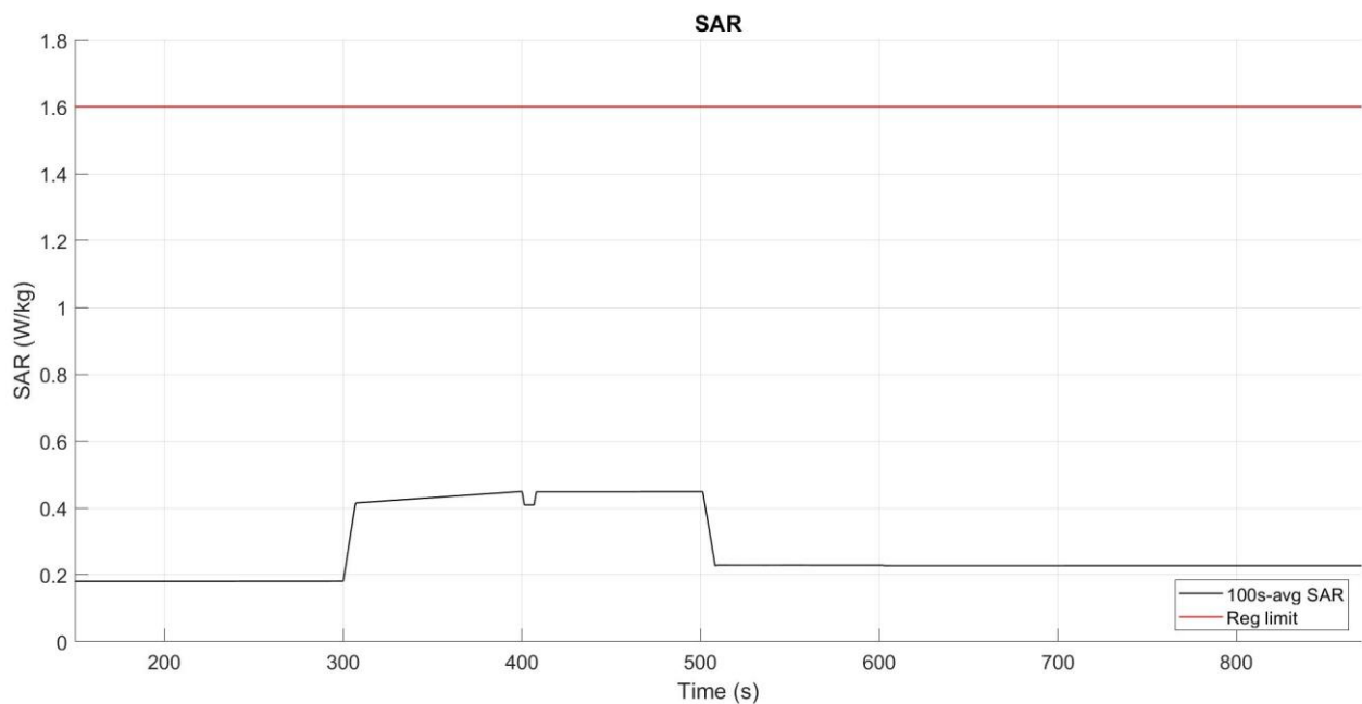
Figure 5- 23 Time-averaged SAR
