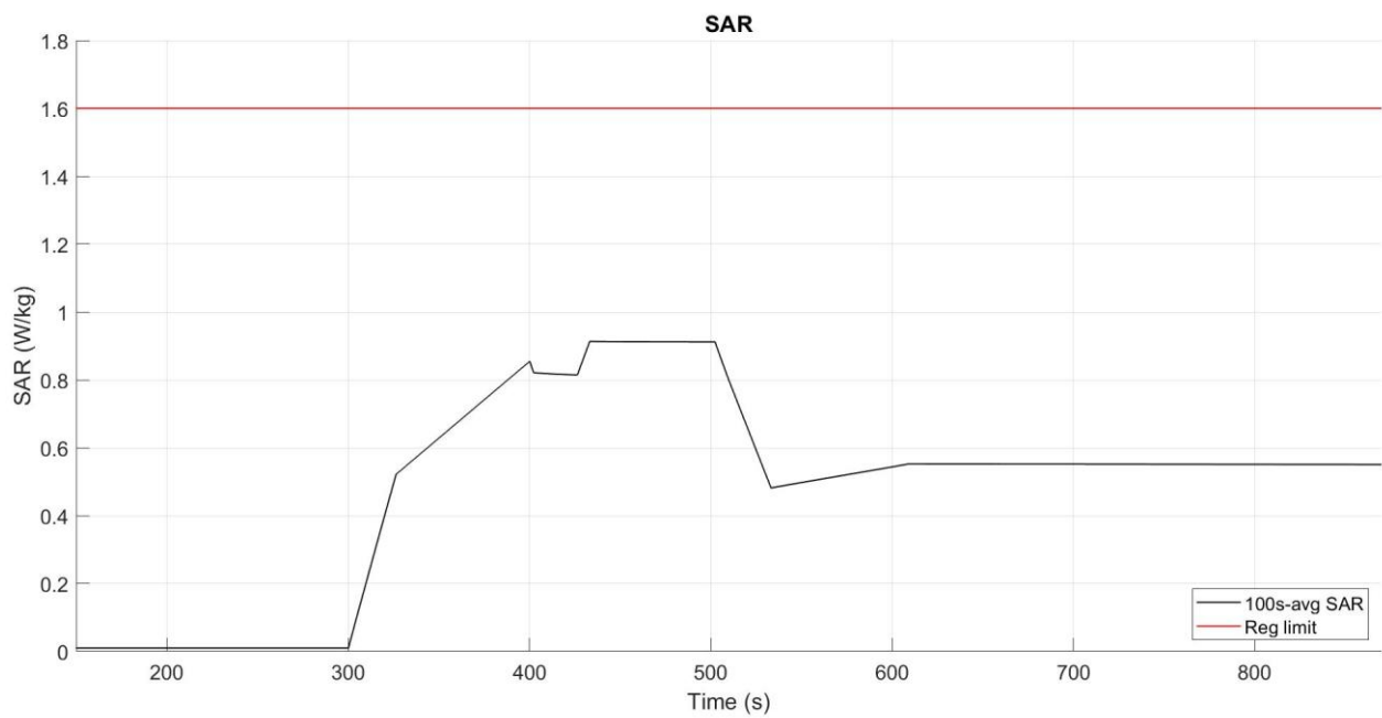
Figure 5- 8 Time-averaged SAR
