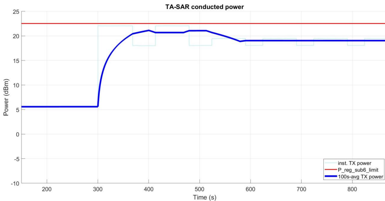
Figure 5- 33 Time-averaged conducted TX power over time
