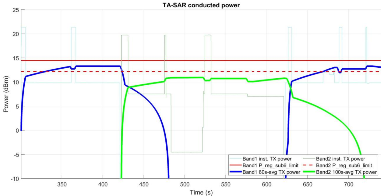
Figure 5- 42 Time-averaged conducted TX power over time
