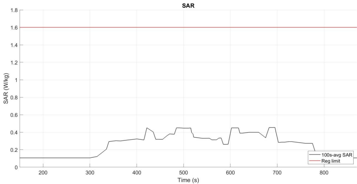
Figure 5- 32 Time-averaged SAR
