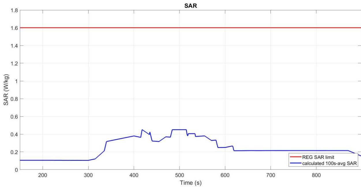
Figure 6-8 Time-averaged SAR
