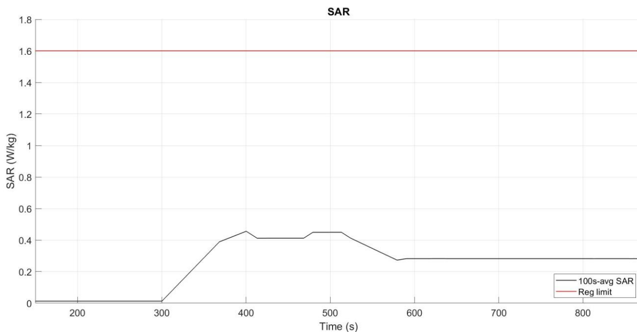
Figure 5- 34 Time-averaged SAR
