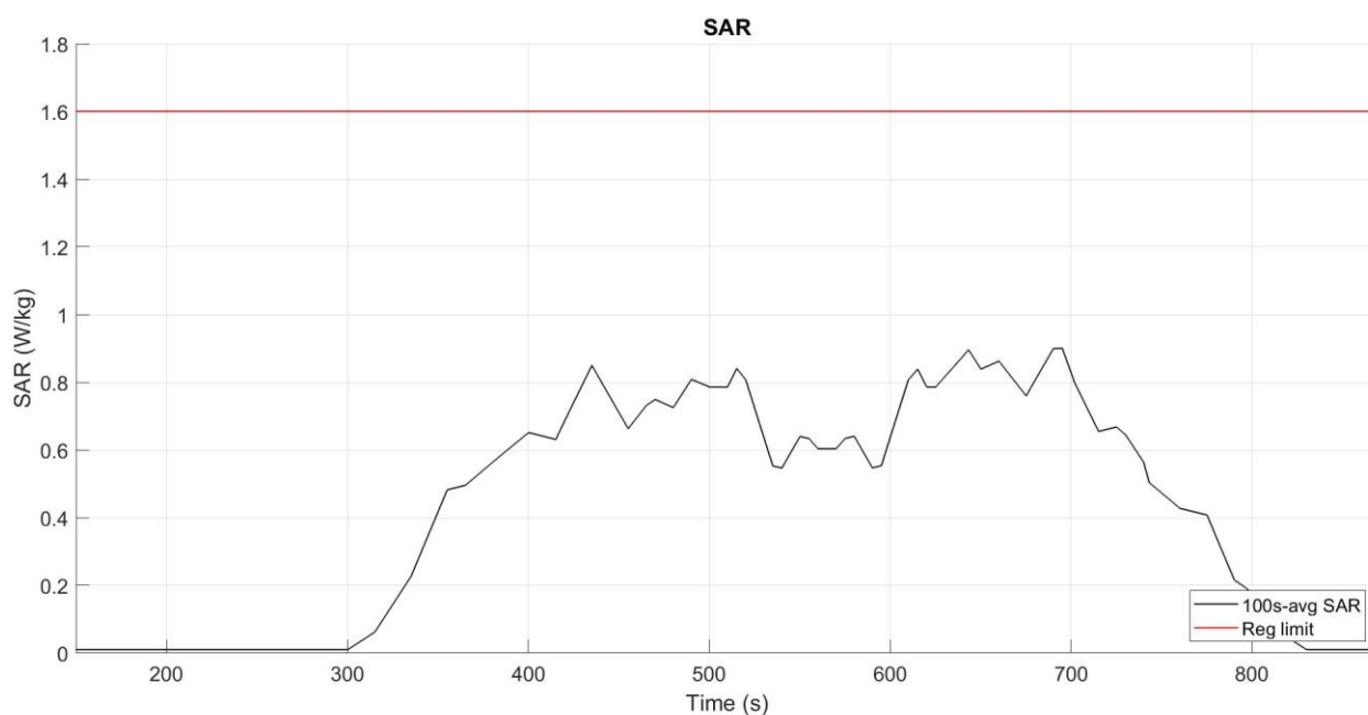
Figure 5- 10 Time-averaged SAR
