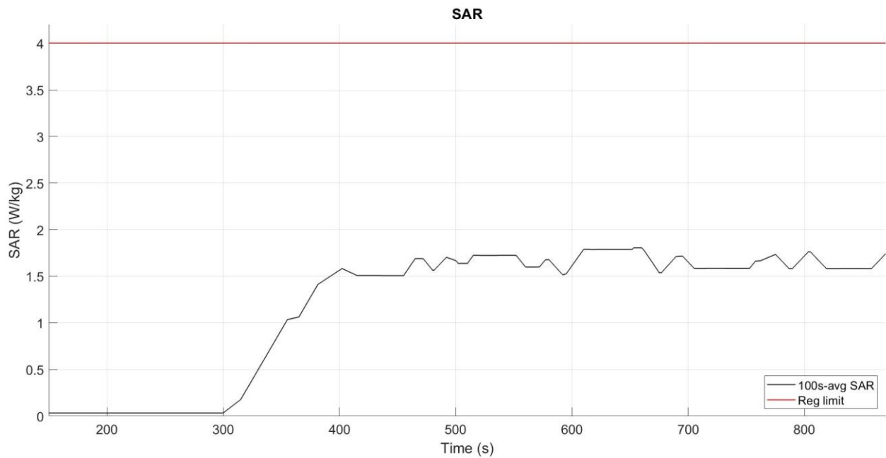
Figure 5- 28 Time-averaged SAR
