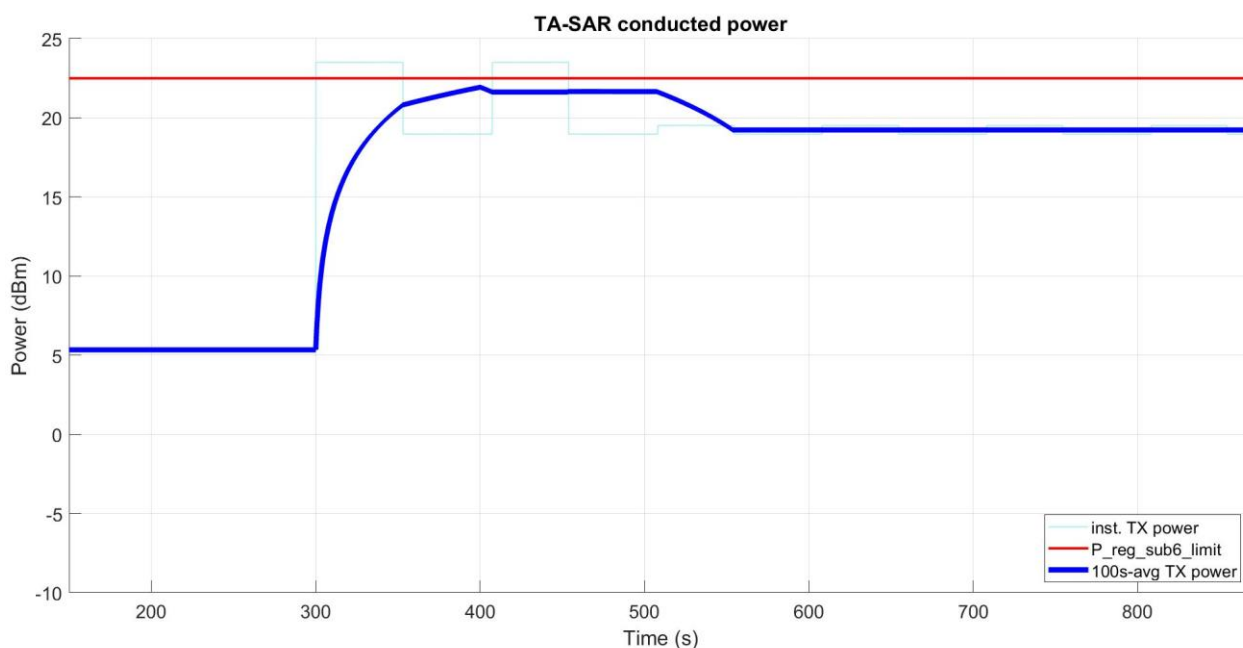
Figure 5- 18 Time-averaged conducted TX power over time
