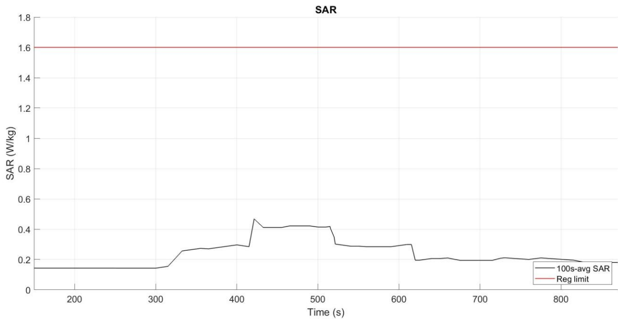
Figure 5- 24 Time-averaged SAR
