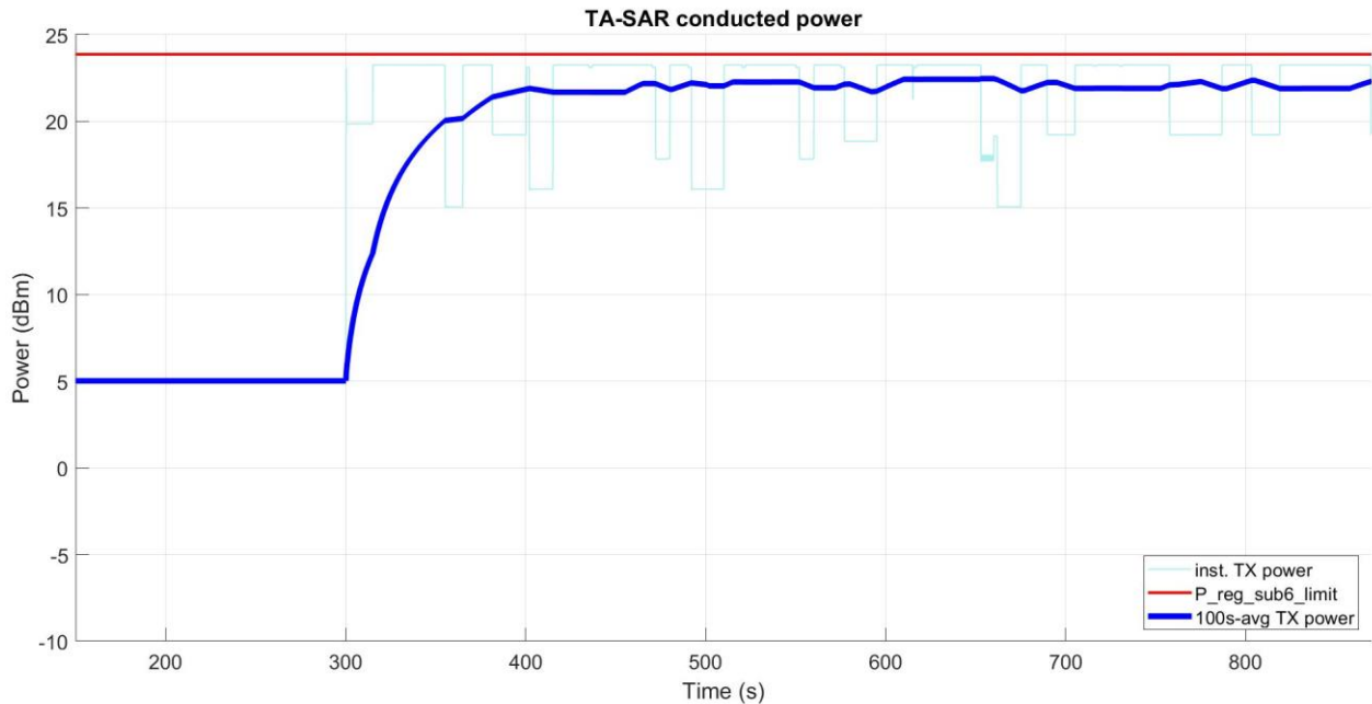
Figure 5- 27 Time-averaged conducted TX power over time
