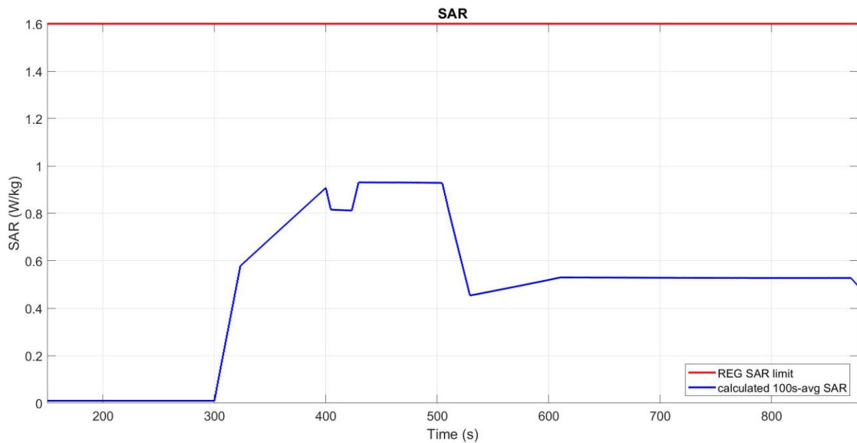
Figure Time-averaged SAR
