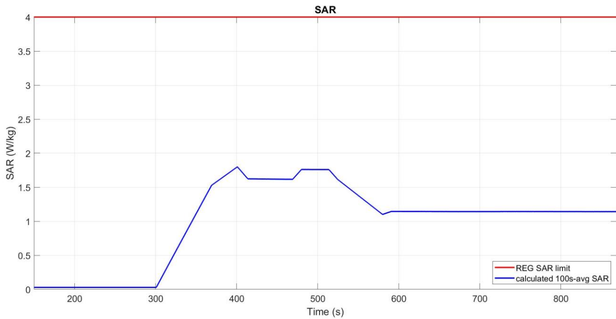
Figure 6-9 Time-averaged SAR
