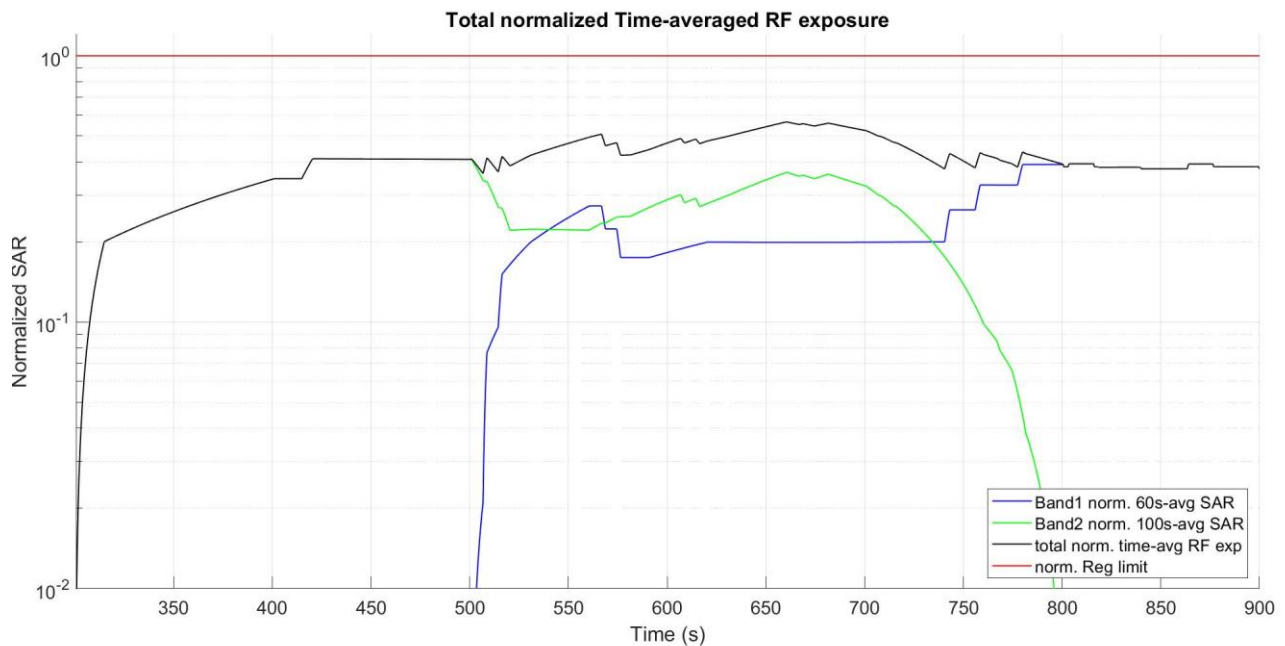
Figure 5- 47 Normalized time-averaged SAR
