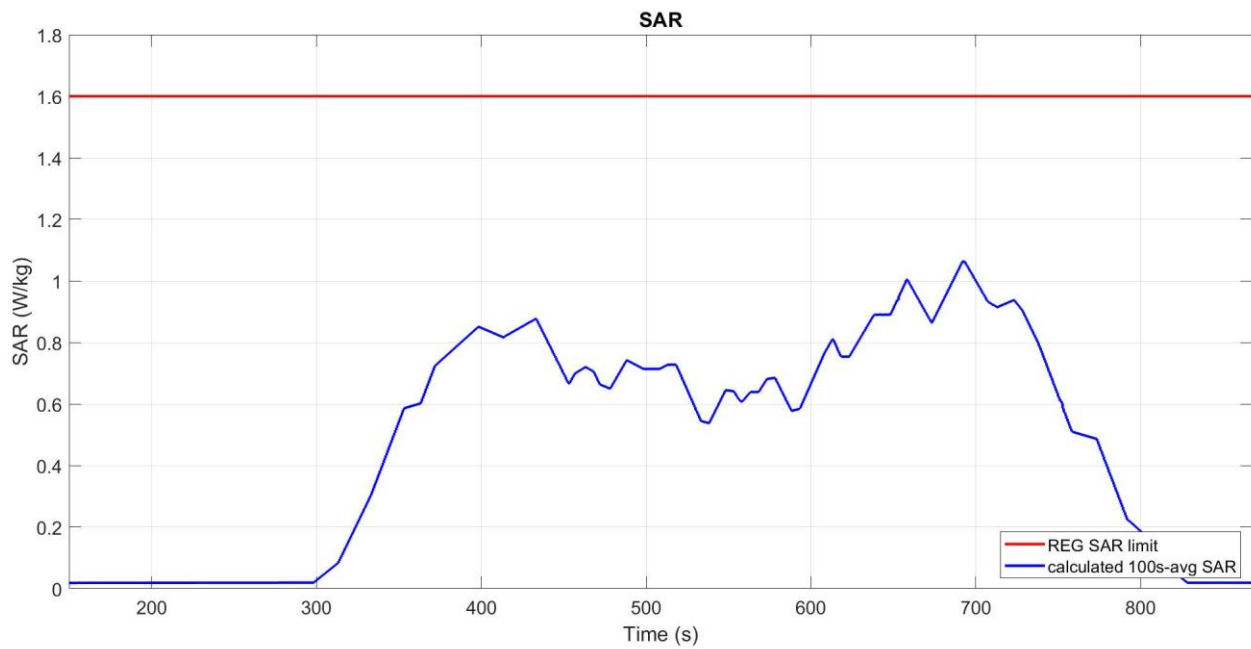
Figure 6-14 Time-averaged SAR
