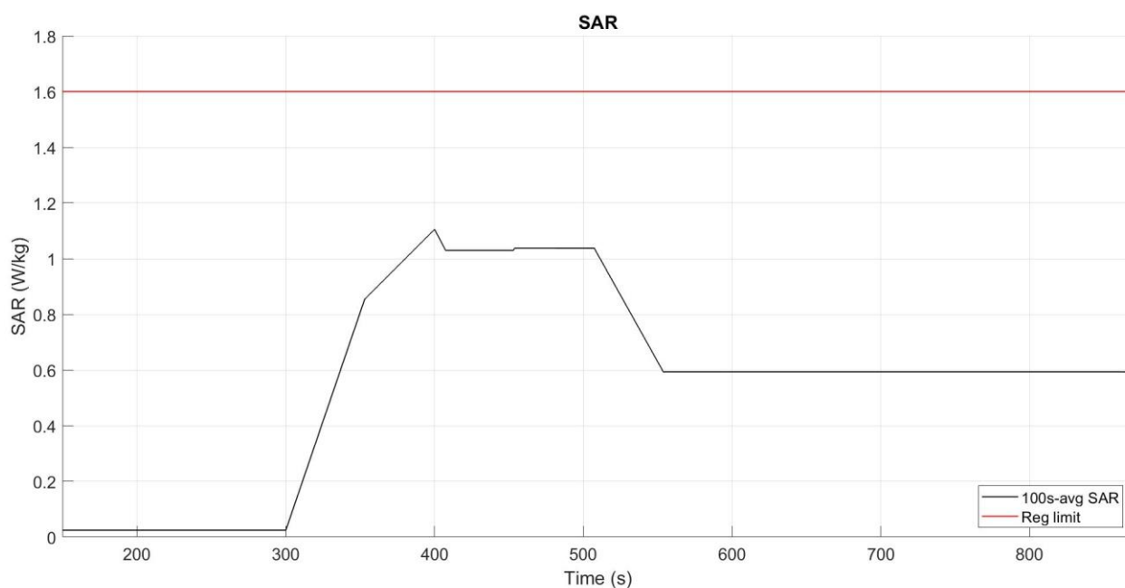
Figure 5- 19 Time-averaged SAR
