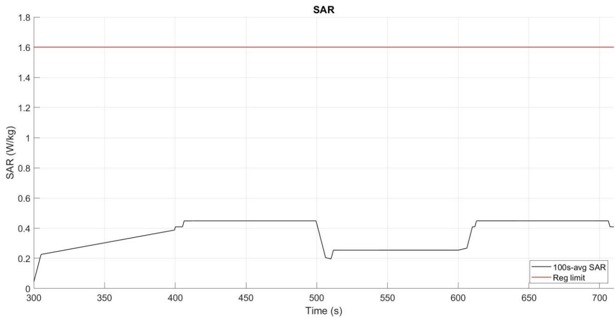
Figure 5- 37 Time-averaged SAR
