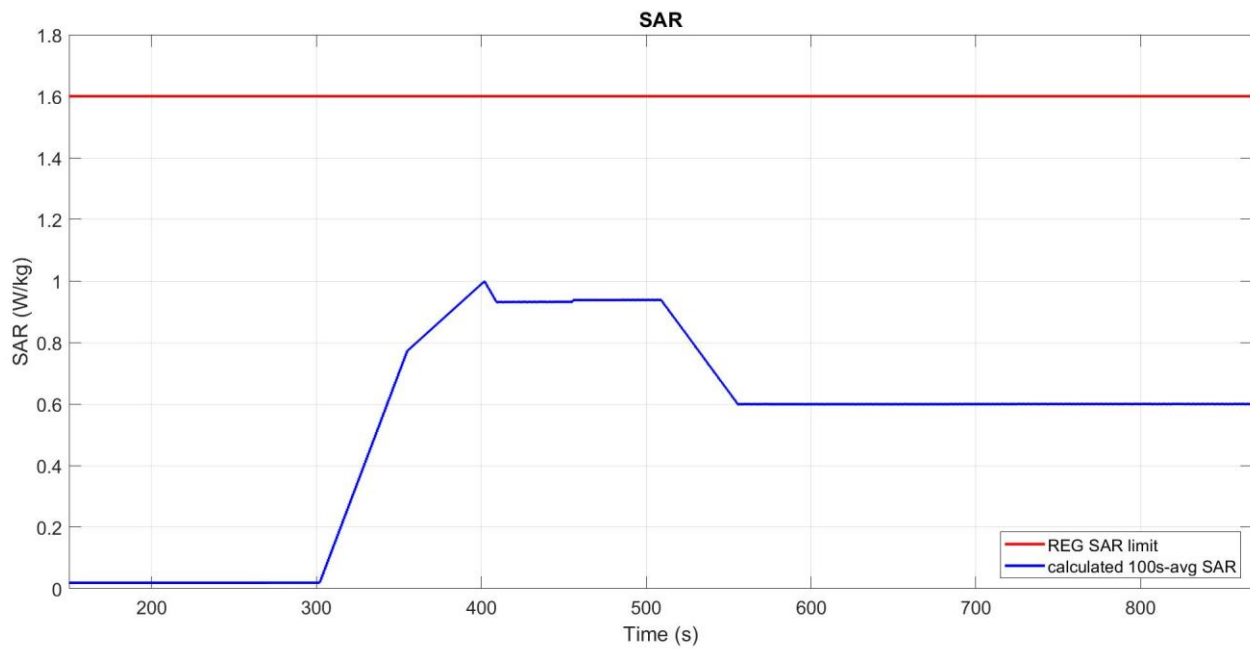
Figure 6-13 Time-averaged SAR
