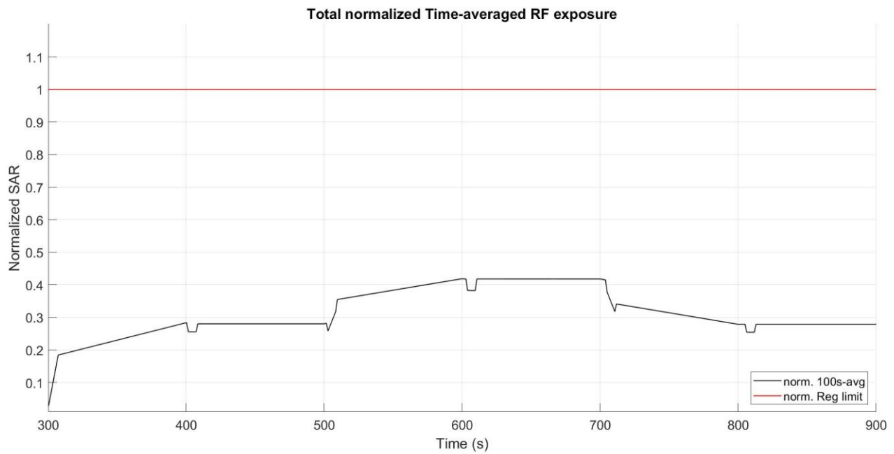
Figure 5- 41 Normalized time-averaged SAR
