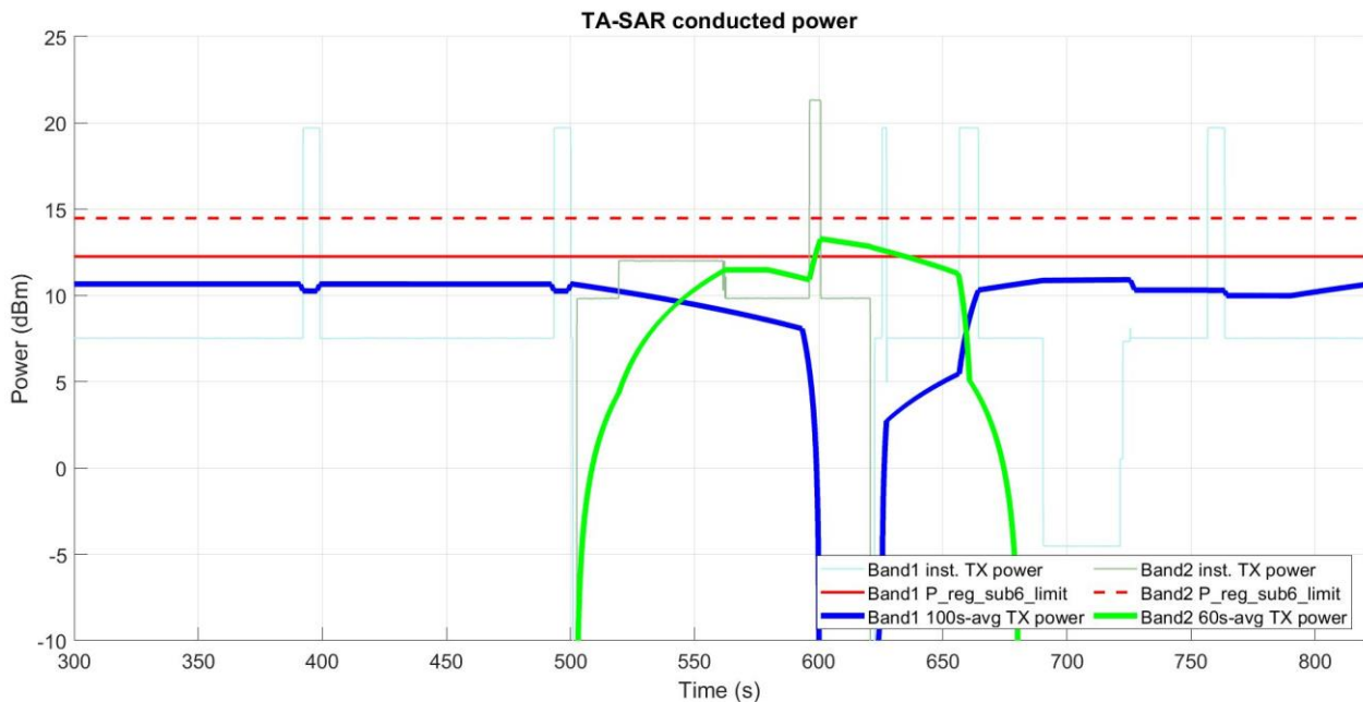
Figure 5- 44 Time-averaged conducted TX power over time
