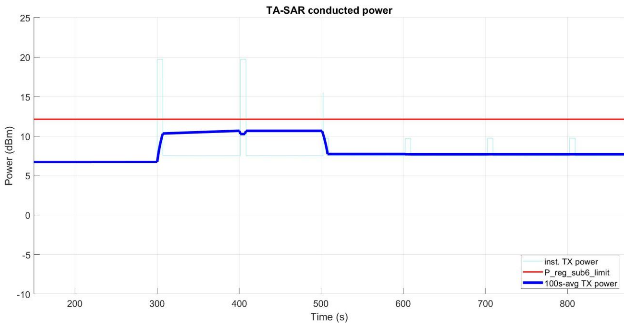
Figure 5- 22 Time-averaged conducted TX power over time
