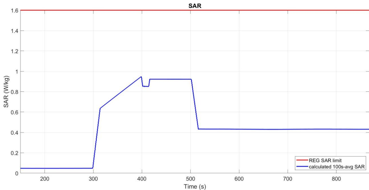
Figure 6-17 Time-averaged SAR
