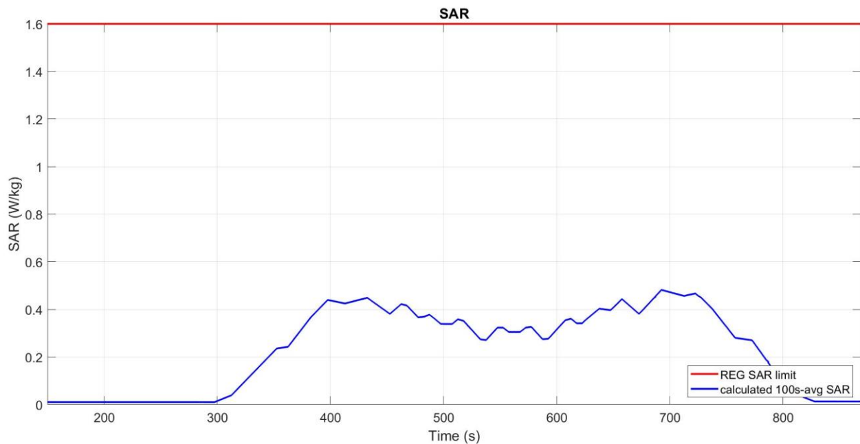
Figure 6-4 Time-averaged SAR
