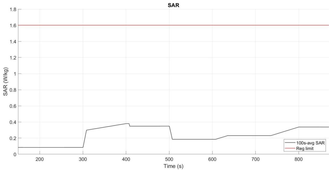
Figure 5- 30 Time-averaged SAR
