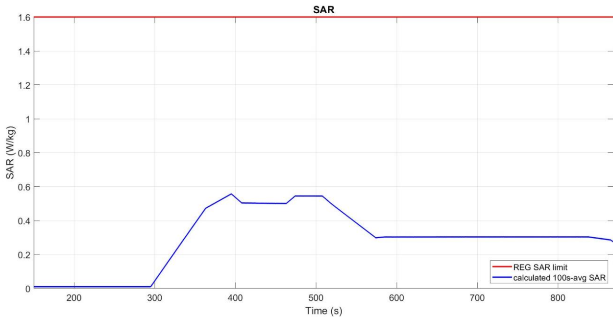
Figure 6-3 Time-averaged SAR
