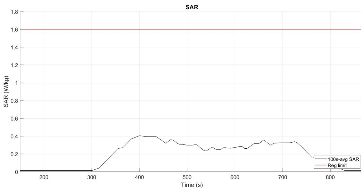
Figure 5- 36 Time-averaged SAR
