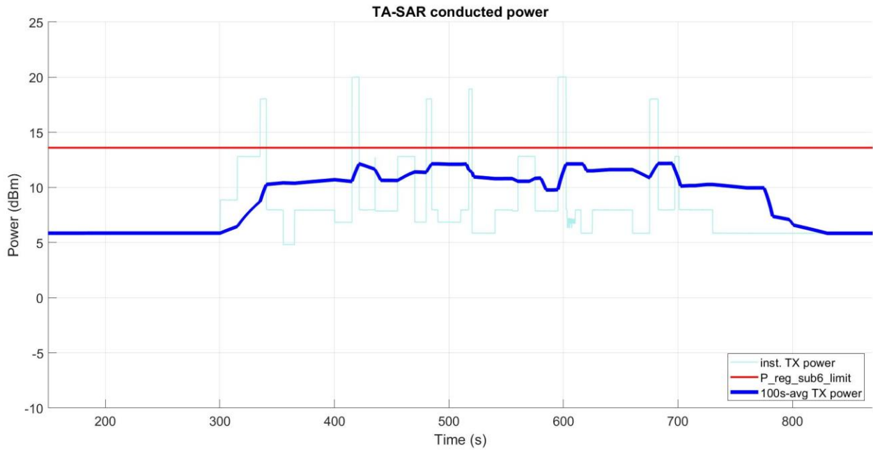
Figure 5- 31 Time-averaged conducted TX power over time
