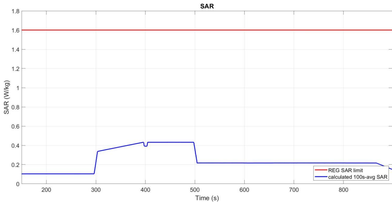
Figure 6-7 Time-averaged SAR
