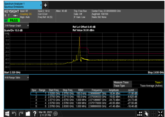
N7(5M)_DFT-s- OFDM_QPSK_Edge_1RB_Right_High_CH
