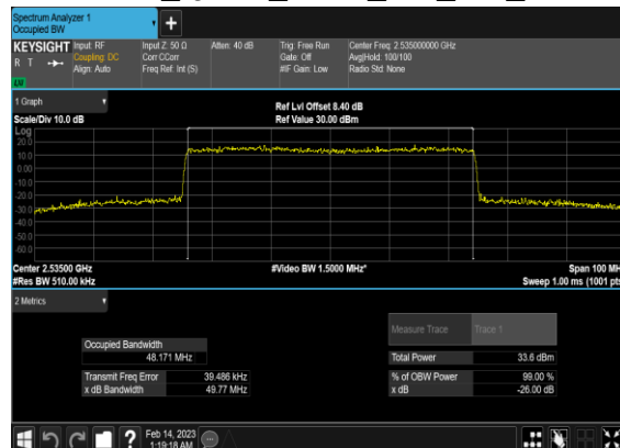
N7(50M)_DFT-s- OFDM_QPSK_Outer_Full_Mid_CH
