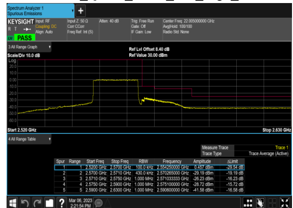
N7(20M)_DFT-s- OFDM_QPSK_Outer_Full_High_CH
