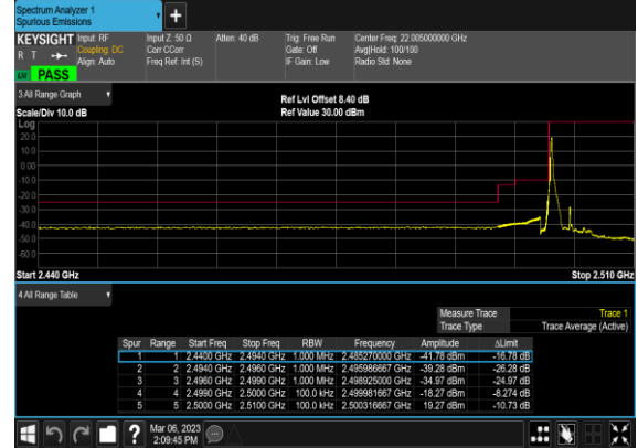
N7(5M)_DFT-s- OFDM_QPSK_Edge_1RB_Left_Low_CH
