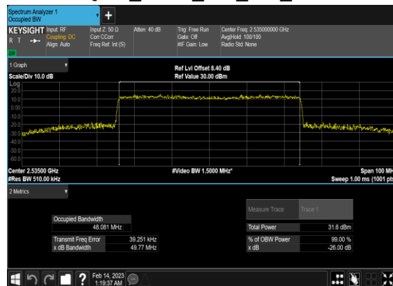
N7(50M)_CP-OFDM_16 QAM_Outer_Full_Mid_CH
