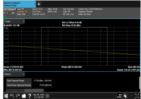
N7(20M)_DFT-s- OFDM_QPSK_Edge_1RB_Right_High_CH_CHP_PASS
