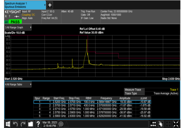
N7(20M)_DFT-s- OFDM_BPSK_Edge_1RB_Right_High_CH
