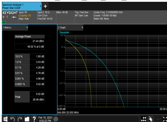
N7(20M)_DFT-s-OFDM_PI_2-BPSK_Outer_Full_Low_CH
