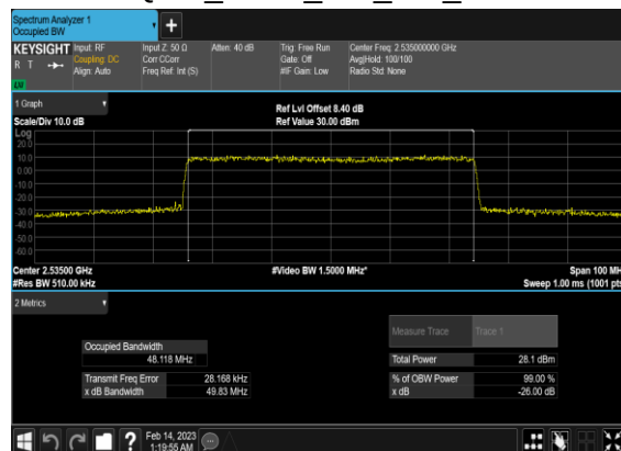
N7(50M)_CP-OFDM_256 QAM_Outer_Full_Mid_CH
