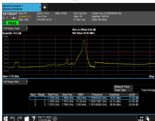
N66(5M)_DFT-s- OFDM_BPSK_Edge_1RB_Right_High_C H
