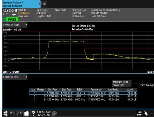
N66(5M)_DFT-s- OFDM_BPSK_Outer_Full_High_CH
