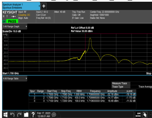
N66(40M)_DFT-s- OFDM_BPSK_Edge_1RB_Left_Low_CH
