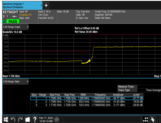
N66(20M)_DFT-s- OFDM_BPSK_Outer_Full_Low_CH
