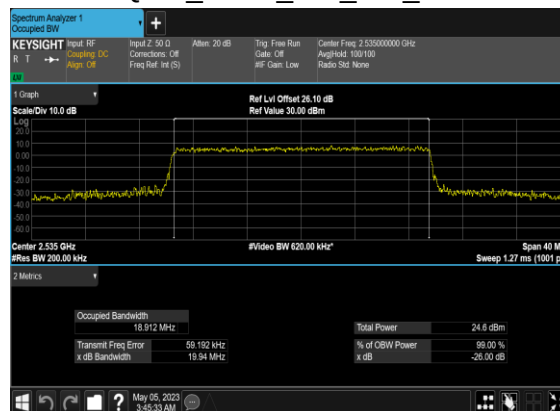
B66_N7(20M)_CP-OFDM_256 QAM_Outer_Full_Mid_CH
