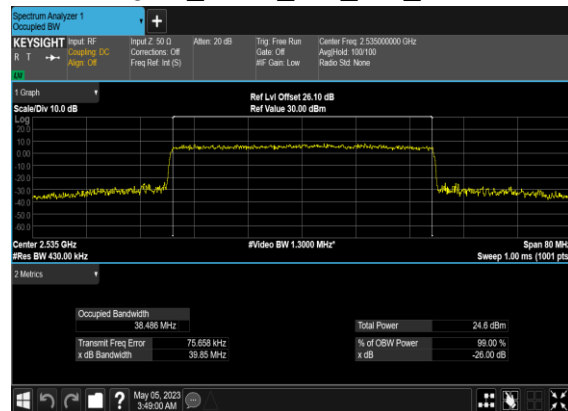
B66_N7(40M)_CP-OFDM_256 QAM_Outer_Full_Mid_CH
