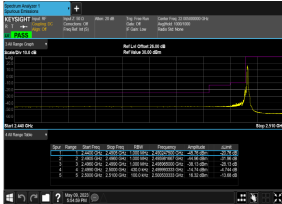
B66_N7(20M)_DFT-s- OFDM_BPSK_Edge_1RB_Left_Low_CH
