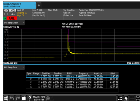
B66_N7(40M)_DFT-s- OFDM_QPSK_Edge_1RB_Right_High_CH
