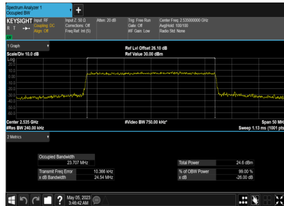
B66_N7(25M)_CP-OFDM_256 QAM_Outer_Full_Mid_CH
