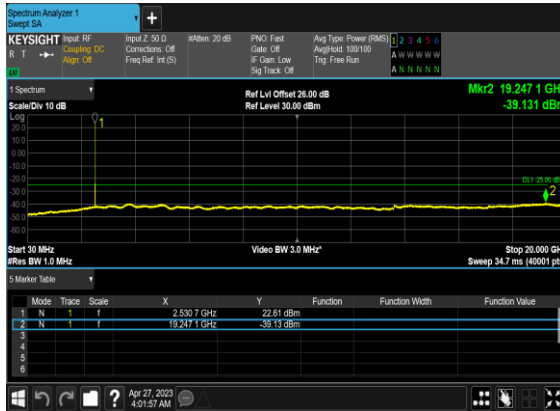
B66_N7(40M)_DFT-s- OFDM_BPSK_Edge_1RB_Left_High_CH
