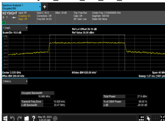
B66_N7(20M)_CP-OFDM_64 QAM_Outer_Full_Mid_CH
