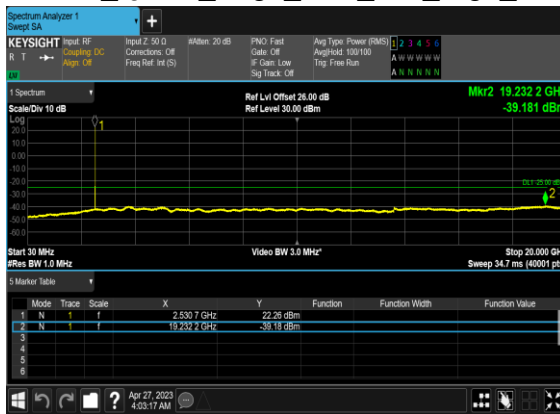
B66_N7(40M)_DFT-s- OFDM_QPSK_Edge_1RB_Left_High_CH
