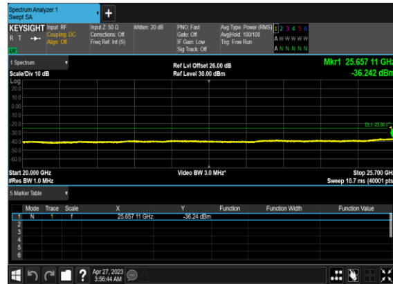
B66_N7(40M)_DFT-s- OFDM_BPSK_Edge_1RB_Left_Low_CH
