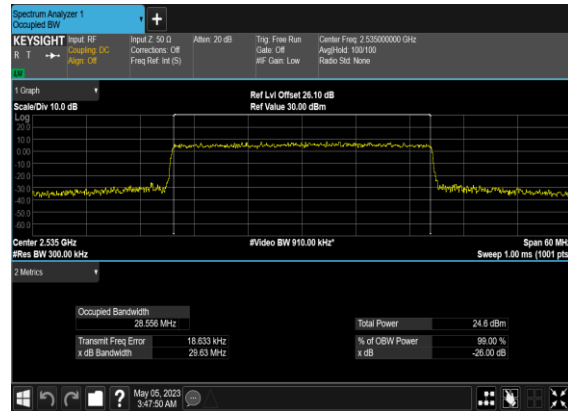
B66_N7(30M)_CP-OFDM_256 QAM_Outer_Full_Mid_CH
