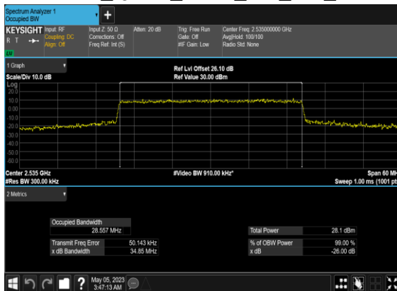
B66_N7(30M)_CP- OFDM_QPSK_Outer_Full_Mid_CH
