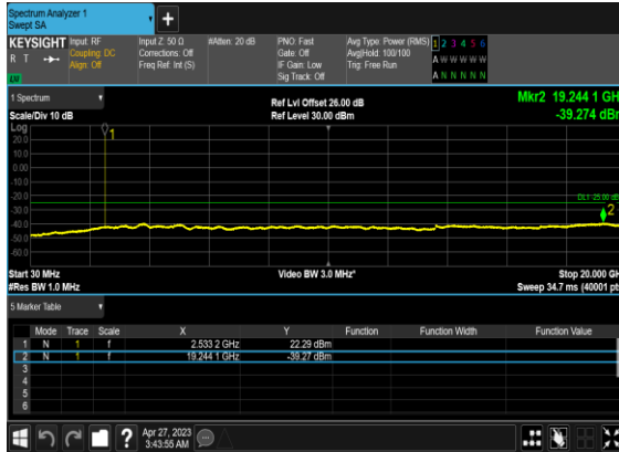
B66_N7(5M)_DFT-s- OFDM_QPSK_Edge_1RB_Left_Mid_CH
