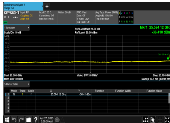
B66_N7(40M)_DFT-s- OFDM_BPSK_Edge_1RB_Left_Mid_CH
