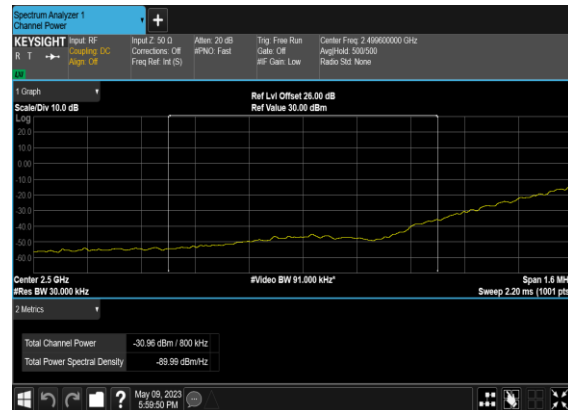
B66_N7(40M)_DFT-s- OFDM_BPSK_Edge_1RB_Left_Low_CH_CHP_ PASS
