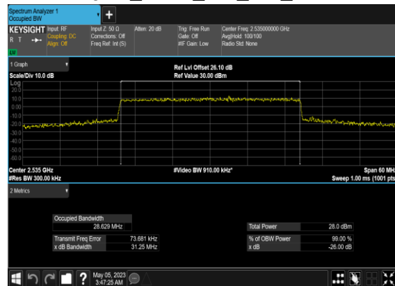
B66_N7(30M)_CP-OFDM_16 QAM_Outer_Full_Mid_CH
