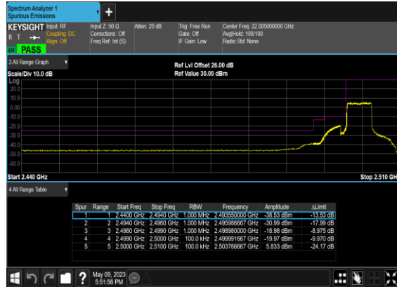
B66_N7(5M)_DFT-s- OFDM_QPSK_Outer_Full_Low_CH
