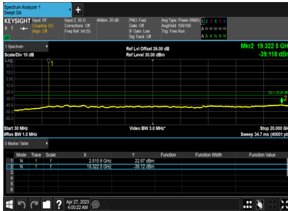
B66_N7(40M)_DFT-s- OFDM_QPSK_Edge_1RB_Left_Mid_CH
