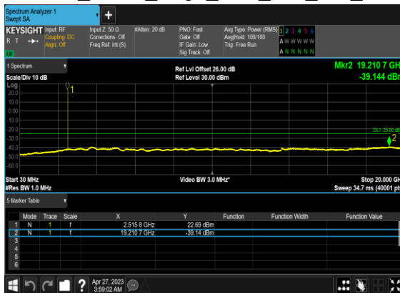
B66_N7(40M)_DFT-s- OFDM_BPSK_Edge_1RB_Left_Mid_CH
