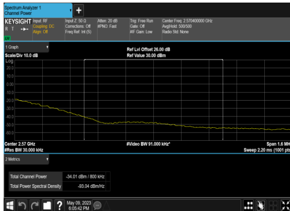
B66_N7(40M)_DFT-s- OFDM_BPSK_Edge_1RB_Right_High_CH_CHP_ PASS
