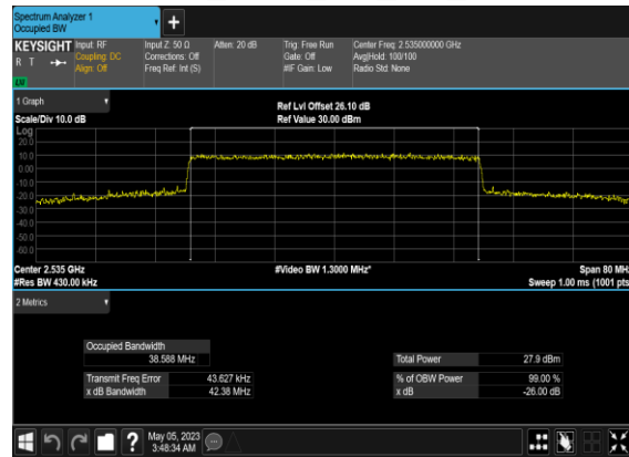
B66_N7(40M)_CP-OFDM_16 QAM_Outer_Full_Mid_CH
