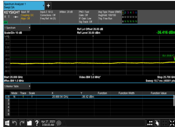
B66_N7(40M)_DFT-s- OFDM_QPSK_Edge_1RB_Left_Low_CH
