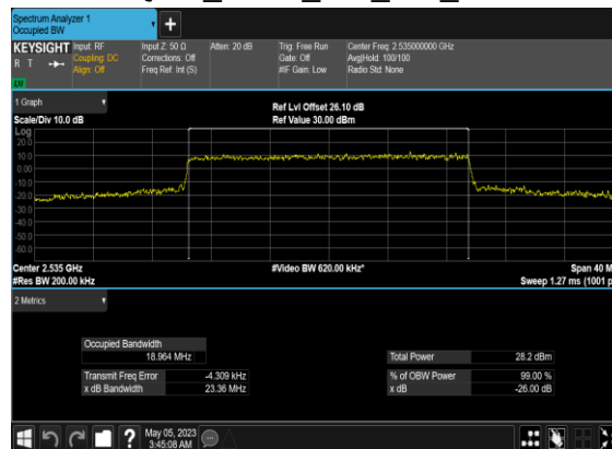
B66_N7(20M)_CP-OFDM_16 QAM_Outer_Full_Mid_CH
