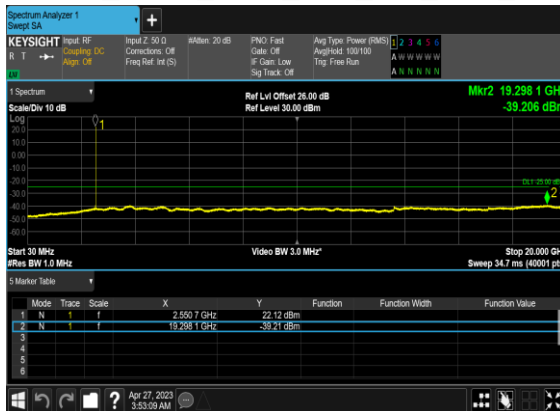
B66_N7(20M)_DFT-s- OFDM_BPSK_Edge_1RB_Left_High_CH
