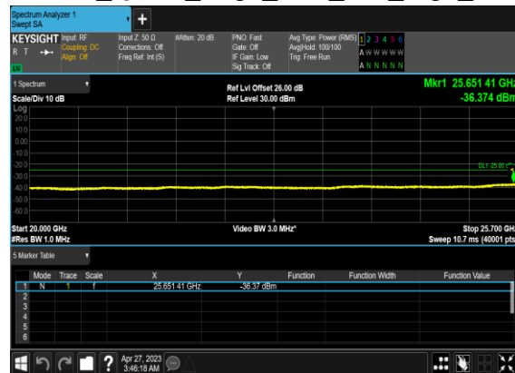
B66_N7(5M)_DFT-s- OFDM_QPSK_Edge_1RB_Left_High_CH
