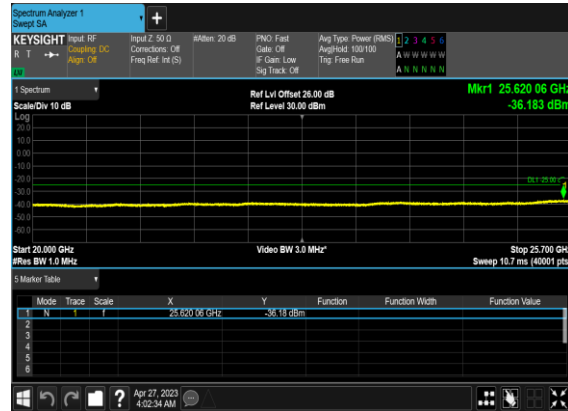
B66_N7(40M)_DFT-s- OFDM_BPSK_Edge_1RB_Left_High_CH
