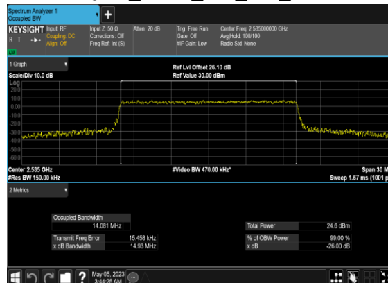
B66_N7(15M)_CP-OFDM_256 QAM_Outer_Full_Mid_CH
