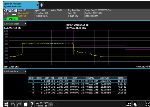
B66_N7(40M)_DFT-s- OFDM_BPSK_Outer_Full_High_CH
