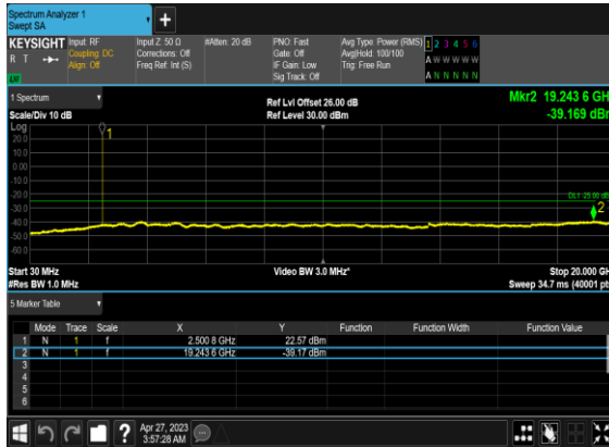
B66_N7(40M)_DFT-s- OFDM_QPSK_Edge_1RB_Left_Low_CH
