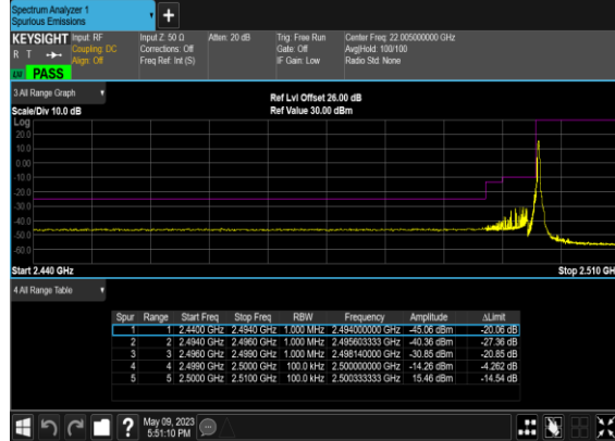
B66_N7(5M)_DFT-s- OFDM_QPSK_Edge_1RB_Left_Low_CH
