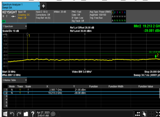
B66_N7(5M)_DFT-s- OFDM_QPSK_Edge_1RB_Left_High_CH
