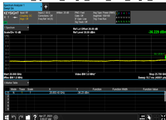
B66_N7(20M)_DFT-s- OFDM_QPSK_Edge_1RB_Left_High_CH
