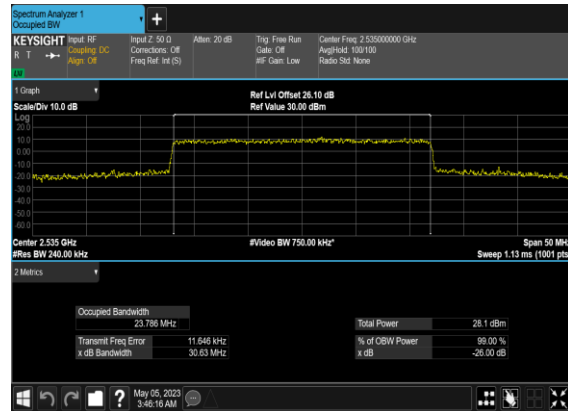
B66_N7(25M)_CP-OFDM_16 QAM_Outer_Full_Mid_CH
