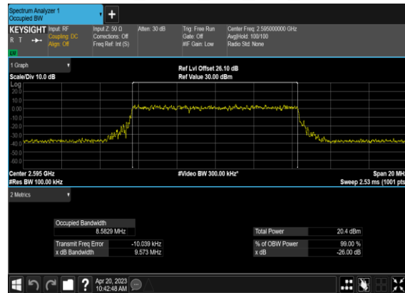
N38(10M)_CP-OFDM_256 QAM_Outer_Full_Mid_CH
