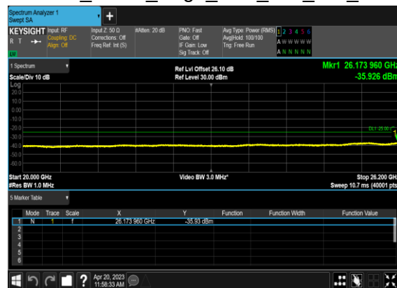
N38(10M)_DFT-s- OFDM_BPSK_Edge_1RB_Left_Mid_CH
