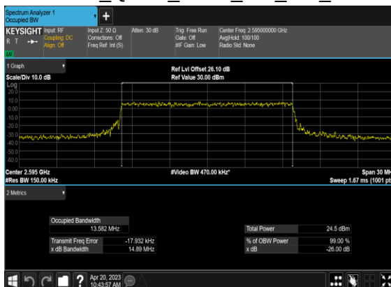
N38(15M)_CP- OFDM_QPSK_Outer_Full_Mid_CH
