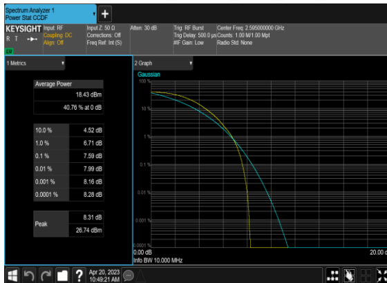
N38(15M)_DFT-s-OFDM_QPSK_Outer_Full_Mid_CH
