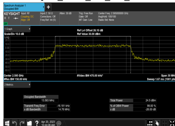
N38(15M)_CP-OFDM_16 QAM_Outer_Full_Mid_CH
