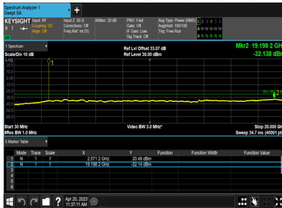
N38(10M)_DFT-s- OFDM_QPSK_Edge_1RB_Left_Low_CH
