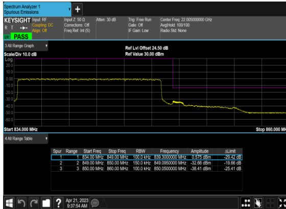
N26(15M)_DFT-s- OFDM_BPSK_Outer_Full_High_CH
