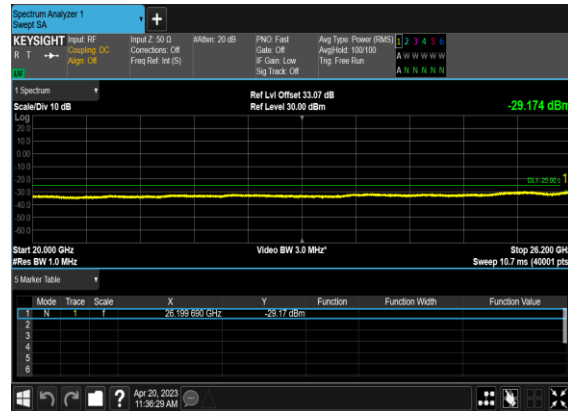
N38(10M)_DFT-s- OFDM_BPSK_Edge_1RB_Left_Low_CH
