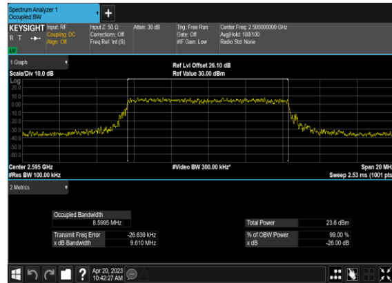
N38(10M)_CP-OFDM_16 QAM_Outer_Full_Mid_CH
