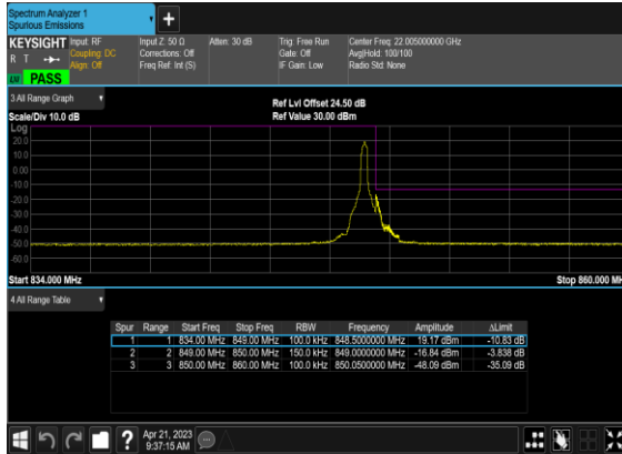
N26(15M)_DFT-s- OFDM_BPSK_Edge_1RB_Right_High_CH
