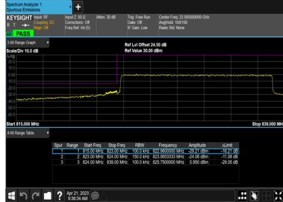
N26(15M)_DFT-s- OFDM_QPSK_Outer_Full_Low_CH
