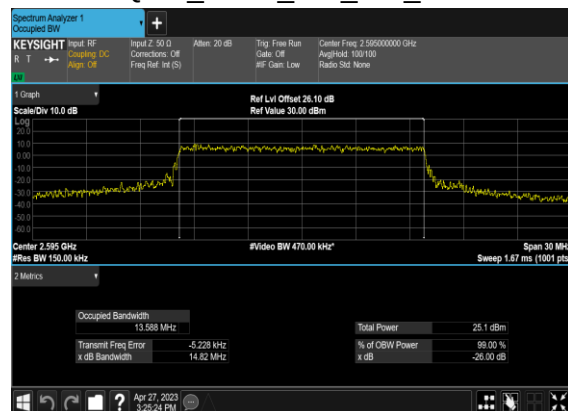
B66_N38(15M)_CP-OFDM_16 QAM_Outer_Full_Mid_CH
