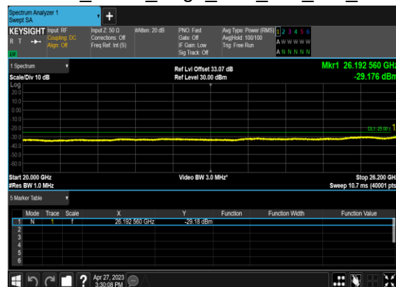
B66_N38(15M)_DFT-s-OFDM_BPSK_Edge_1RB_Left_Mid_CH
