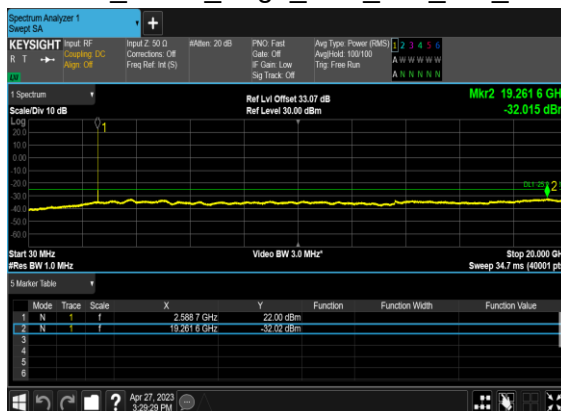
B66_N38(15M)_DFT-s-OFDM_BPSK_Edge_1RB_Left_Mid_CH
