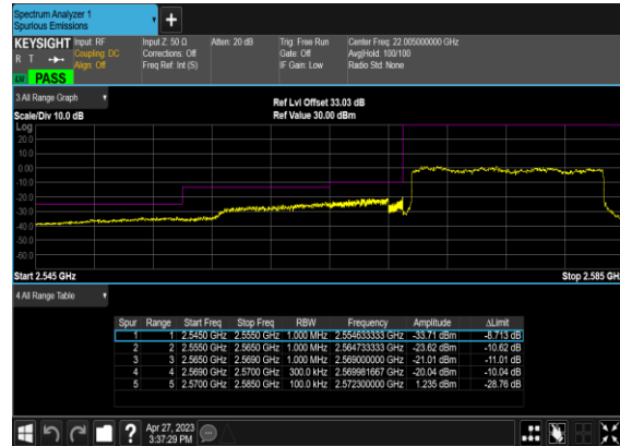
B66_N38(15M)_DFT-s- OFDM_QPSK_Outer_Full_Low_CH
