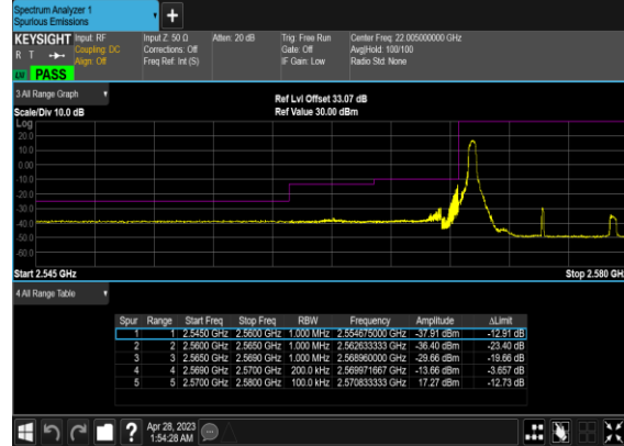
B66_N38(10M)_DFT-s- OFDM_QPSK_Edge_1RB_Left_Low_CH
