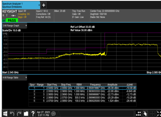
B66_N38(15M)_DFT-s- OFDM_BPSK_Outer_Full_Low_CH
