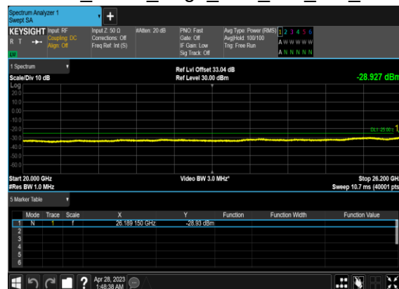
B66_N38(10M)_DFT-s-OFDM_BPSK_Edge_1RB_Left_Mid_CH
