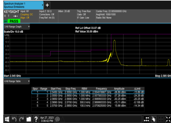
B66_N38(15M)_DFT-s- OFDM_QPSK_Edge_1RB_Left_Low_CH
