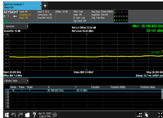
B66_N38(15M)_DFT-s-OFDM_QPSK_Edge_1RB_Left_Low_CH
