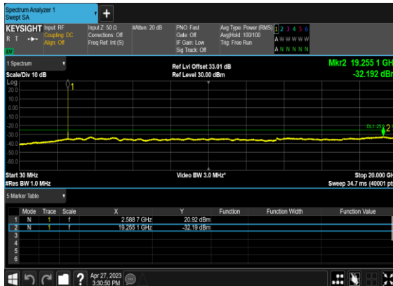
B66_N38(15M)_DFT-s-OFDM_QPSK_Edge_1RB_Left_Mid_CH
