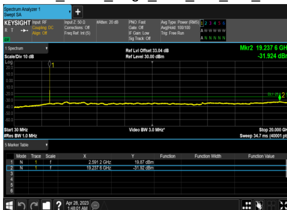
B66_N38(10M)_DFT-s-OFDM_BPSK_Edge_1RB_Left_Mid_CH
