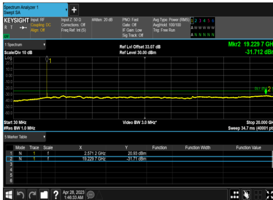
B66_N38(10M)_DFT-s-OFDM_QPSK_Edge_1RB_Left_Low_CH
