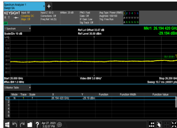
B66_N38(15M)_DFT-s-OFDM_BPSK_Edge_1RB_Left_High_CH
