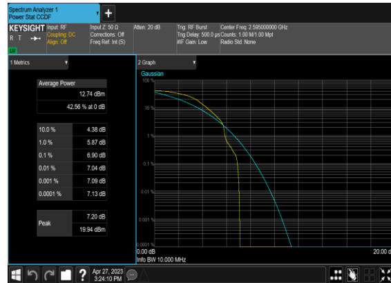
B66_N38(15M)_DFT-s-OFDM_PI_2-BPSK_Edge_1RB_Left_Mid_CH
