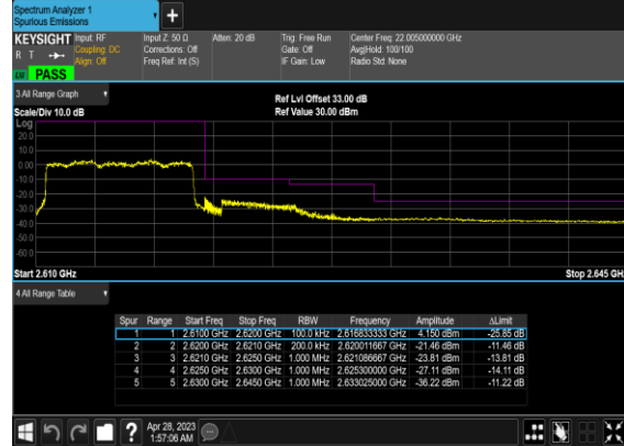
B66_N38(10M)_DFT-s- OFDM_QPSK_Outer_Full_High_CH
