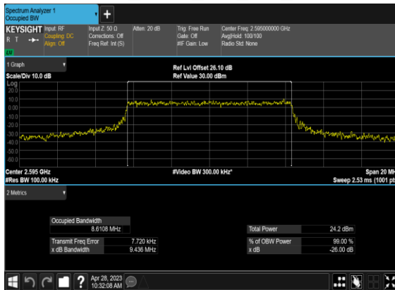
B66_N38(10M)_CP-OFDM_64 QAM_Outer_Full_Mid_CH
