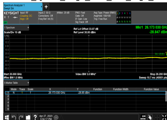
B66_N38(15M)_DFT-s-OFDM_QPSK_Edge_1RB_Left_High_CH
