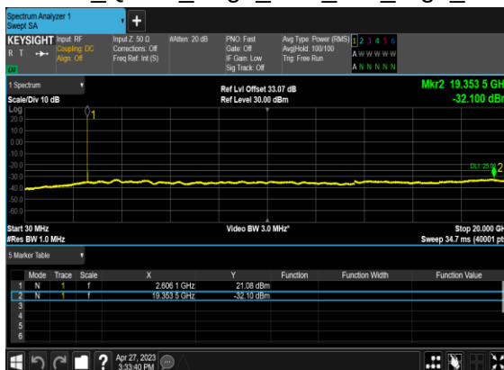
B66_N38(15M)_DFT-s-OFDM_QPSK_Edge_1RB_Left_High_CH
