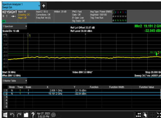
B66_N38(15M)_DFT-s-OFDM_BPSK_Edge_1RB_Left_High_CH
