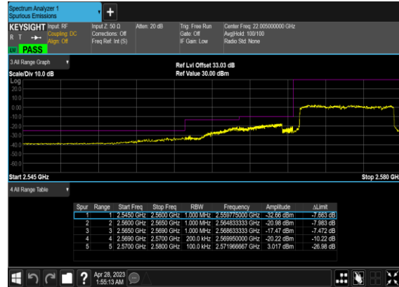
B66_N38(10M)_DFT-s- OFDM_QPSK_Outer_Full_Low_CH
