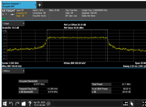
B66_N38(10M)_CP- OFDM_QPSK_Outer_Full_Mid_CH
