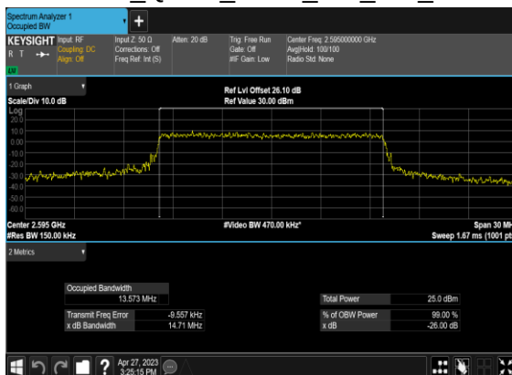
B66_N38(15M)_CP- OFDM_QPSK_Outer_Full_Mid_CH
