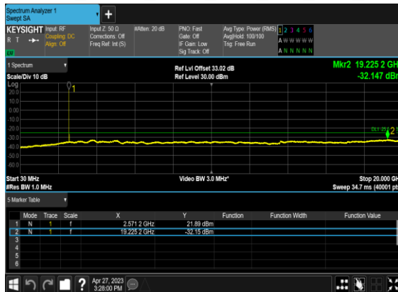
B66_N38(15M)_DFT-s-OFDM_QPSK_Edge_1RB_Left_Low_CH
