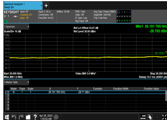
B66_N38(10M)_DFT-s-OFDM_BPSK_Edge_1RB_Left_Low_CH
