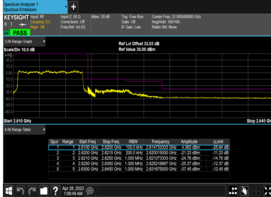
B66_N38(10M)_DFT-s- OFDM_BPSK_Outer_Full_High_CH
