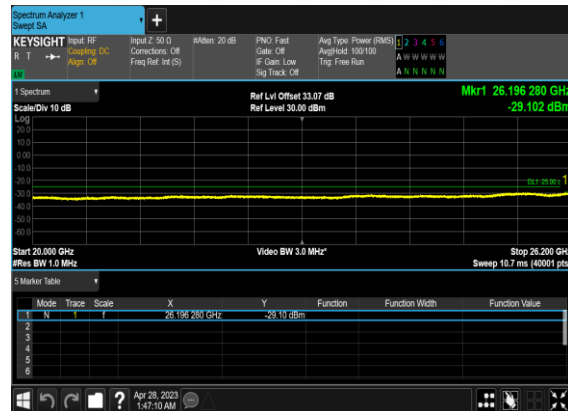
B66_N38(10M)_DFT-s-OFDM_QPSK_Edge_1RB_Left_Low_CH
