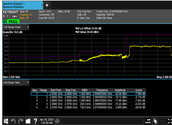
B66_N38(10M)_DFT-s- OFDM_BPSK_Outer_Full_Low_CH
