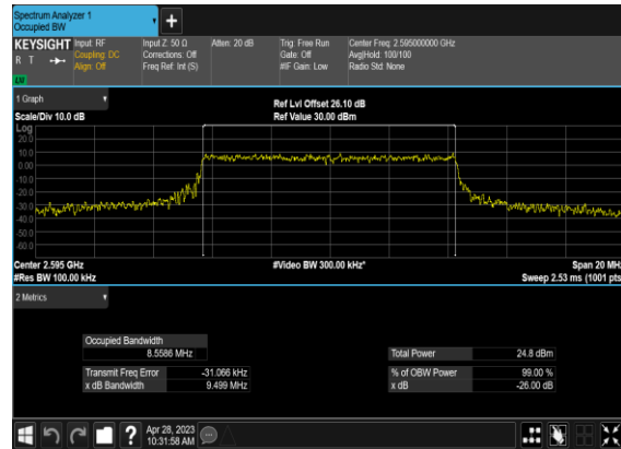
B66_N38(10M)_CP-OFDM_16 QAM_Outer_Full_Mid_CH
