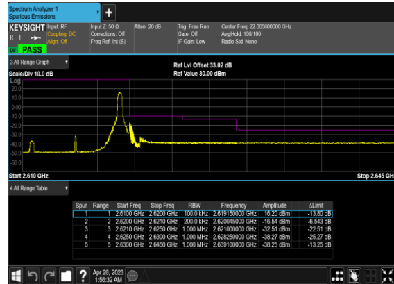
B66_N38(10M)_DFT-s- OFDM_QPSK_Edge_1RB_Right_High_CH
