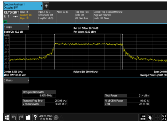
B66_N38(10M)_CP-OFDM_256 QAM_Outer_Full_Mid_CH
