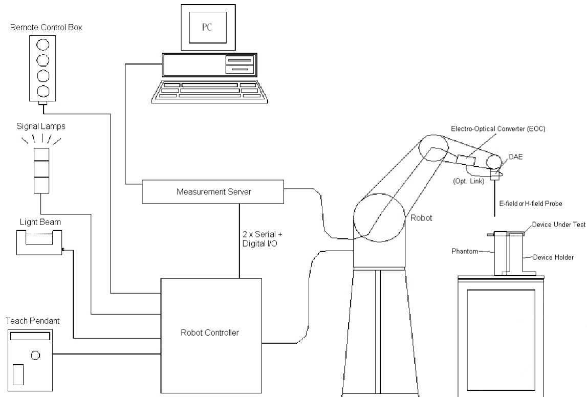
Fig 6.1 System Configurations
