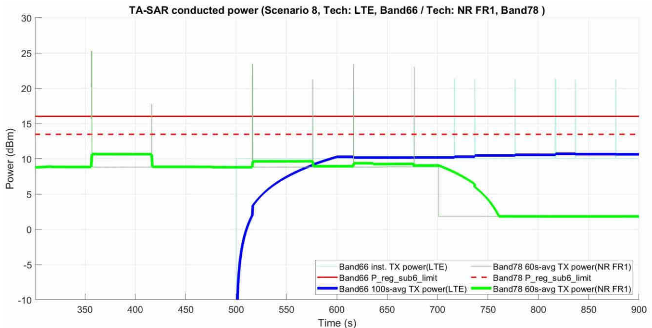
Figure 5- 46 Time-averaged conducted TX power over time
