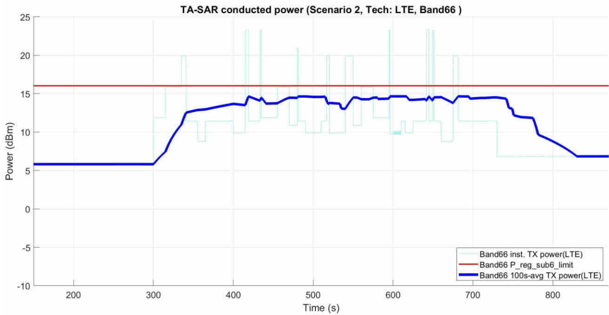
Figure 5- 20 Time-averaged conducted TX power over time
