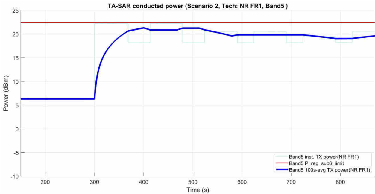
Figure 5- 29 Time-averaged conducted TX power over time
