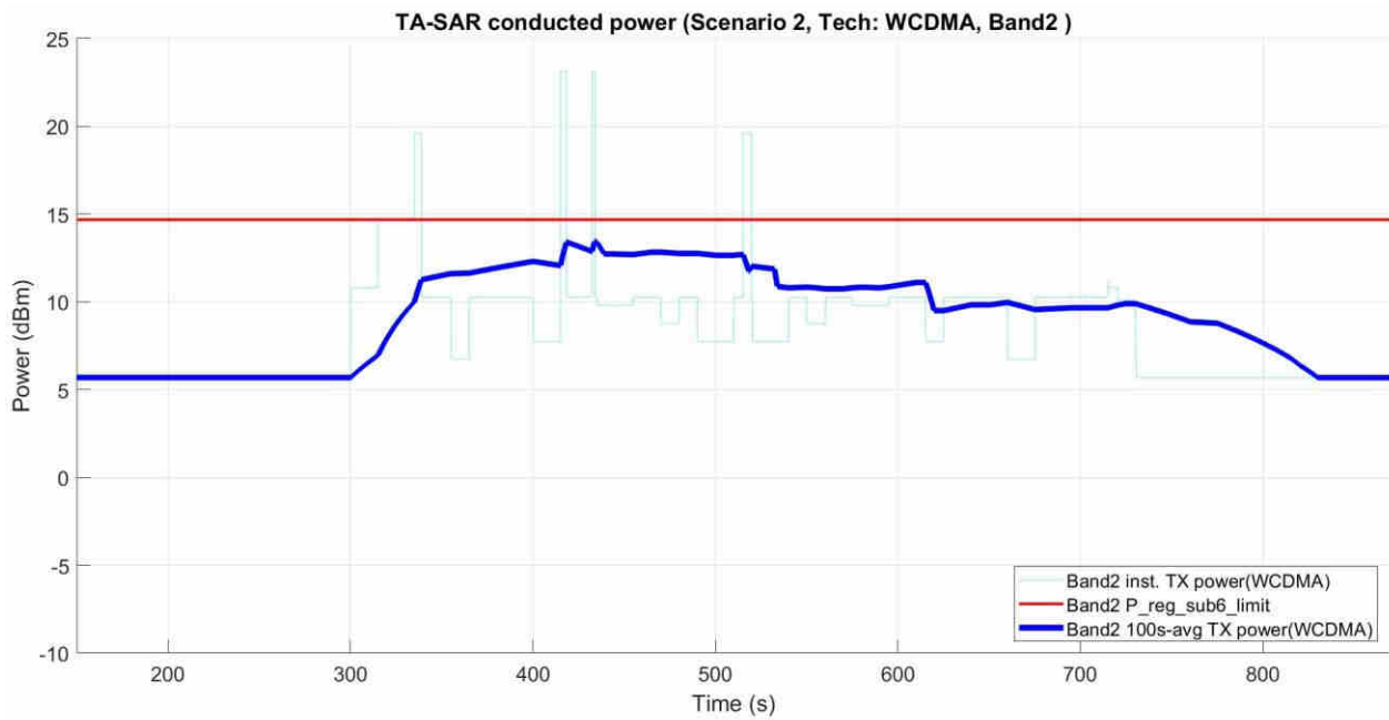
Figure 5- 28 Time-averaged conducted TX power over time
