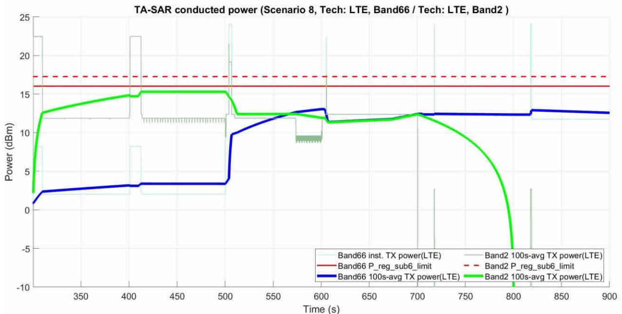
Figure 5- 48 Time-averaged conducted TX power over time
