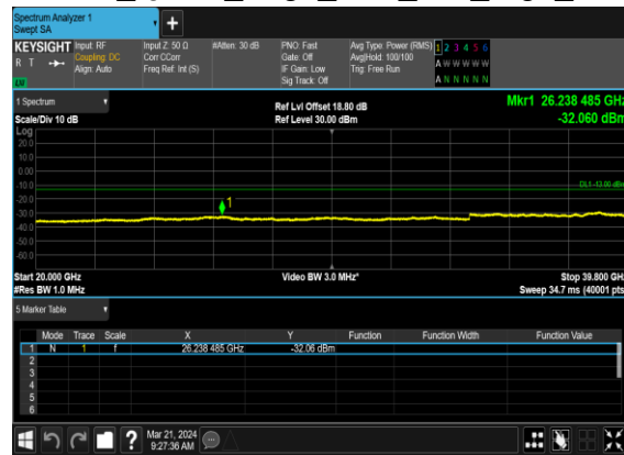
N77(50M)_DFT-s- OFDM_QPSK_Edge_1RB_Left_High_CH
