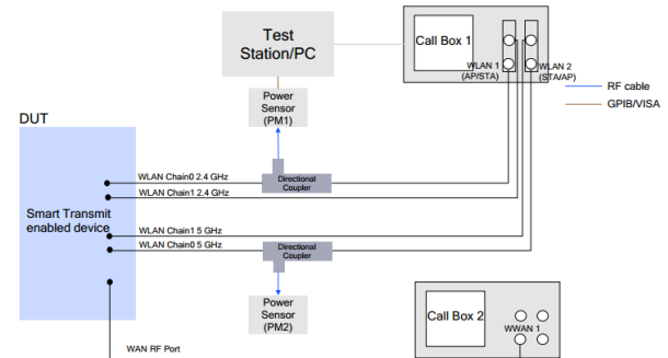
WLAN DBS Test setup - MIMO
