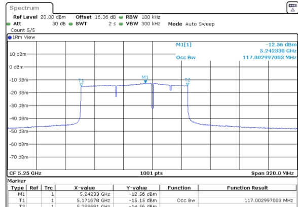
11BE160MIMO_5250_Puncturing 40M_4
