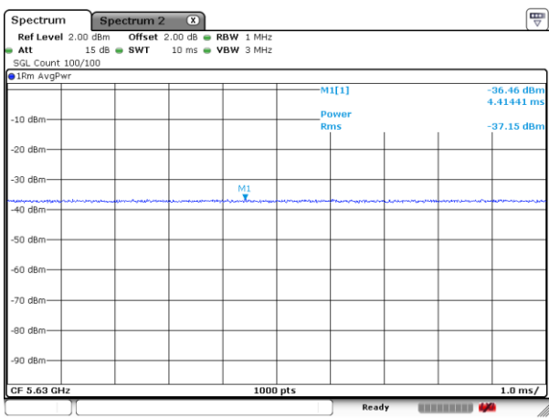
11BE160MIMO_5570_Puncturing 40M_4
