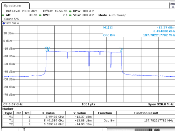
11BE160MIMO_5570_Puncturing 20M_8
