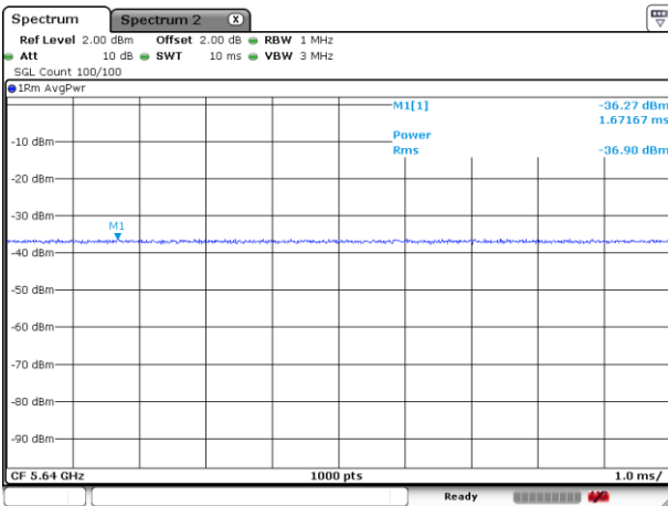
11BE160MIMO_5570_Puncturing 20M_8
