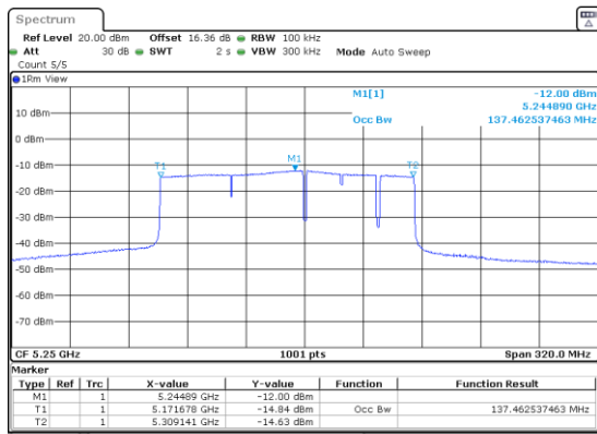
11BE160MIMO_5250_Puncturing 20M_8
