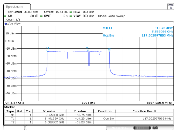
11BE160MIMO_5570_Puncturing 40M_4
