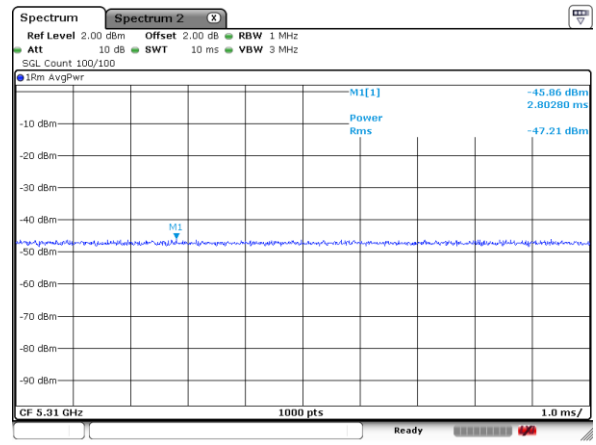
11BE160MIMO_5250_Puncturing 40M_4
