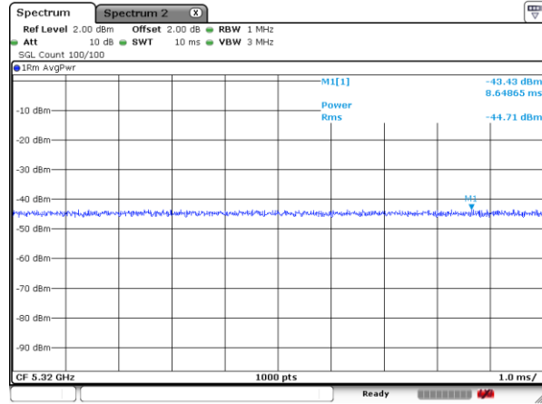
11BE160MIMO_5250_Puncturing 20M_8
