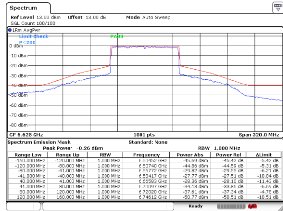
Plot on Channel 6625MHz
