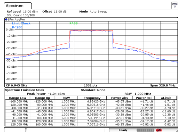
Plot on Channel 6945MHz
