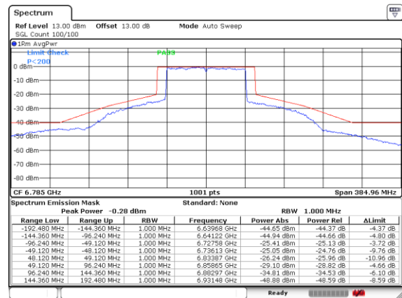
Plot on Channel 6785MHz
