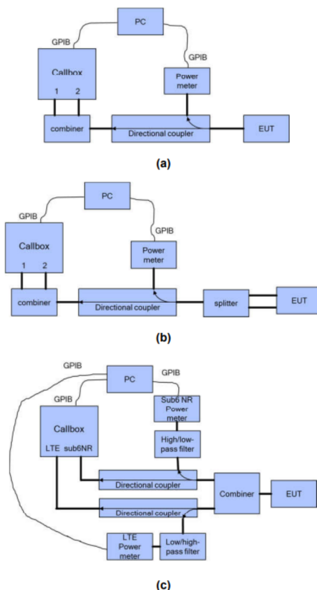
Figure 5-1 Conducted power measurement setup
