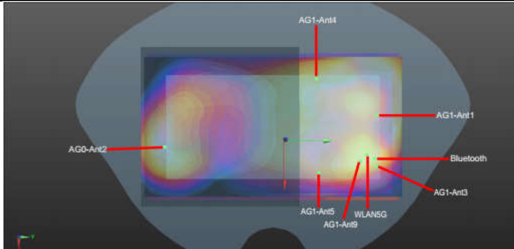
Hotspot_Front 5mm
