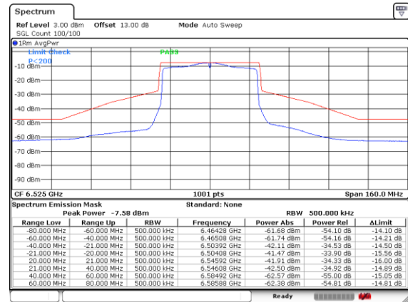
Plot on Channel 6525MHz
