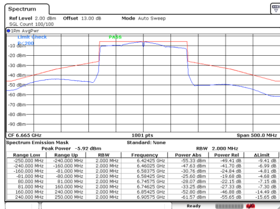
Plot on Channel 6665MHz
