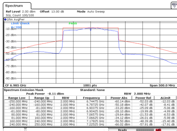
Plot on Channel 6985MHz
