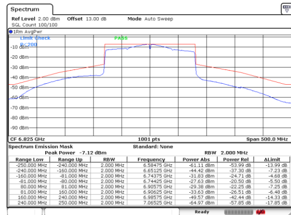
Plot on Channel 6825MHz
