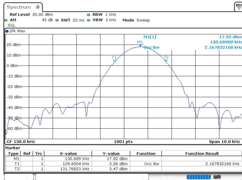
99% Occupied Bandwidth Plot
