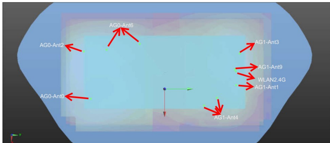
Body_Back 5mm
