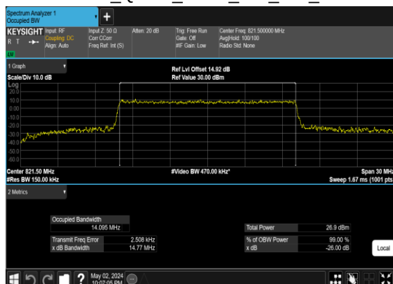
N26(15M)_CP- OFDM_QPSK_Outer_Full_Mid_CH
