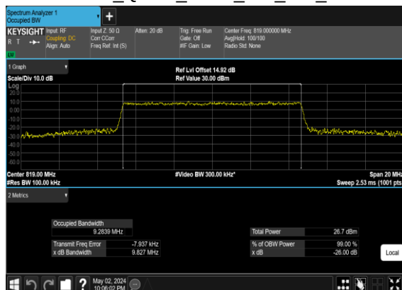
N26(10M)_CP- OFDM_QPSK_Outer_Full_Mid_CH
