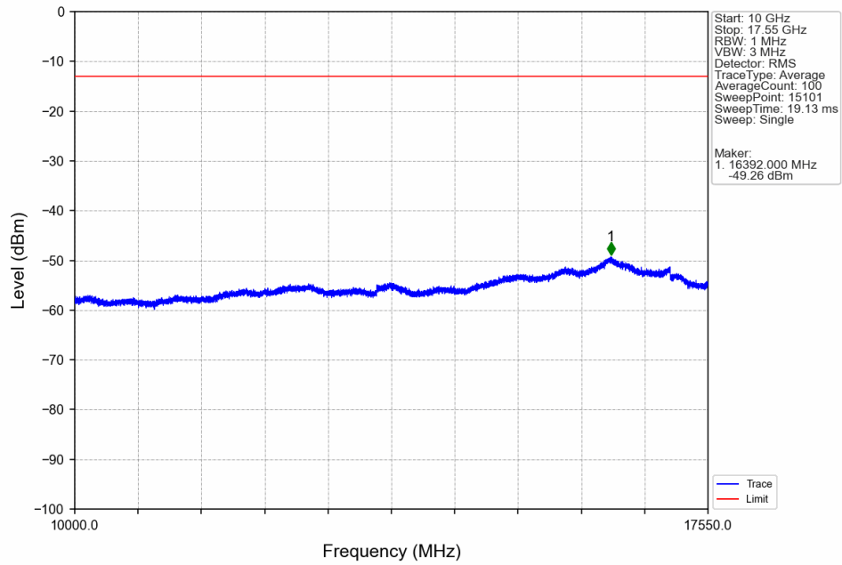
BandIV_RMC_MCH_1732.6MHz_12.2kbps RMC_NTNV
