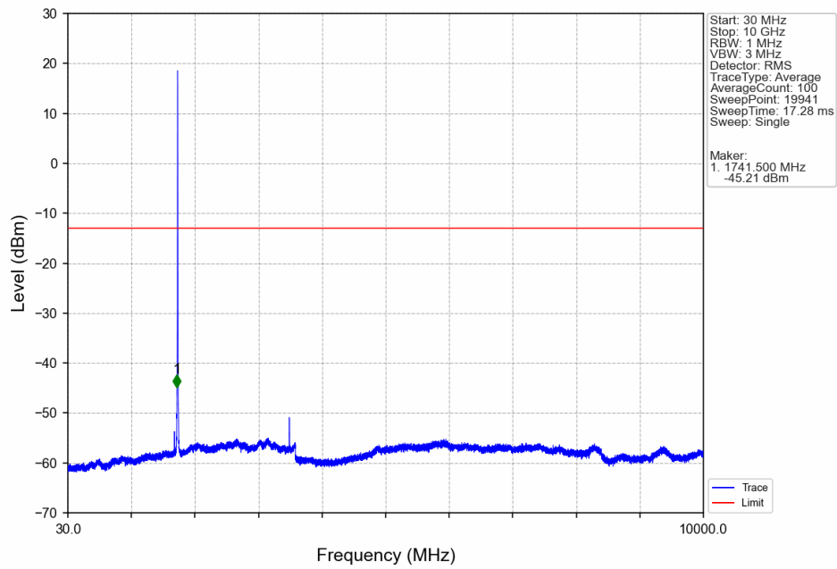
BandIV_RMC_HCH_1752.6MHz_12.2kbps RMC_NTNV
