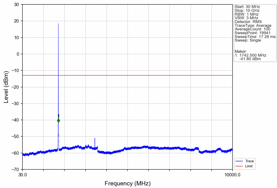
BandIV_RMC_MCH_1732.6MHz_12.2kbps RMC_NTNV
