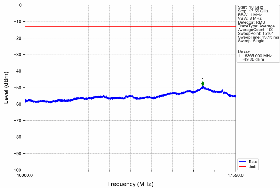
BandIV_RMC_HCH_1752.6MHz_12.2kbps RMC_NTNV
