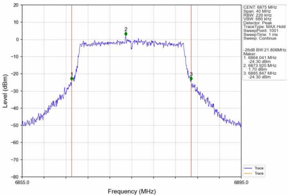
802.11ax(HEW20)_HCH_6875MHz_SU_ / Ant4_NTNV
