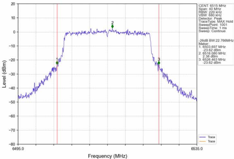
802.11ax(HEW20)_HCH_6515MHz_SU_ / Ant4_NTNV
