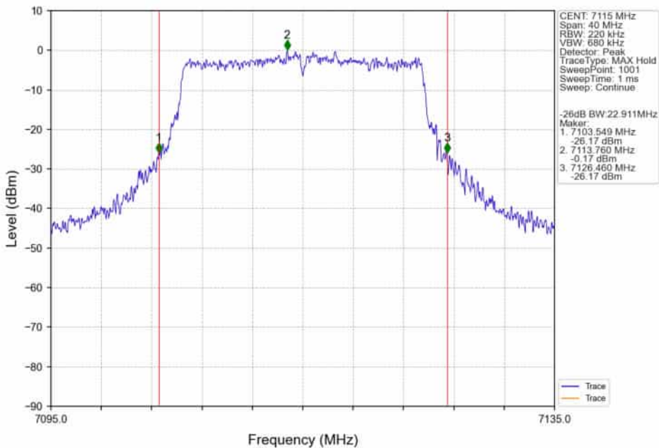
802.11ax(HEW20)_HCH_7115MHz_SU_ / Ant4_NTNV
