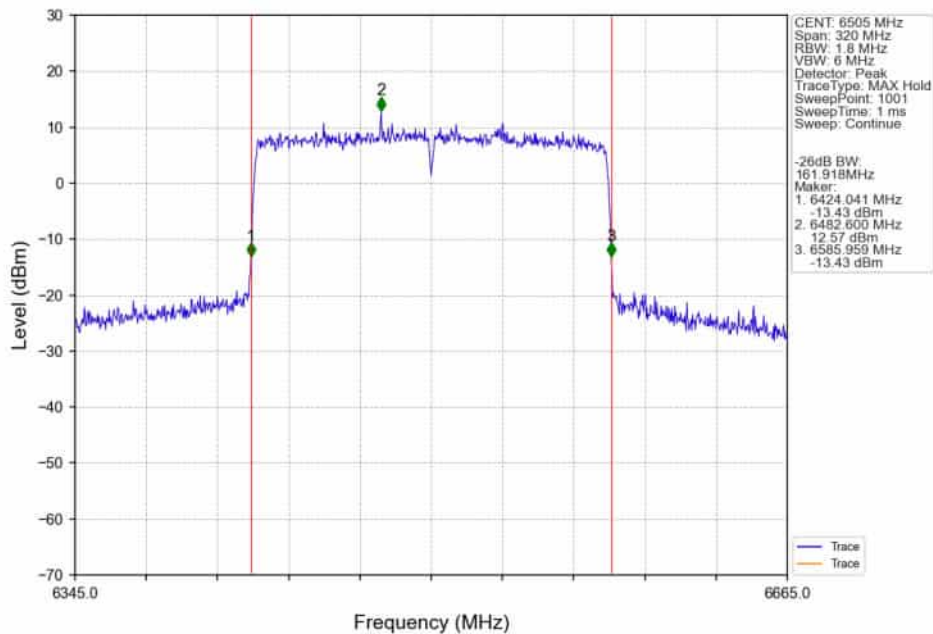
802.11ax(HEW160)_HCH_6505MHz_SU / _Ant4_NTNV
