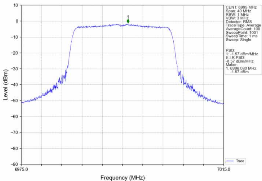
802.11ax(HEW20)_MCH_6995MHz_SU_/_Ant4_NTNV
