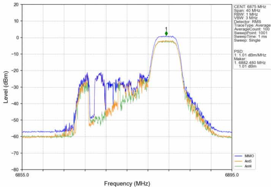
802.11ax(HEW20)_HCH_6875MHz_RU106_/_Ant5_NTNV
