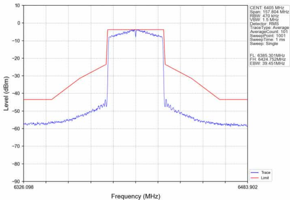
802.11ax(HEW40)_HCH_6405MHz_SU_/_Ant4_NTNV
