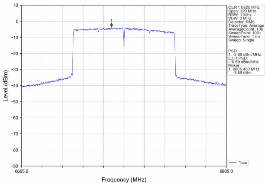
802.11ax(HEW160)_HCH_6825MHz_SU_/_Ant5_NTNV
