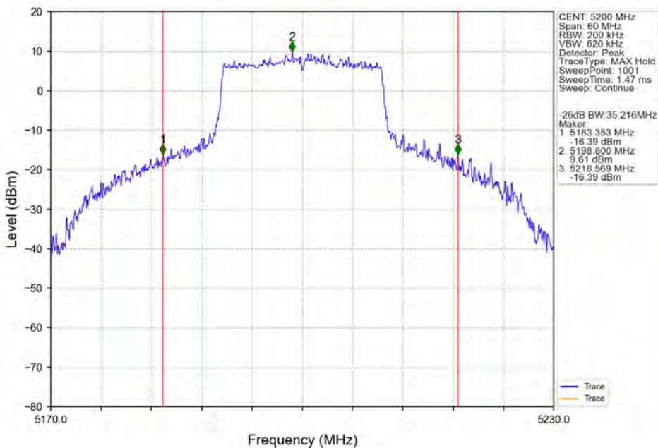
802.11ax(HEW20)_MCH_5200MHz_SU_ / Ant4_NTNV
