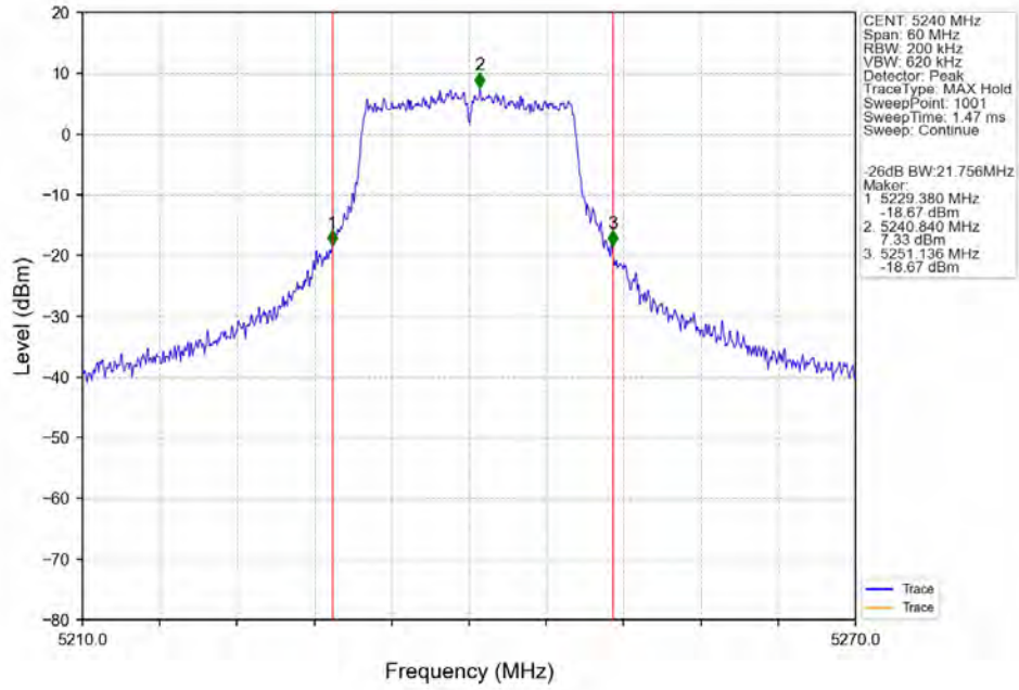
802.11a_HCH_5240MHz_Ant4_NTNV
