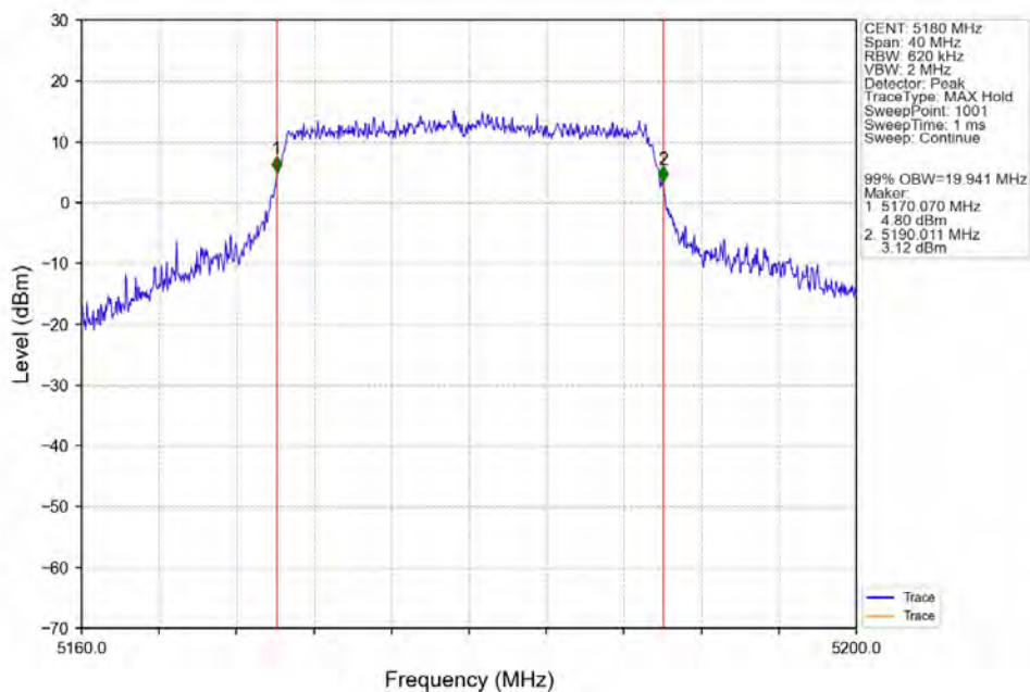
802.11ax(HEW20)_LCH_5180MHz_SU_ / Ant4_NTNV
