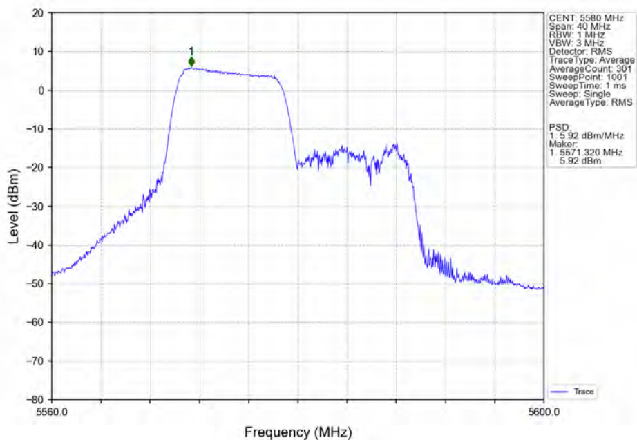
802.11ax(HEW20)_MCH_5580MHz_RU106 / _Ant4_NTNV
