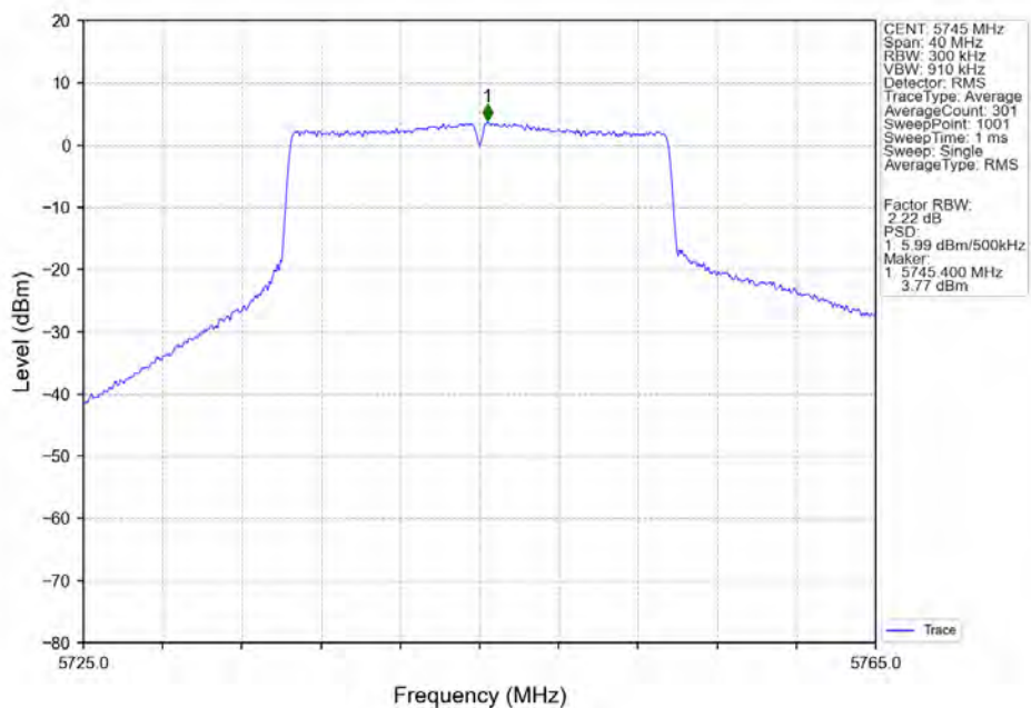
802.11ax(HEW20)_LCH_5745MHz_SU_/_Ant5_NTNV
