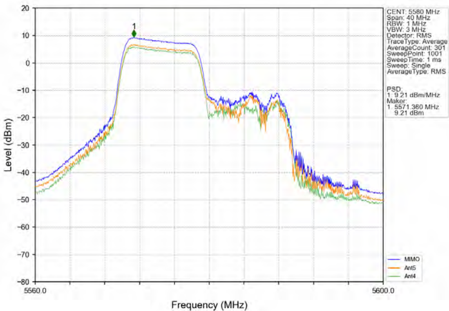
802.11ax(HEW20)_MCH_5580MHz_SU_ / Ant5_NTNV
