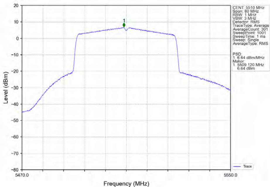
802.11ax(HEW40)_LCH_5510MHz_SU_/_Ant4_NTNV
