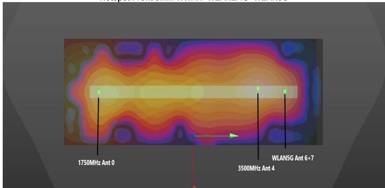
Hotspot Left Side 5mm WWAN+WLAN5G
