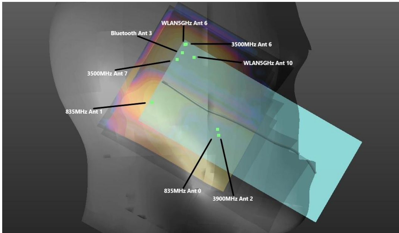
Head Left Cheek WWAN+WLAN5G+BT 0mm
