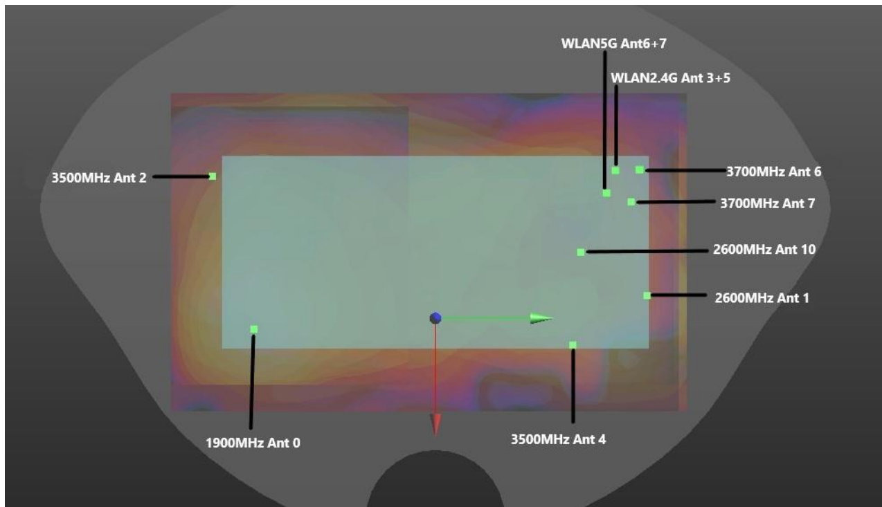
Body worn (n-1) Back 18mm WWAN+WLAN2.4G+WLAN5G
