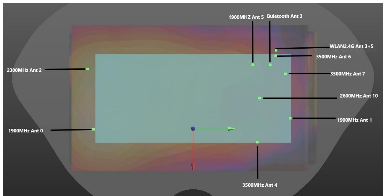
Body-worn Back 5mm WWAN+WLAN2.4G+BT
