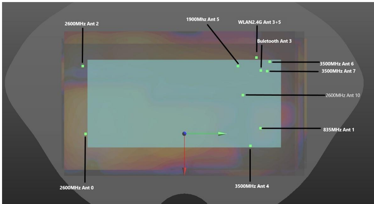
Hotspot Back 5mm WWAN+WLAN2.4G+BT
