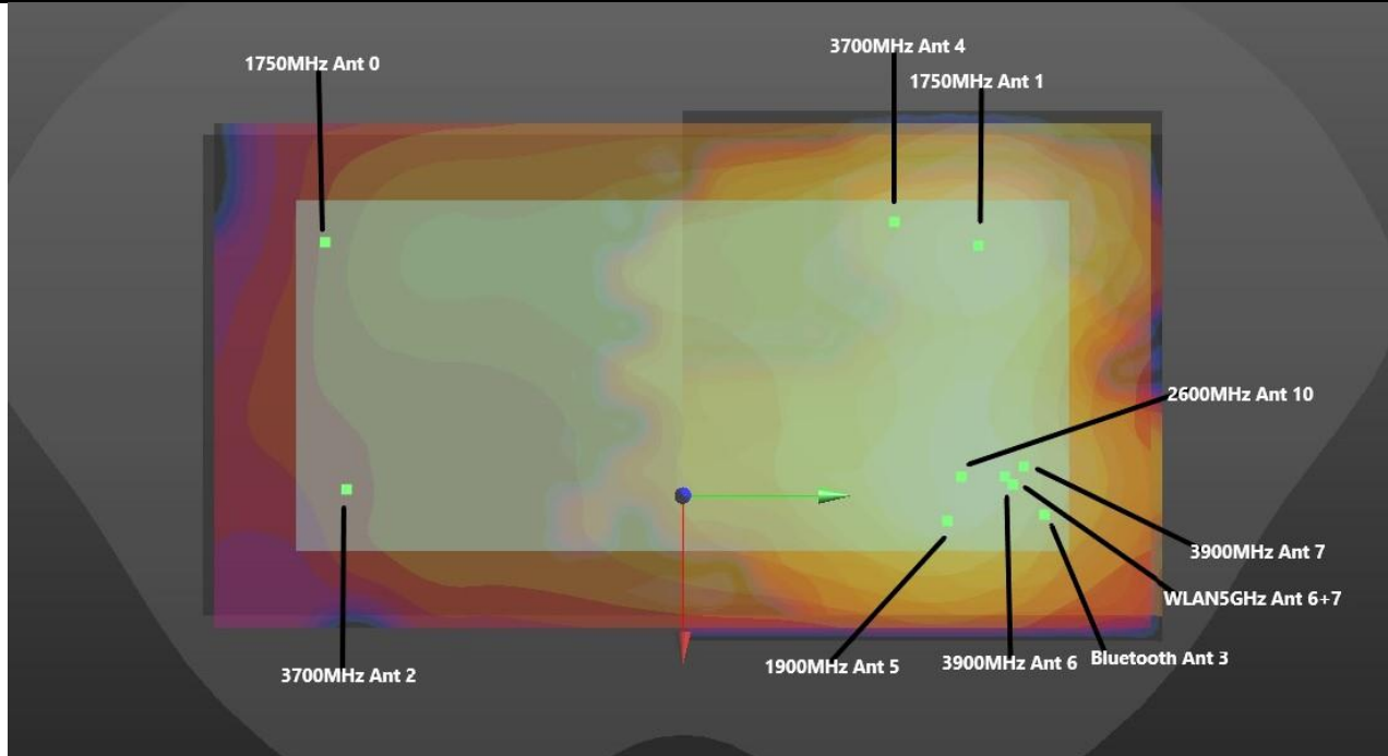
Body-worn Front 5mm WWAN+WLAN5G+BT
