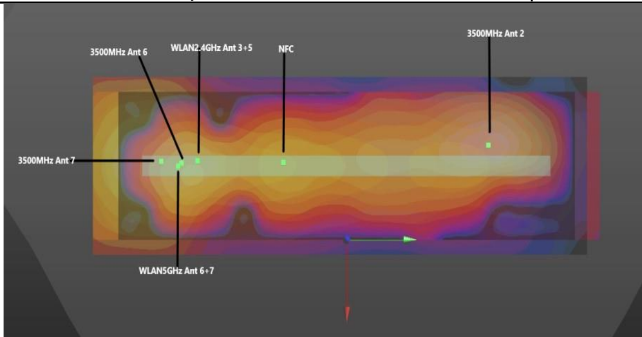
Extremity Right Side 0mm WWAN+WLAN5G+WLAN2.4G+NFC
