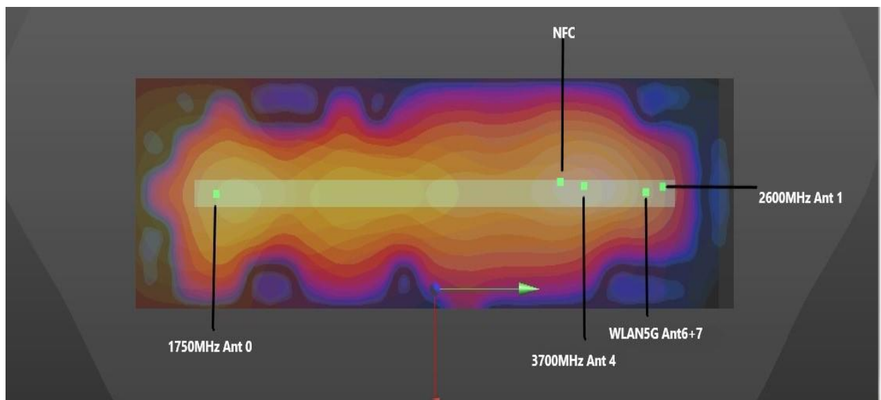
Extremity Left Side 0mm WWAN+WLAN5G+NFC
