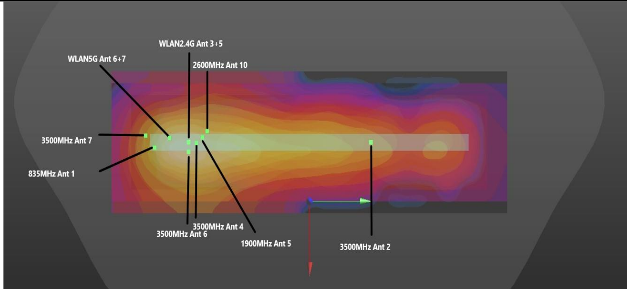
Hotspot Right Side 5mm WWAN+WLAN5G+WLAN2.4G
