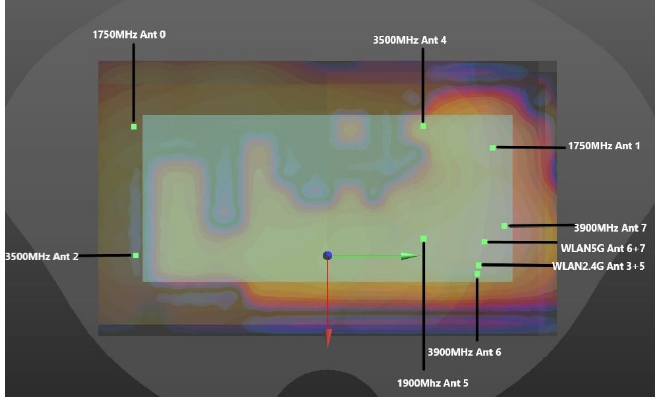
Hotspot Front 5mm WWAN+WLAN2.4G+WLAN5G
