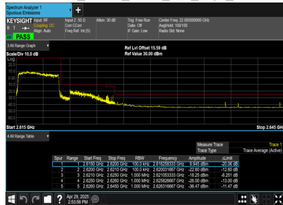
N38(5M)_DFT-s- OFDM_QPSK_Outer_Full_High_CH
