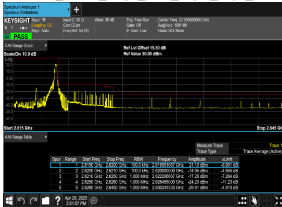
N38(5M)_DFT-s- OFDM_BPSK_Edge_1RB_Right_High_CH
