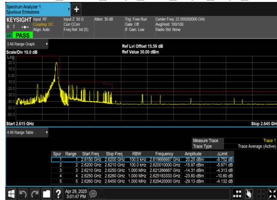
N38(5M)_DFT-s- OFDM_QPSK_Edge_1RB_Right_High_CH
