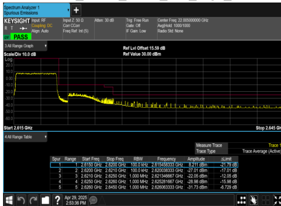
N38(5M)_DFT-s- OFDM_BPSK_Outer_Full_High_CH
