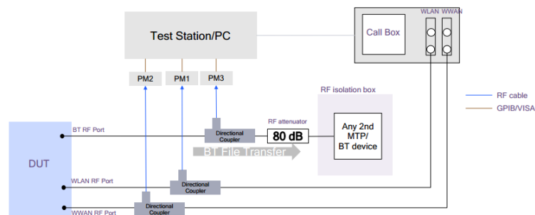
Figure 5-3 System Level Continuity test setup
