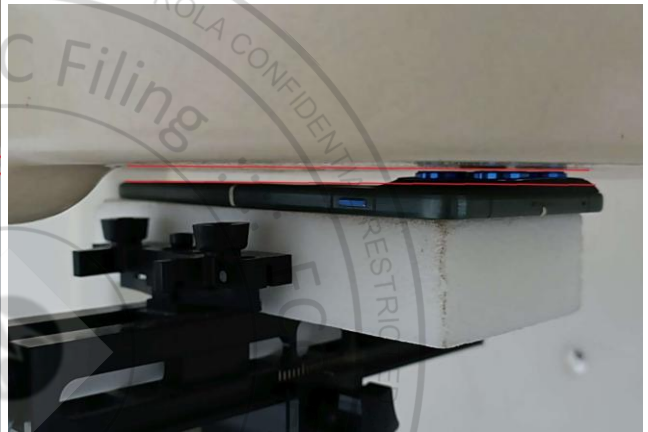
Back, Test Separation 6 mm
