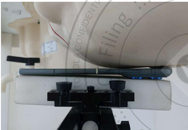
Left Cheek, Test Separation 0mm
