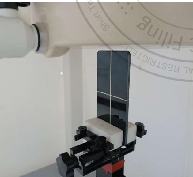
Top Side, Test Separation 6 mm
