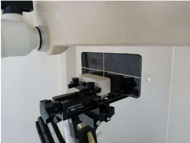
Left Side, Test Separation 11 mm
