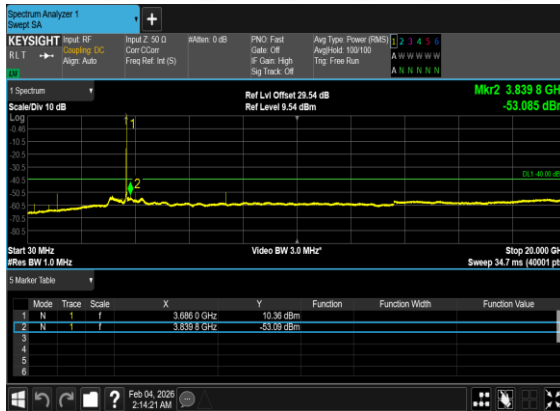
N48(15M)_DFT-s- OFDM_BPSK_Edge_1RB_Left_High_CH
