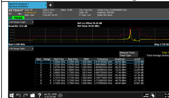
Conducted Band Edge Band 48 15MHz/3692.49/High BPSK 1@0
