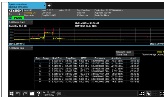
Conducted Band Edge Band 48 15MHz/3557.52/Low BPSK 36@0
