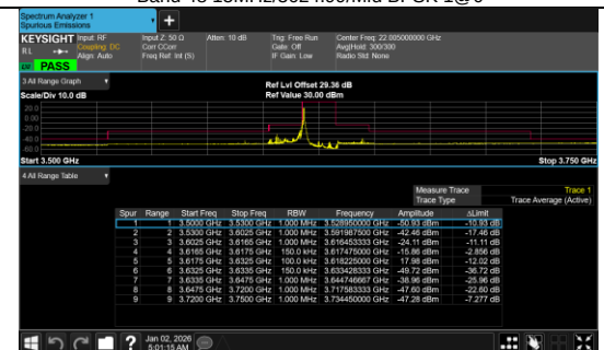
Conducted Band Edge Band 48 15MHz/3624.99/Mid QPSK 1@0
