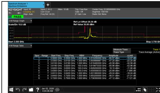
Conducted Band Edge Band 48 10MHz/3624.99/Mid BPSK 1@23
