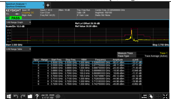
Conducted Band Edge Band 48 10MHz/3694.98/High QPSK 1@0
