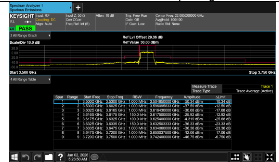
Conducted Band Edge Band 48 15MHz/3624.99/Mid QPSK 36@0
