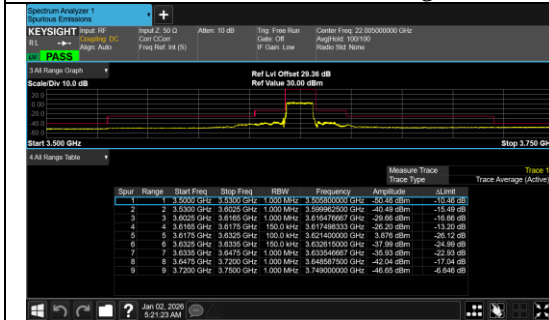
Conducted Band Edge Band 48 15MHz/3624.99/Mid BPSK 36@0
