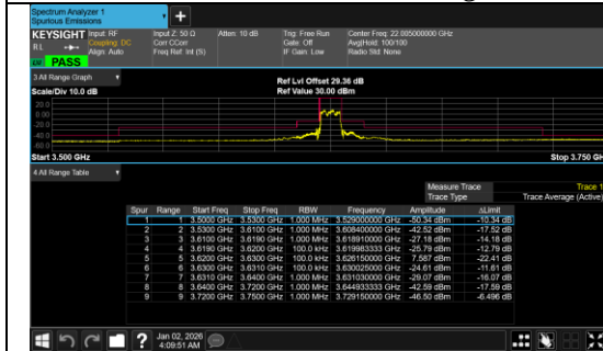
Conducted Band Edge Band 48 10MHz/3624.99/Mid BPSK 24@0
