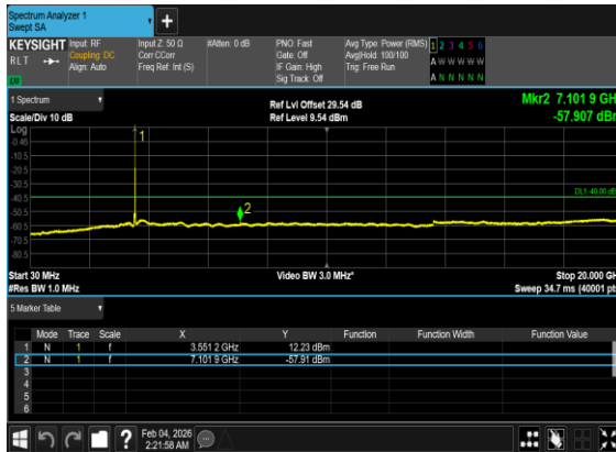
N48(30M)_DFT-s- OFDM_BPSK_Edge_1RB_Left_Low_CH
