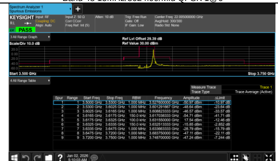
Conducted Band Edge Band 48 15MHz/3624.99/Mid BPSK 1@37
