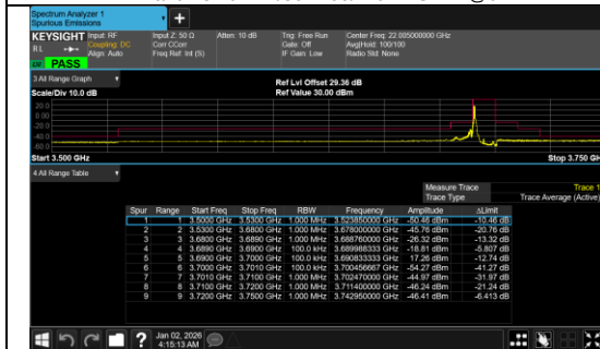
Conducted Band Edge Band 48 10MHz/3694.98/High BPSK 1@0
