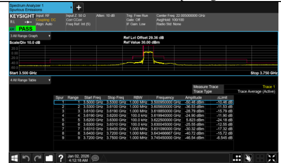
Conducted Band Edge Band 48 10MHz/3624.99/Mid QPSK 24@0
