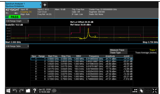
Conducted Band Edge Band 48 15MHz/3624.99/Mid QPSK 1@37
