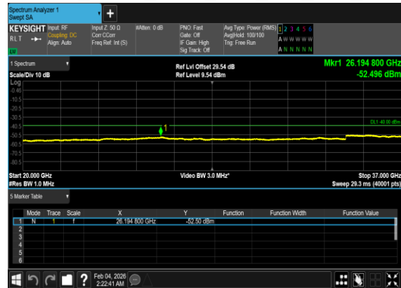
N48(30M)_DFT-s- OFDM_BPSK_Edge_1RB_Left_Low_CH
