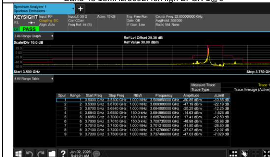
Conducted Band Edge Band 48 15MHz/3692.49/High QPSK 1@0
