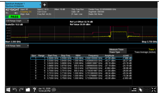
Conducted Band Edge Band 48 40MHz/3570.0/Low QPSK 1@0
