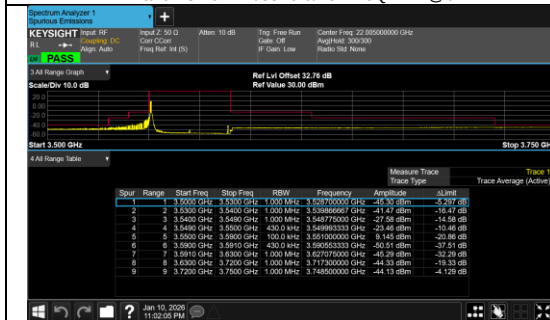
Conducted Band Edge Band 48 40MHz/3570.0/Low 16QAM 1@105
