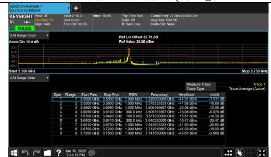
Conducted Band Edge Band 48 30MHz/3624.99/Mid QPSK 1@0
