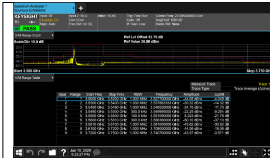
Conducted Band Edge Band 48 30MHz/3564.99/Low 16QAM 1@77
