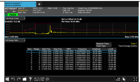
Conducted Band Edge Band 48 30MHz/3564.99/Low QPSK 75@0
