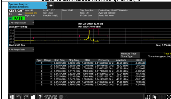
Conducted Band Edge Band 48 15MHz/3624.99/Mid 16QAM 1@0
