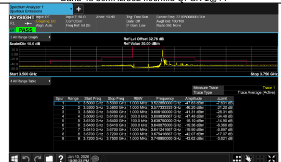
Conducted Band Edge Band 48 30MHz/3624.99/Mid QPSK 1@77
