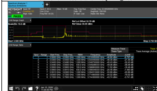
Conducted Band Edge Band 48 40MHz/3570.0/Low 16QAM 100@0
