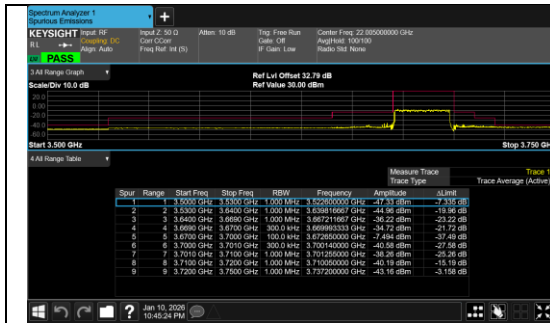
Conducted Band Edge CHP Range9 PASS Band 48 30MHz/3684.99/High 16QAM 75@0
