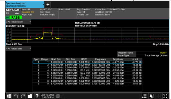
Conducted Band Edge CHP Range1 PASS Band 48 15MHz/3557.52/Low 16QAM 36@0
