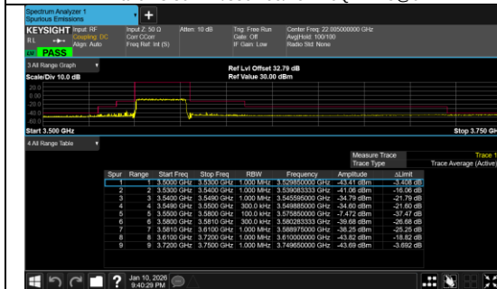
Conducted Band Edge Band 48 30MHz/3624.99/Mid 16QAM 1@0
