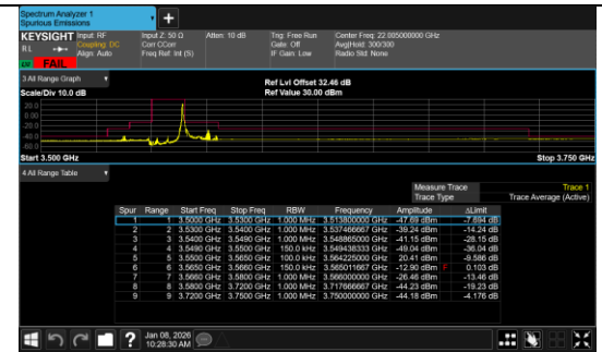
Conducted Band Edge Band 48 15MHz/3557.52/Low QPSK 36@0
